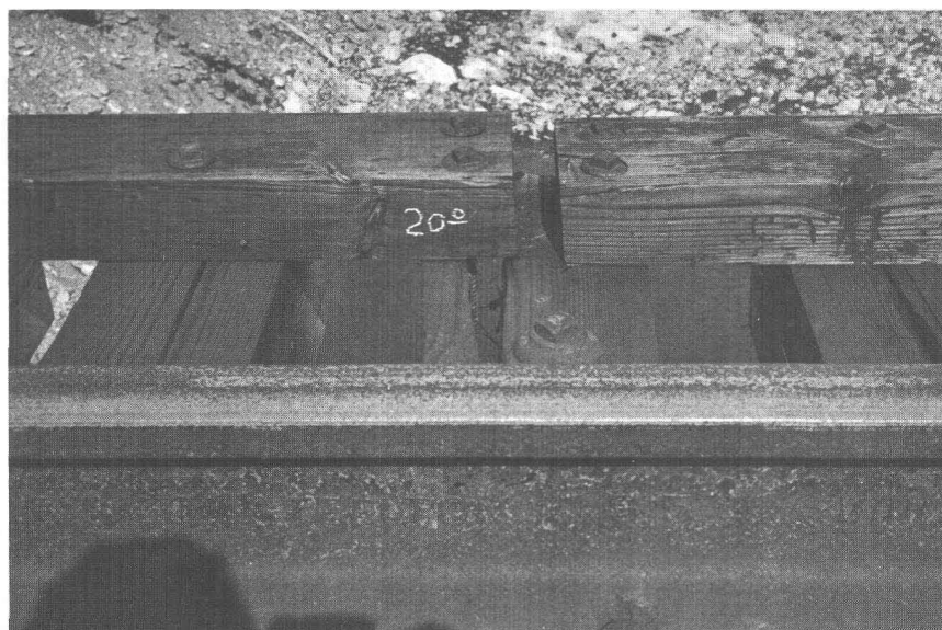
27.—Tension on Lakeview delta railroad bridge pulled guard timbers apart and split a tie.
