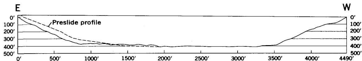
PROFILE ALONG FATHOMETER LINE 89
