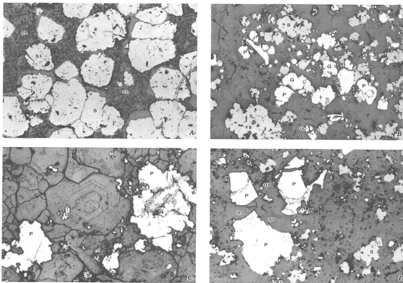
FIGURE 12.—Polished thin sections of sulfide minerals in Mississippian chert and metaquartzite of the Kagvik sequence in Drenchwater Creek area; numerous dark inclusions in sphalerite are polishing imperfections. Reflected plane-polarized light. S, sphalerite; G, galena; P, pyrite and marcasite; qv, quartz vein; ch, chert. A, Disseminated sphalerite in chert. Field of view is 1.8 mm long. B, Disseminated sphalerite, galena, pyrite, and marcasite in metaquartzite. Field of view is 0.9 mm long. C, Metaquartzite containing inclusions of sulfide minerals and hexagonal growth zones. Field of view is 1.8 mm long. D, Metaquartzite containing quartz vein and fractured pyrite and marcasite; quartz vein is between large pyrite and marcasite fragments. Field of view is 0.9 mm long.
