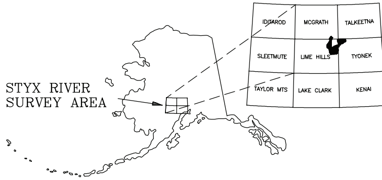
Section outlines from U.S. Geological Survey Lime Hills D-1, 1958; Tyonek D-7, 1973; D-8, 1958; Quadrangles, Alaska
