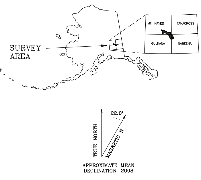
Section outlines from U.S. Geological Survey Gulkana D-1, 1978; Nabesna D-6, 1969; Quadrangles, Alaska
