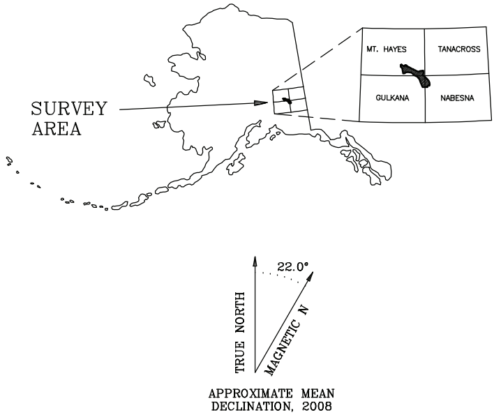
Section outlines from U.S. Geological Survey Gulkana D-1, 1978; Nabesna D-6, 1969; Quadrangles, Alaska
