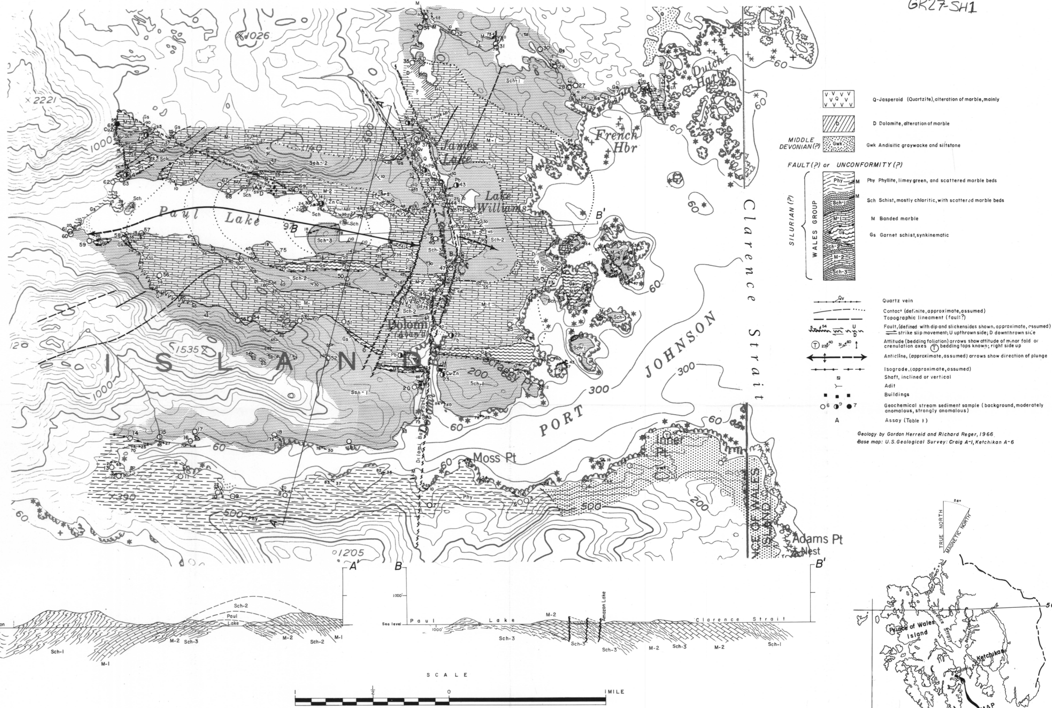
Figure 1. Geologic map and sections of the Dolomi area, Alaska
