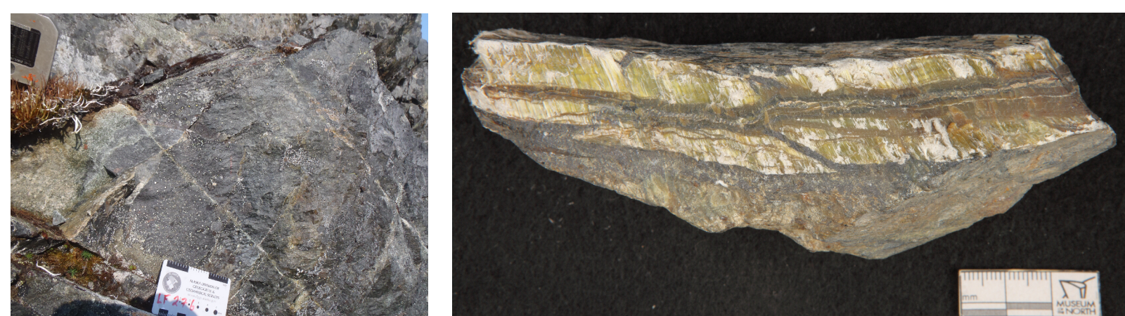
Five-grained Truesdell microgranitic rock, with orthopyroxene, clinopyroxene, and interstitial plagioclase. Ultramylonite rock is altered by epidote and pyroxene. Although this rock does not contain visible asbestos-forming minerals, it has the right chemistry to form them given the current metamorphic conditions. Photo collected during 2014 DGGS mapping in the Tulukina Mountains C-4 Quadrangle (photograph taken 07/21/2014 by L. K. Freeman). Chrysotile in serpentinite (UAMES 34964) collected from Comas Creek, Comas Hills area, Kobuk District, Alaska, by Edith Anderson. Occurrence likely corresponds to Alaska Resource Data File number ARD11. Image courtesy of the University of Alaska Museum Earth Sciences Department.
