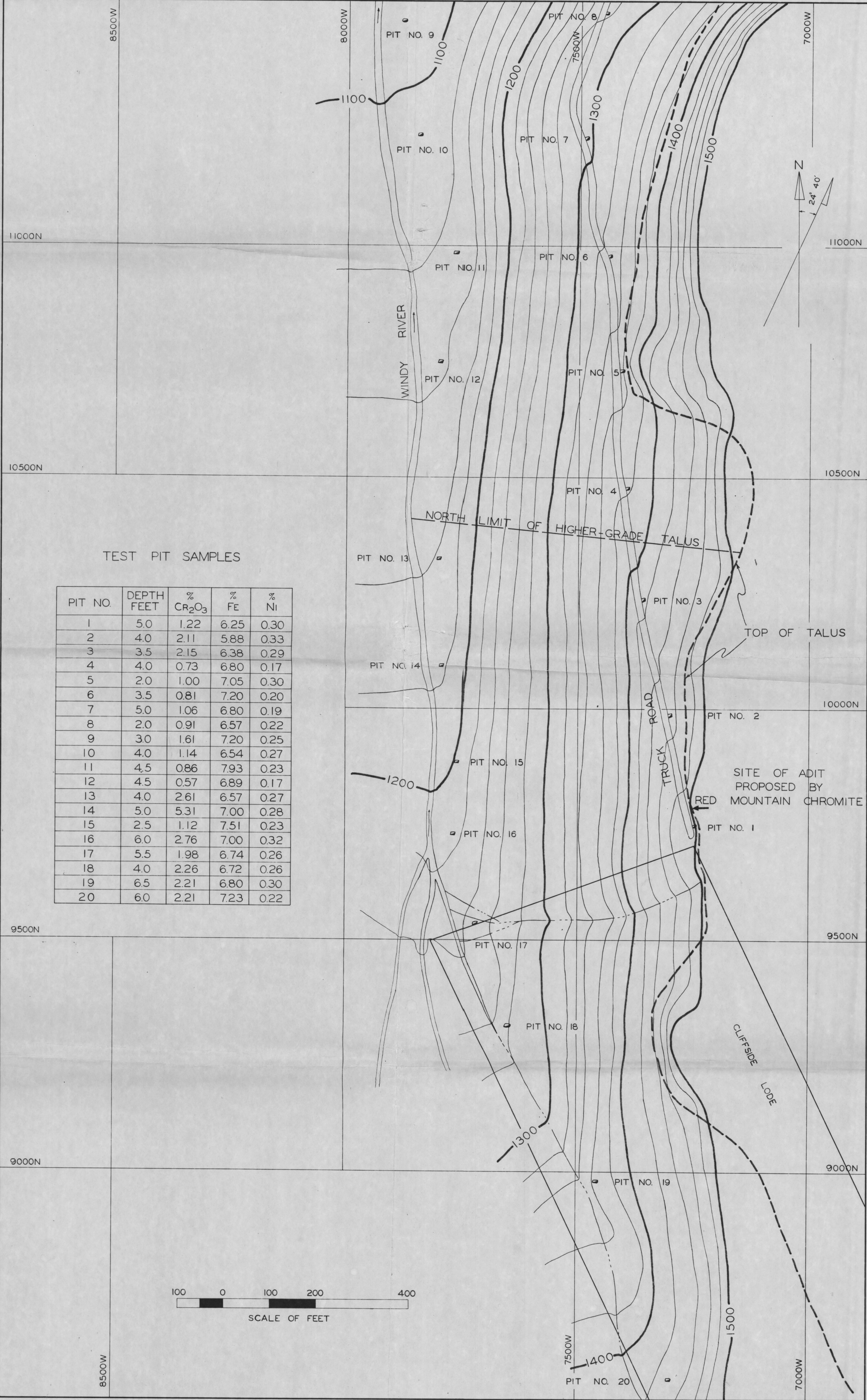
FIG. 27 SKETCH MAP SHOWING TEST PITS IN TALUS, RED MOUNTAIN, ALASKA
