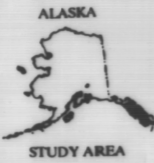
PLATE 1. GEOLOGY OF THE UPPER CLEARWATER CREEK AREA, MT. HAYES A-6 QUADRANGLE, ALASKA
