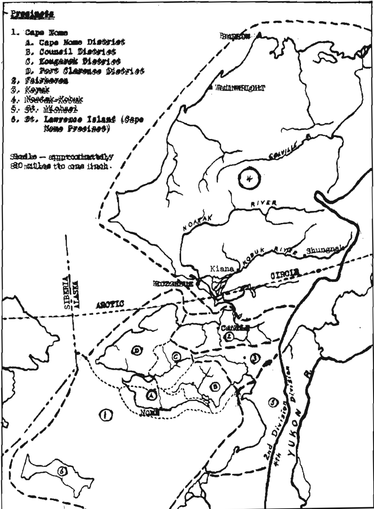
Fig. 1. Map of Northwestern Alaska showing mining precincts.
