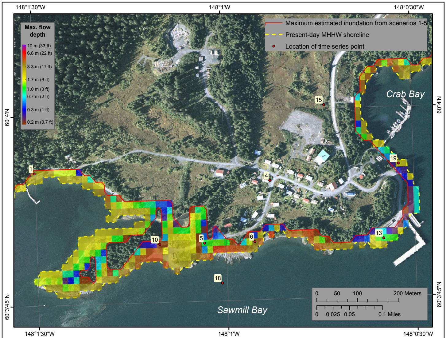
Maximum composite potential inundation computed for scenarios 1–5 near the community of Cheneaga Bay, and the maximum composite flow depths over dry land. The present-day MHHW shoreline is shown by a dashed yellow line.
