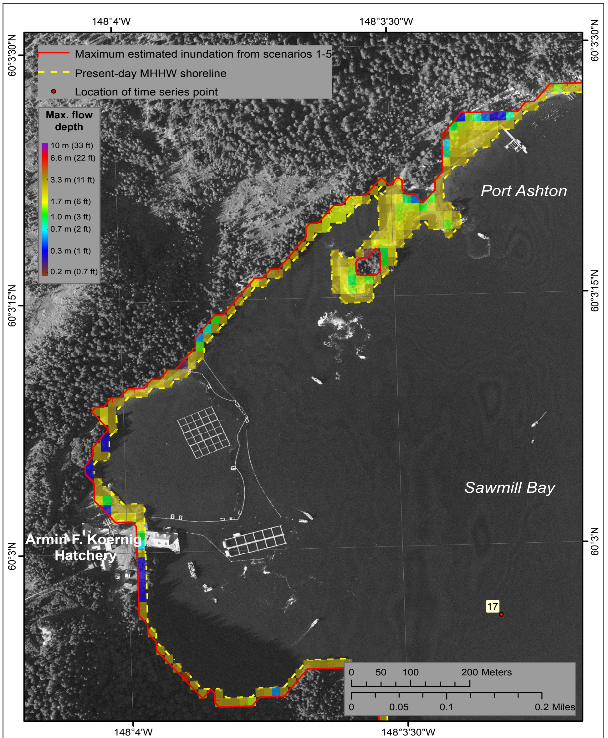
Maximum composite potential inundation for scenarios 1–5 in the western part of Sawmill Bay near the Armin F. Koernig hatchery, and the maximum composite flow depths over dry land.
