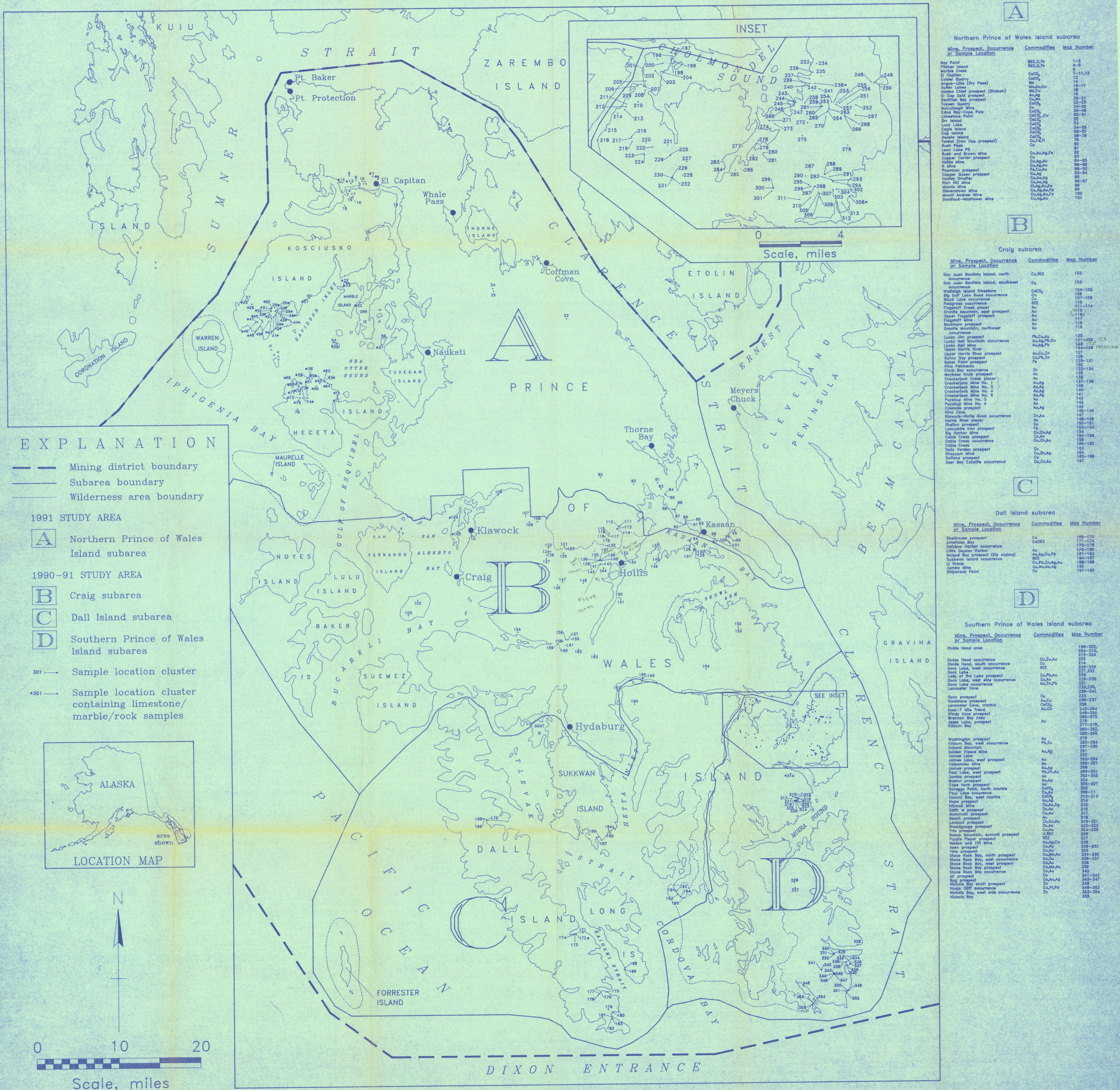
Figure 4. - Mines, prospects, occurrences, and sample locations from 1991 activities on Prince of Wales Island and vicinity
