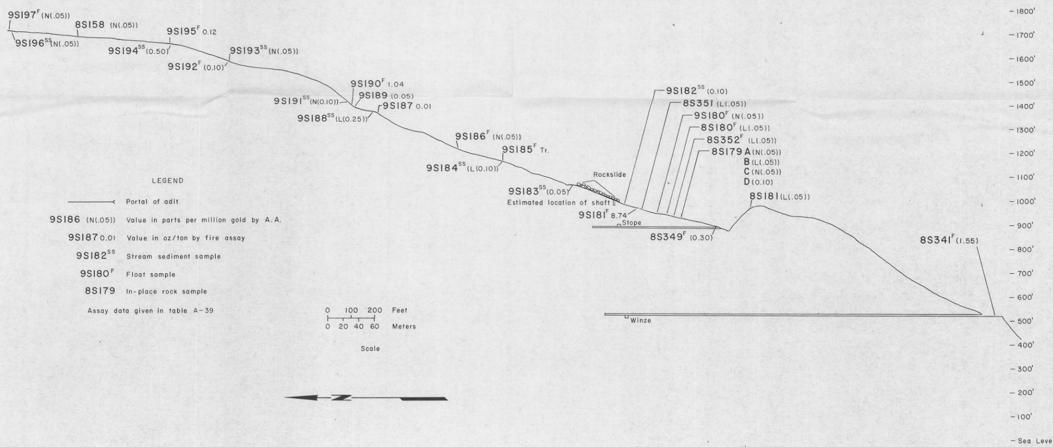
Plate 10.— Cobol mine area map showing workings, surface sample locations, and section along drifts and along gulch north of drifts. View looking east. (Modified from mine map dated 1948)
