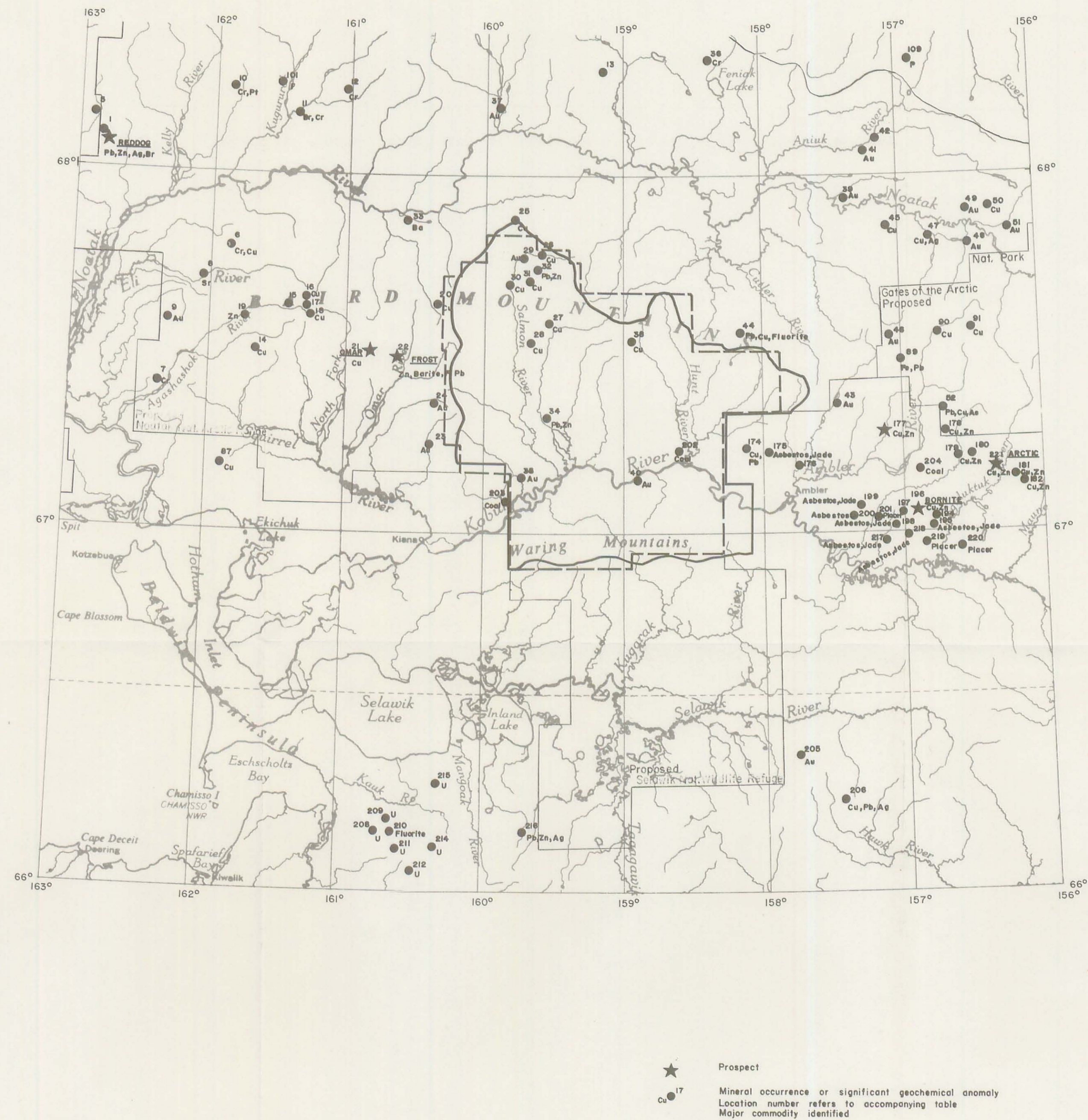
FIGURE 4.- Mineral deposit map of the proposed Kobuk Valley National Monument
