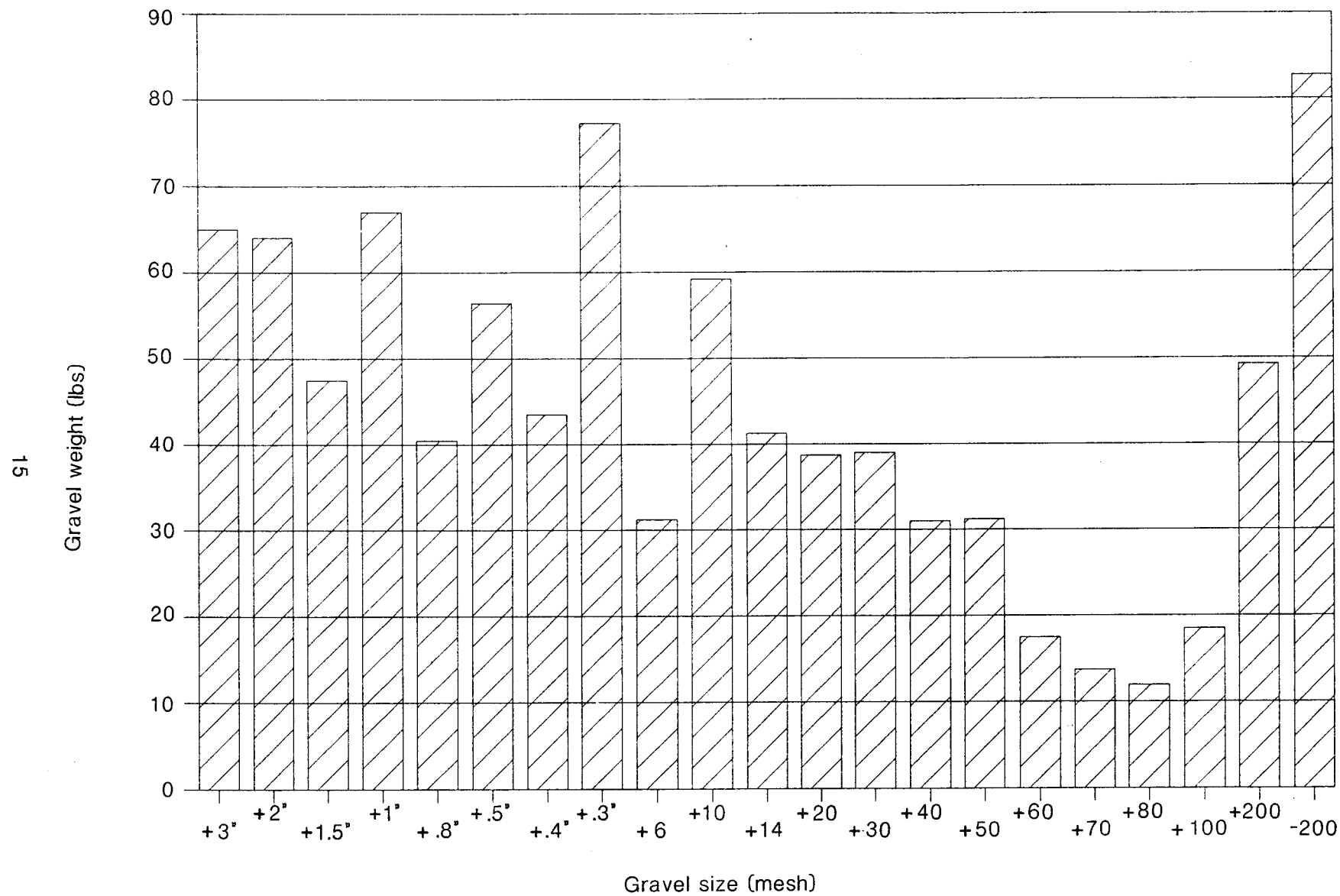
Figure 5. -- Gravel size distribution for the Valdez Creek sample.
