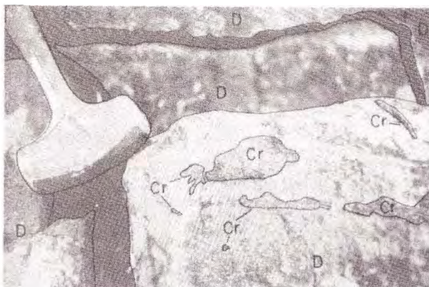
FIGURE 9. - Chromite pods in dunite.
