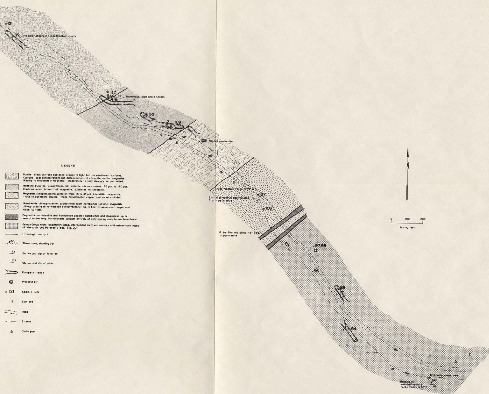
FIGURE 8. -- Geologic map of Fox Gulch
