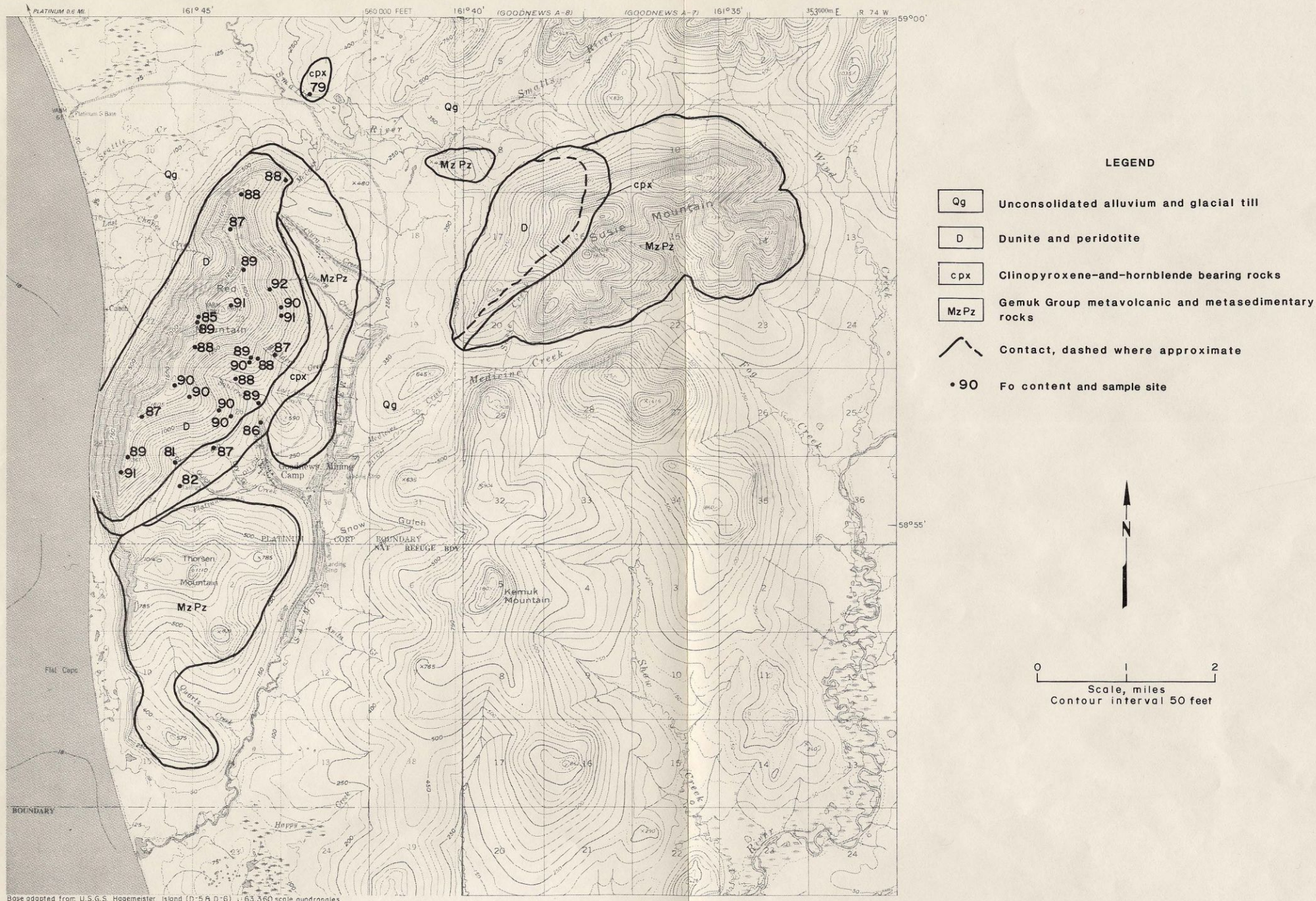
FIGURE 7. -- Distribution of forsterite (Fo) content of olivines in the Goodnews Bay ultramafic complex
