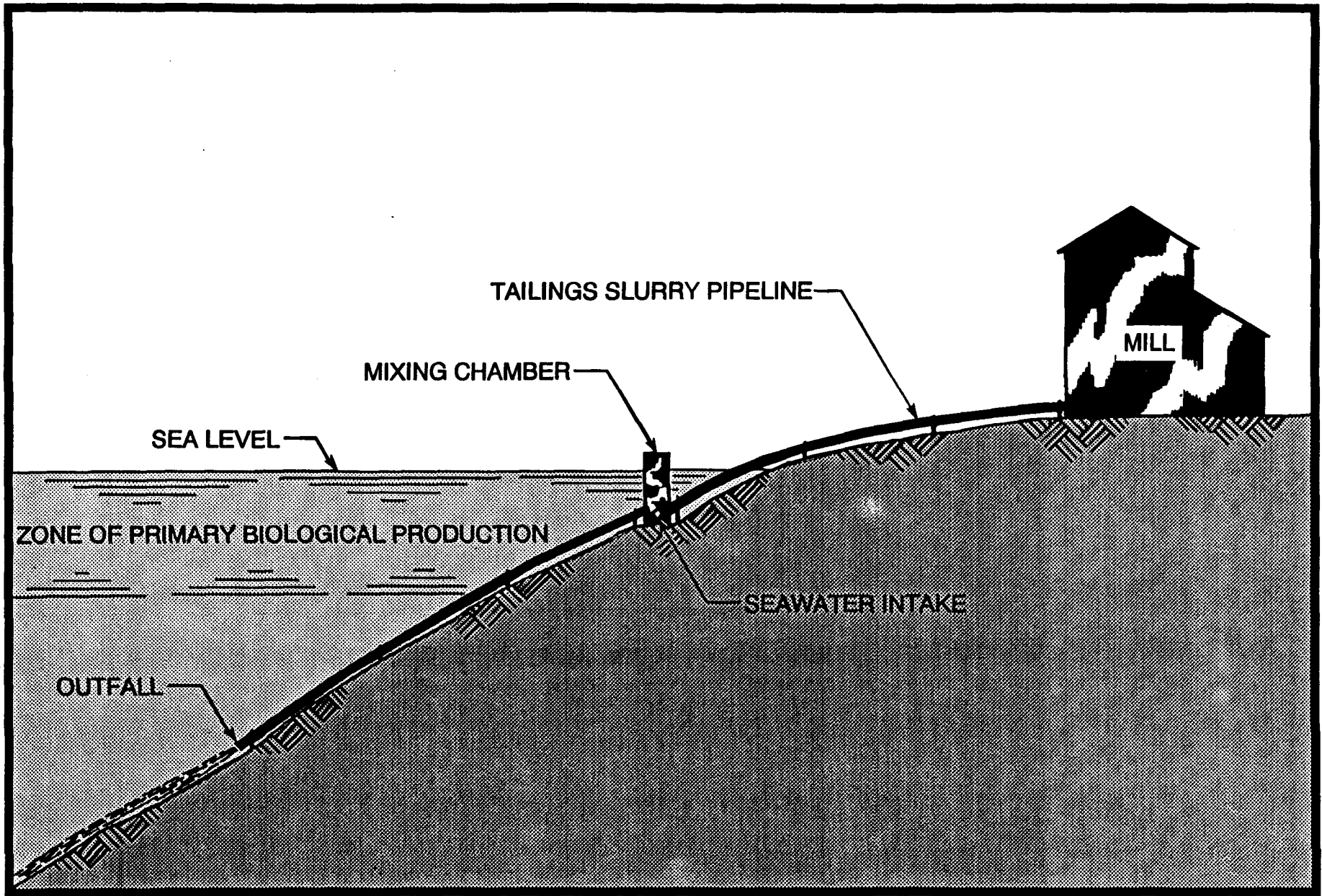
Figure 1. - Generalized Submarine Tailings Discharge System.
