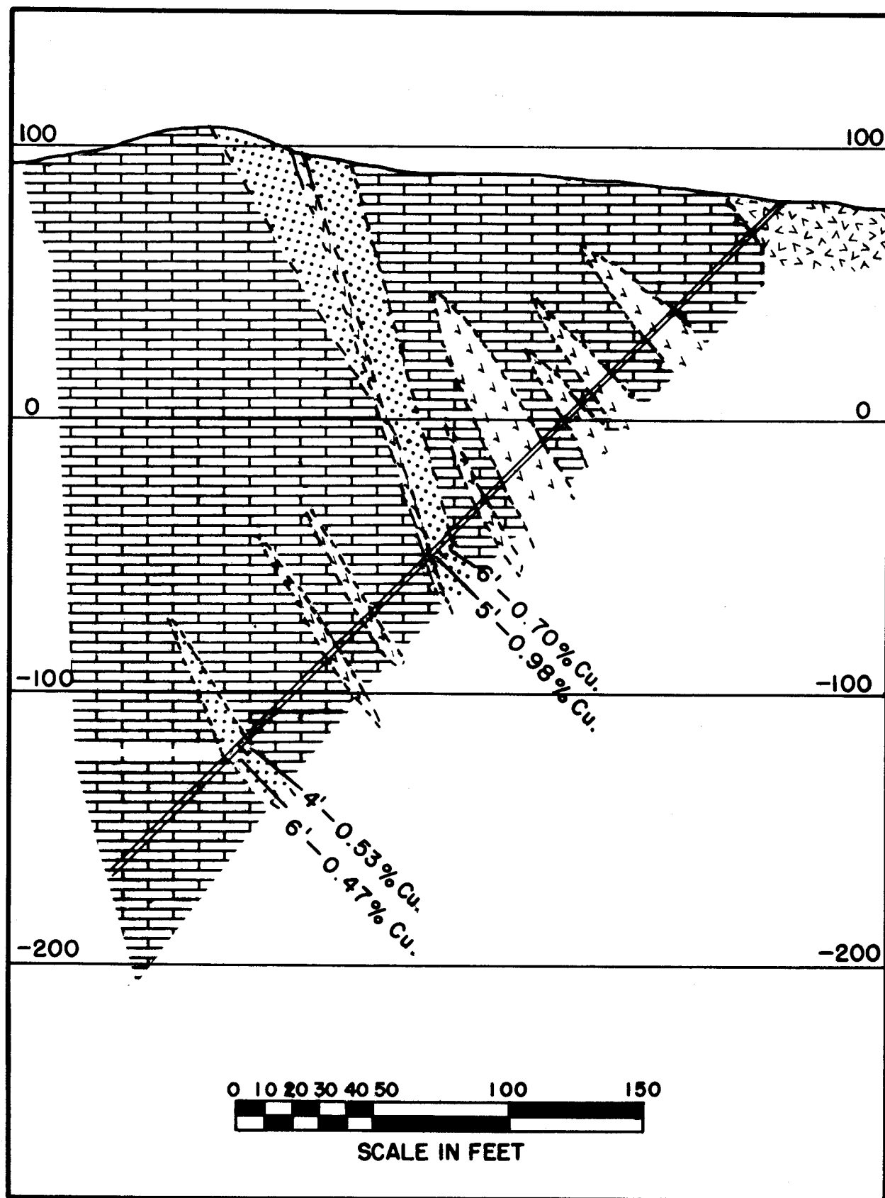
Figure 7. - Section through diamond-drill hole 1.
