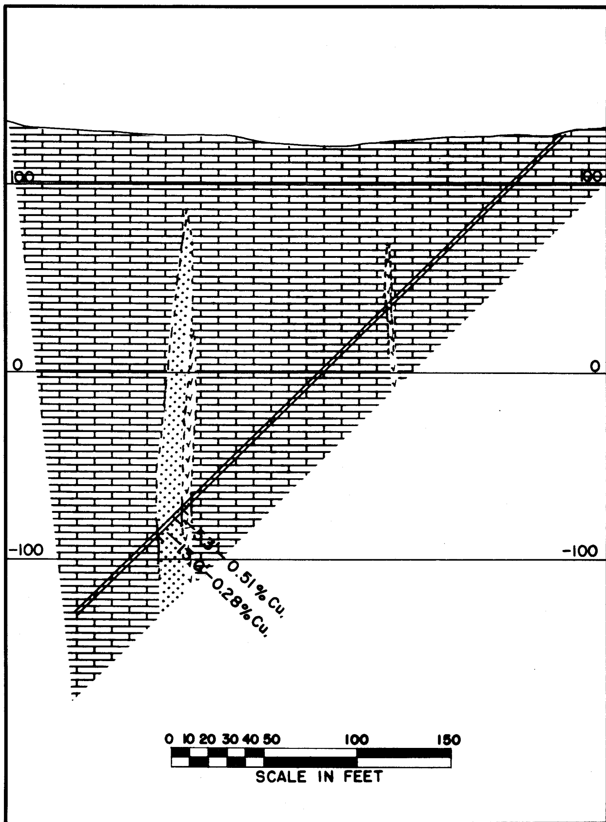
Figure 11. - Section through diamond-drill hole 5.
