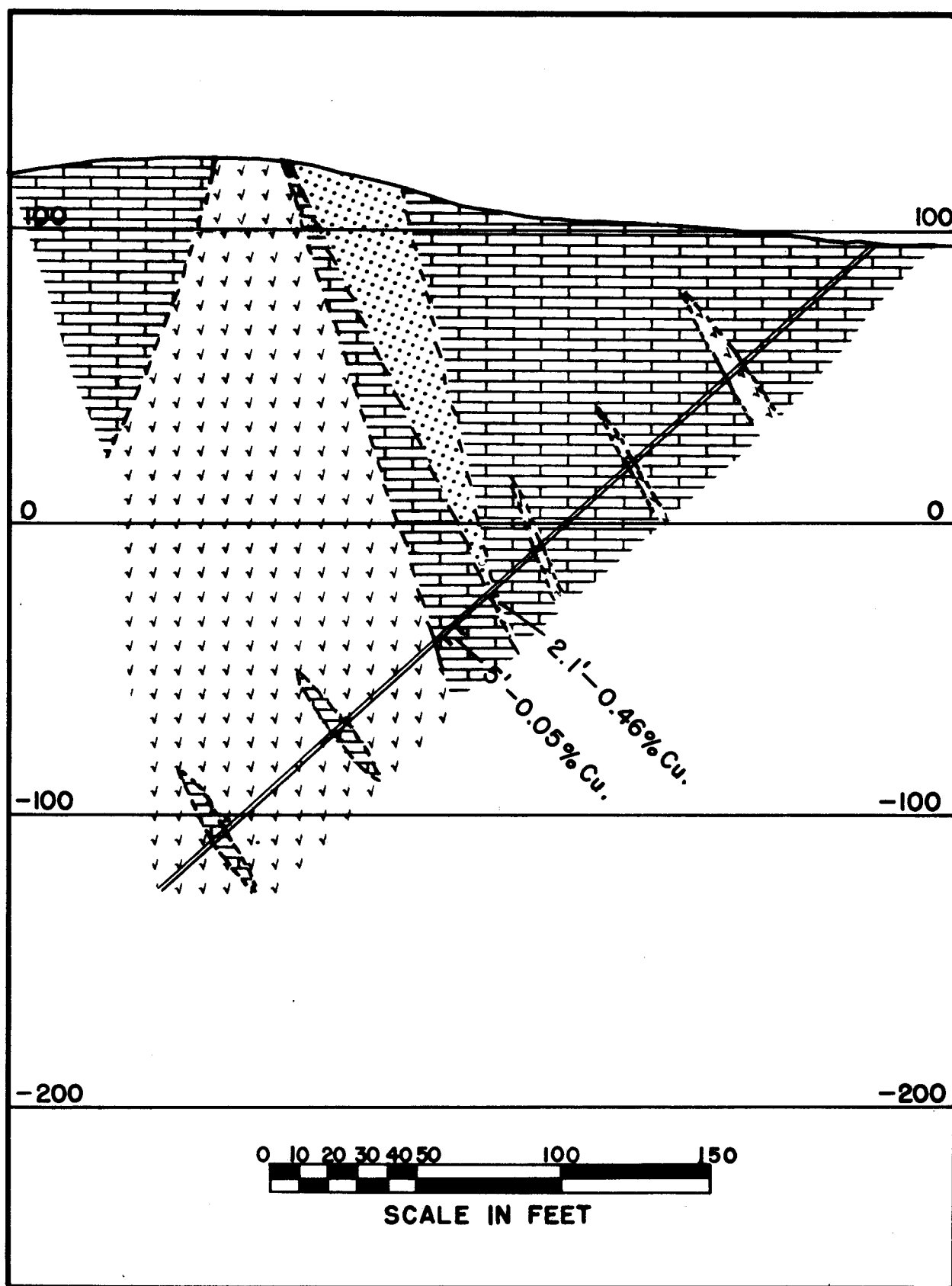
Figure 8. - Section through diamond-drill hole 2.
