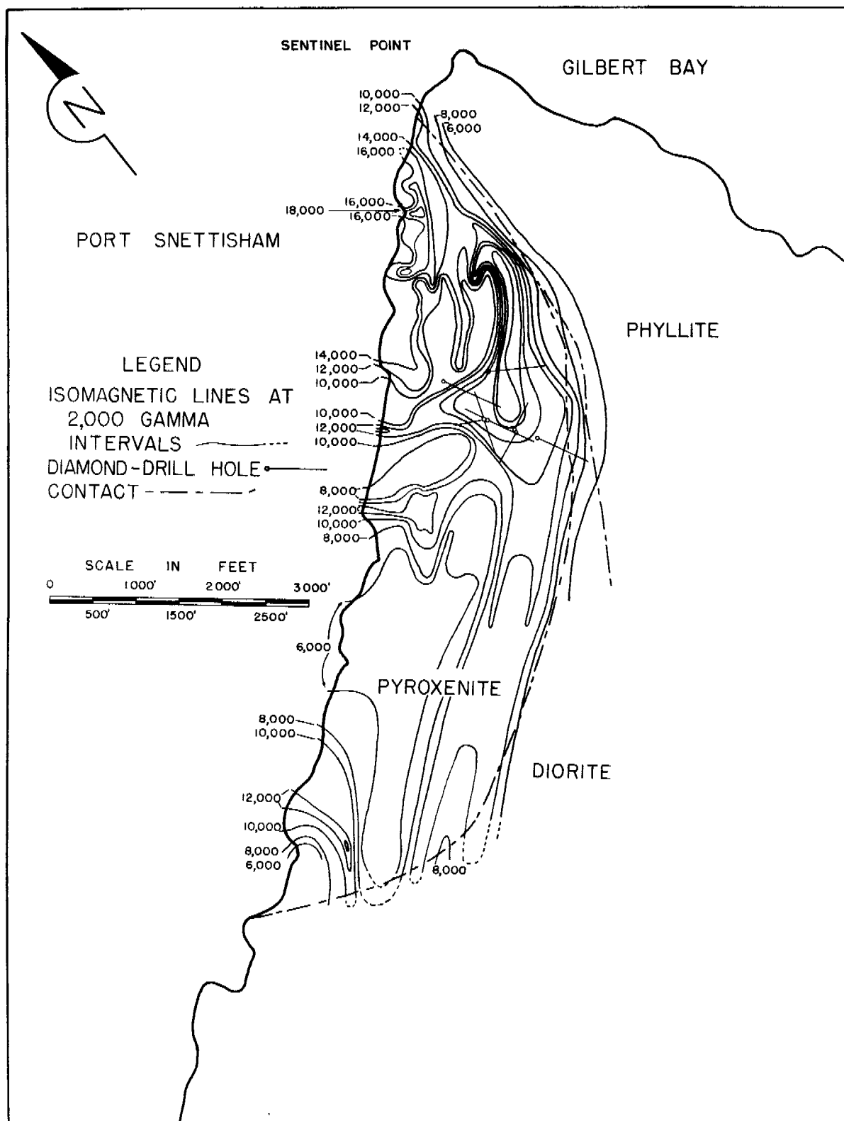
Figure 5. - Magnetometer survey.
