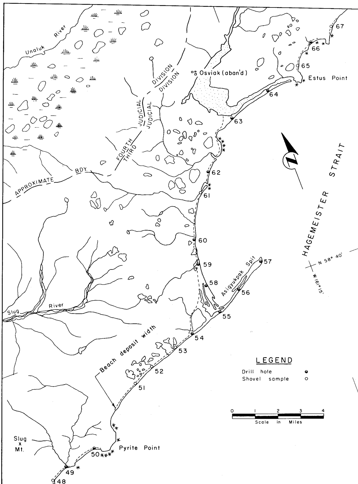
FIGURE 4. - Hagemeister Strait. Adapted from Geological Survey map.
