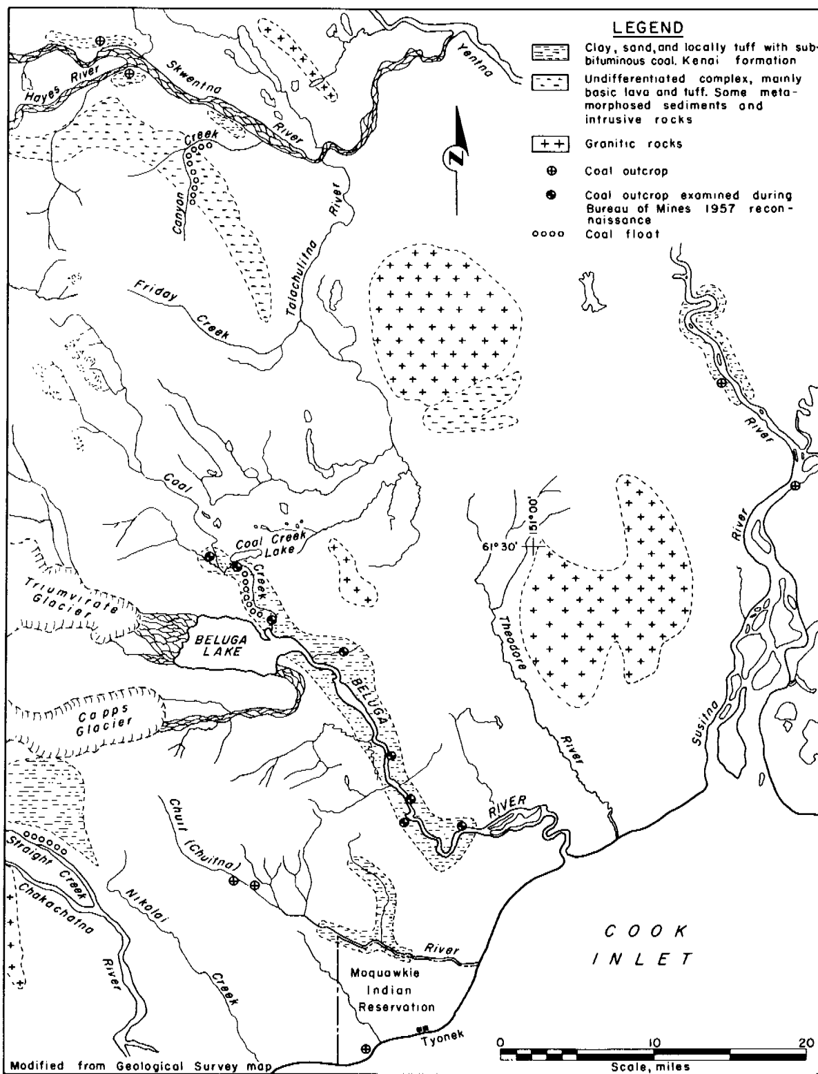
FIGURE 4. - General Geology, Beluga River Coalfield.
