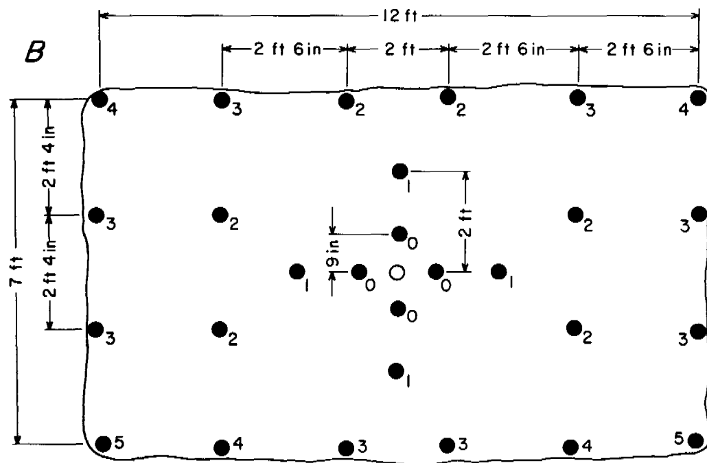
FIGURE 4. - Blast Rounds Used in Factorial Experiment. A , 26-hole V-cut round showing delays. V-holes 7 feet 6 inches deep; "busters" 5 feet deep; all others 7 feet deep. All holes 1½ inches in diameter. B , 29-hole burn-cut round showing delays. All holes 7 feet deep and 1½ inches in diameter.
