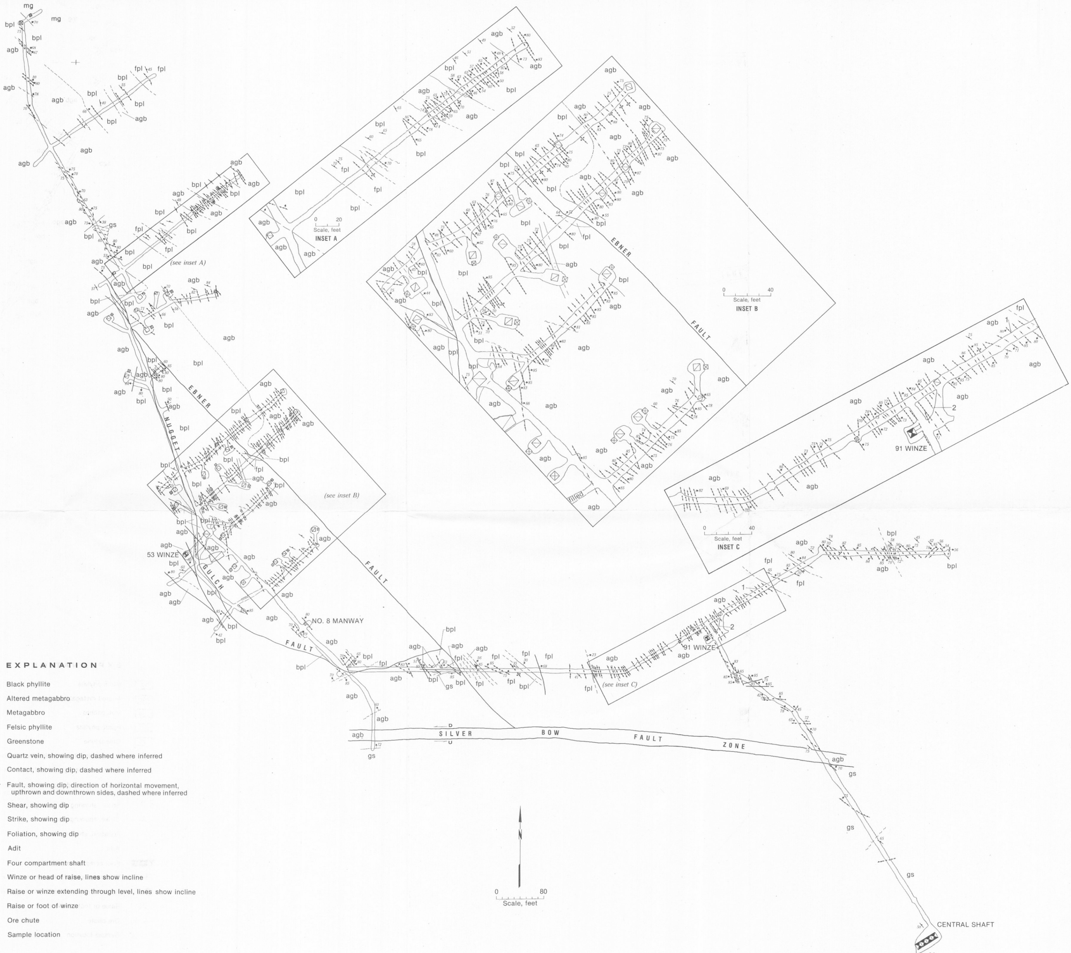
Figure D-21. — Geology and sample locations of the 8-level Alaska Juneau Deep North Orebody.
