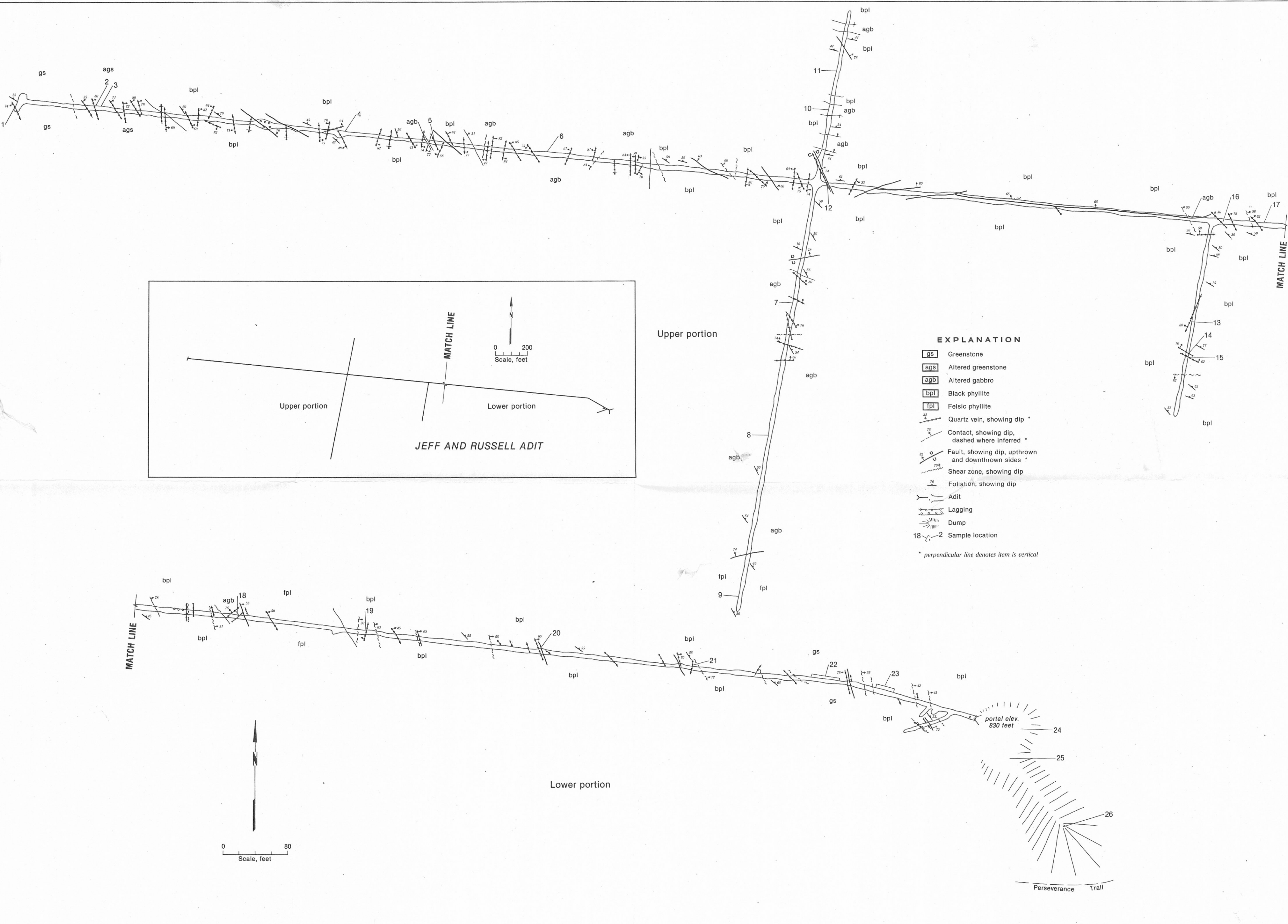
Figure D-125. — The Jeff & Russell adit, showing geology and sample locations.
