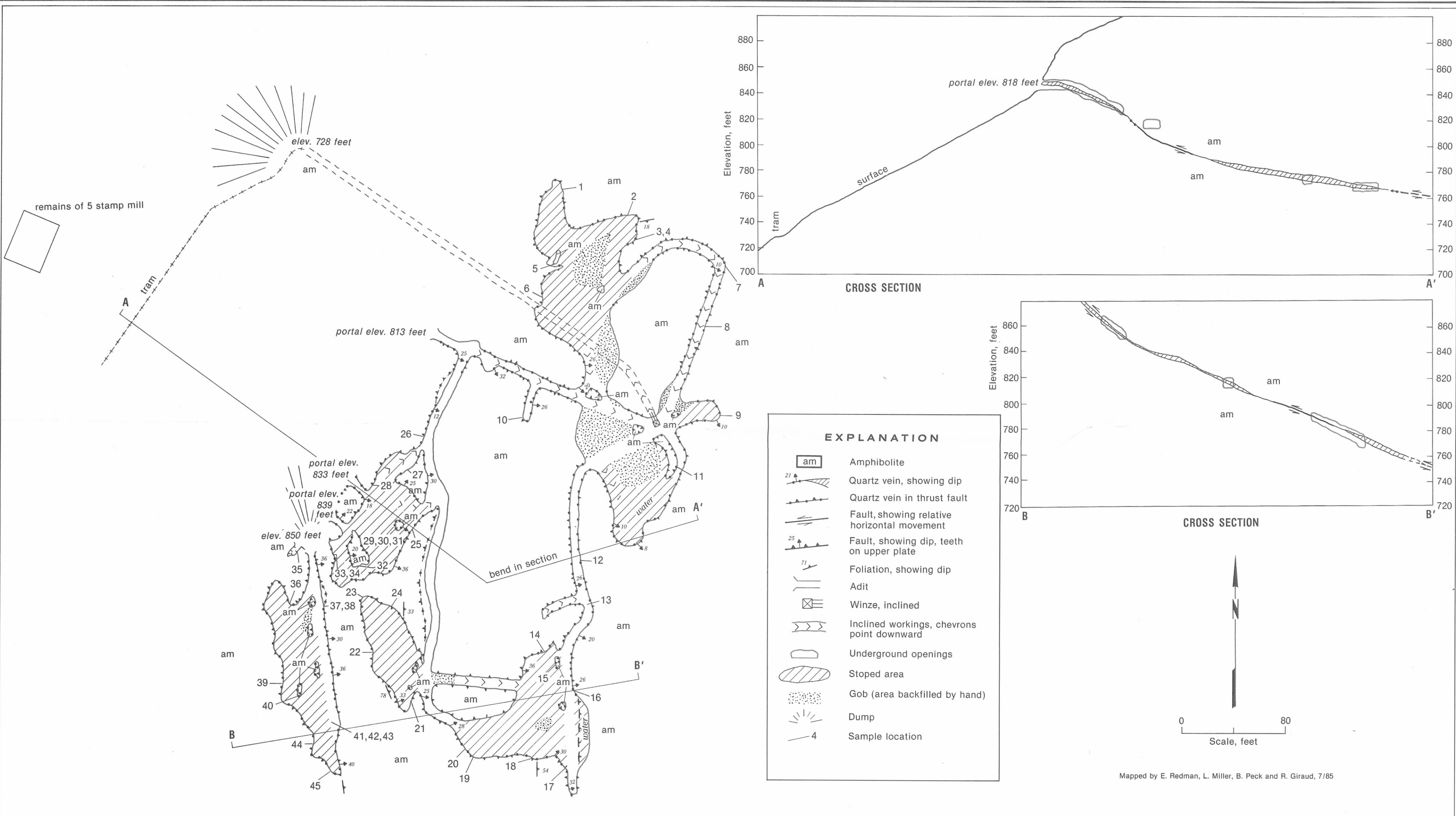
Figure D-221. — The Crystal Mine, showing geology and sample locations.
