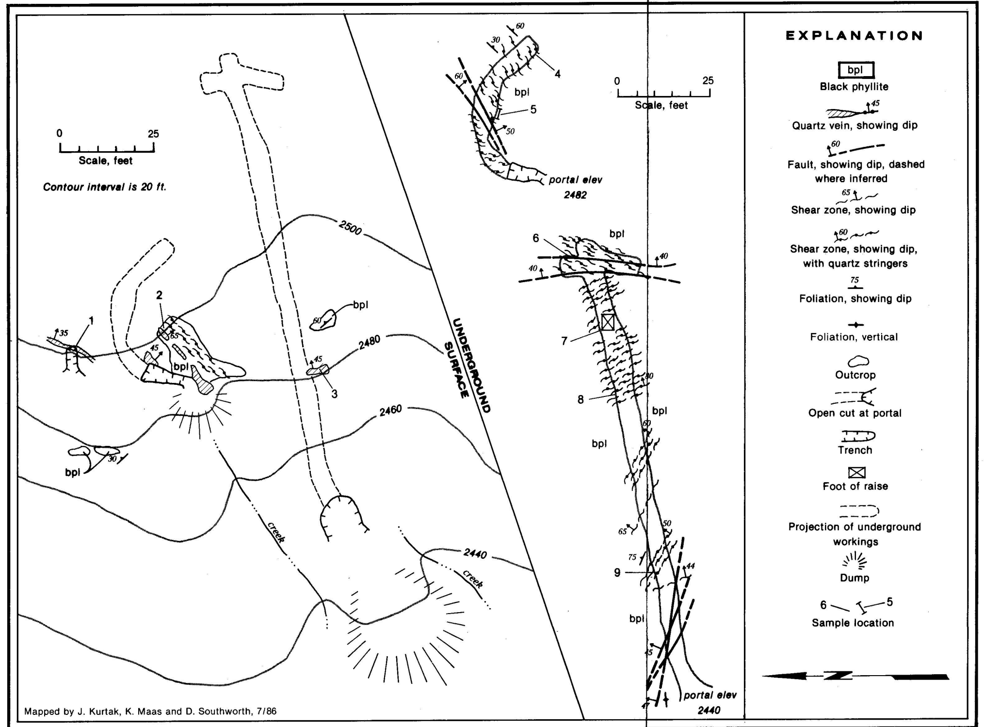
Figure D-61. — Maude S prospect, showing geology, workings, and sample locations.
