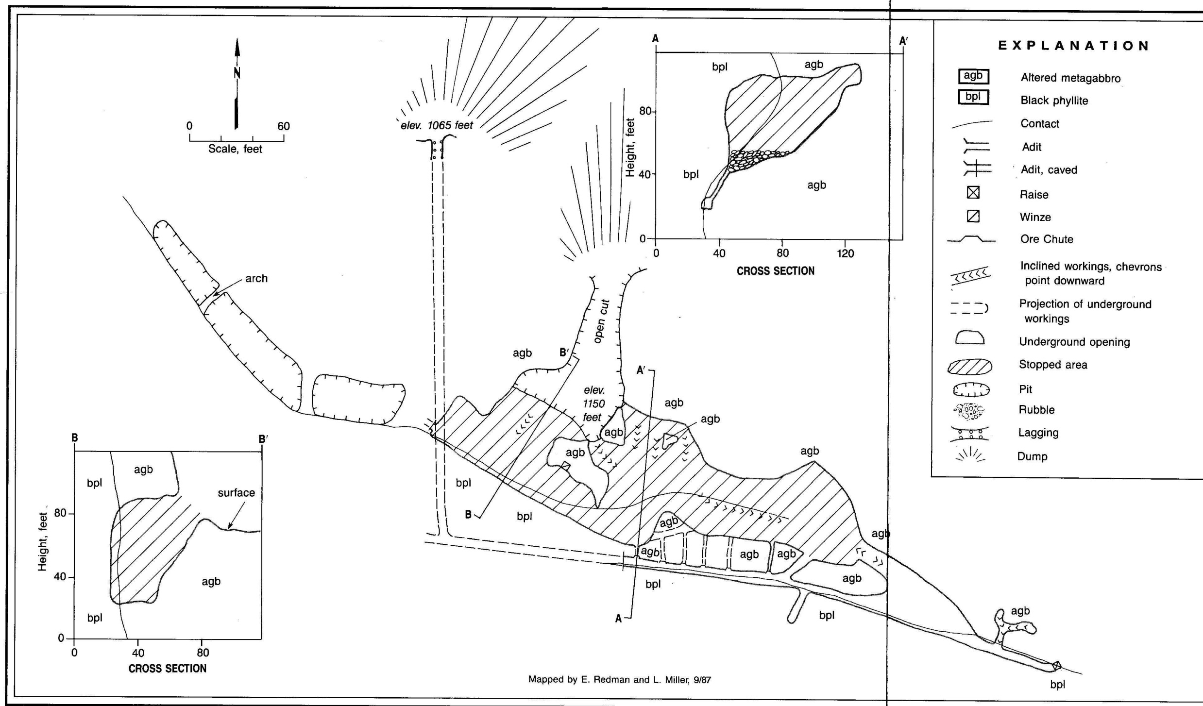
Figure D-132. — The upper Ebner workings, stopes, and pits, showing geology and sample locations.
