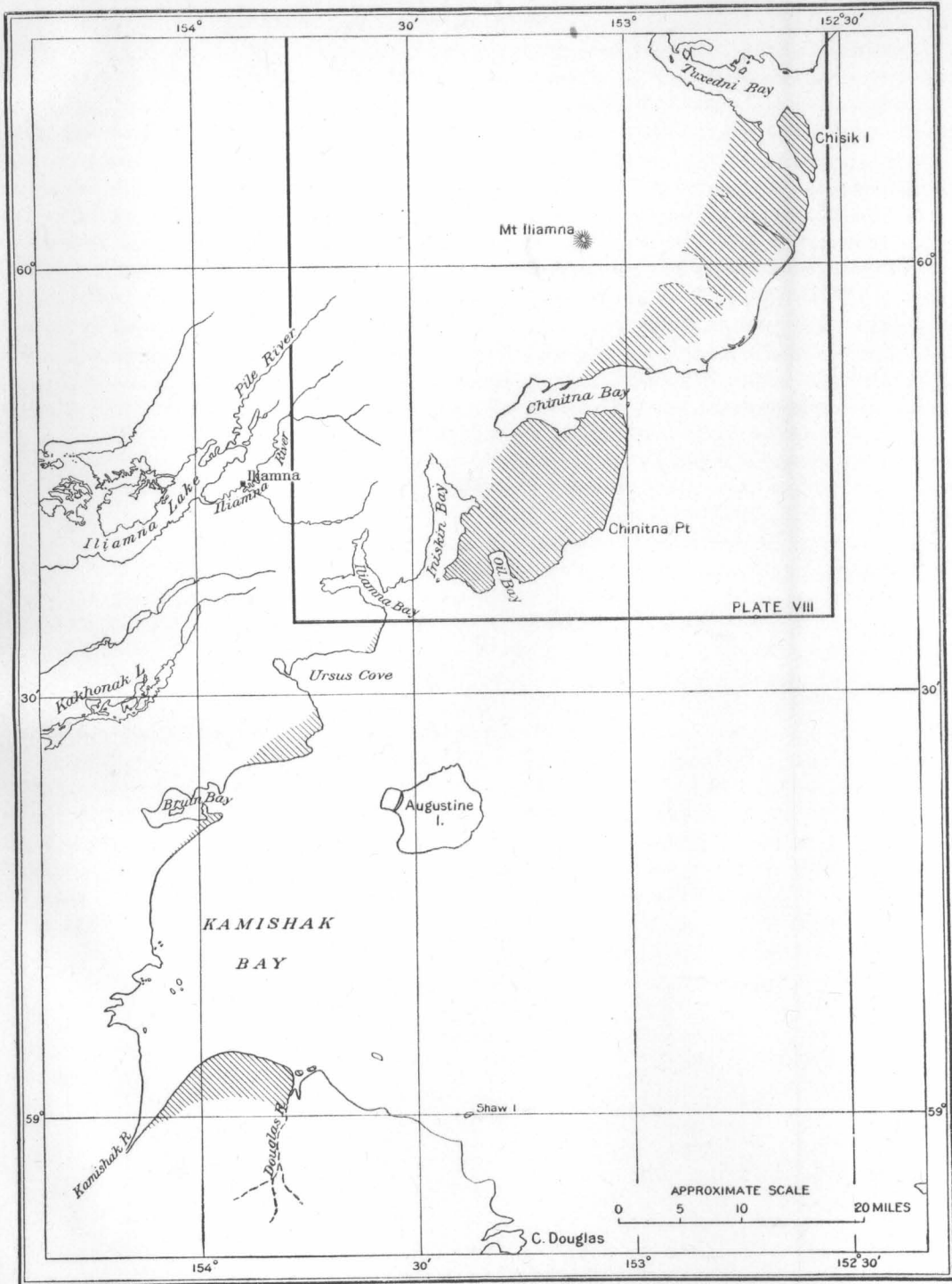
MAP OF PART OF WEST SHORE OF COOK INLET, SHOWING DISTRIBUTION OF JURASSIC SEDIMENTARY ROCKS.
