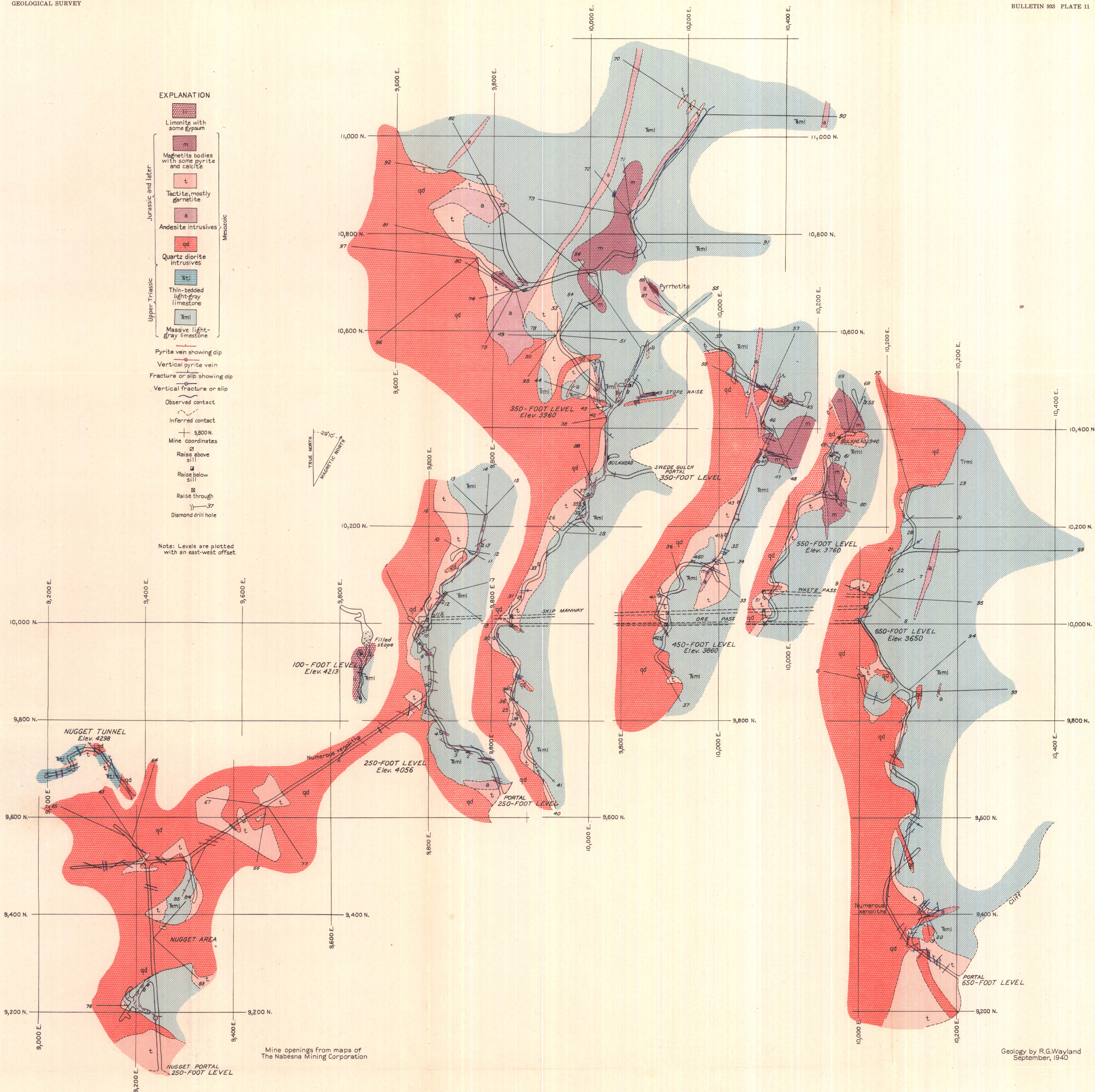
GEOLOGIC MAPS OF UNDERGROUND WORKINGS, NABESNA MINE
