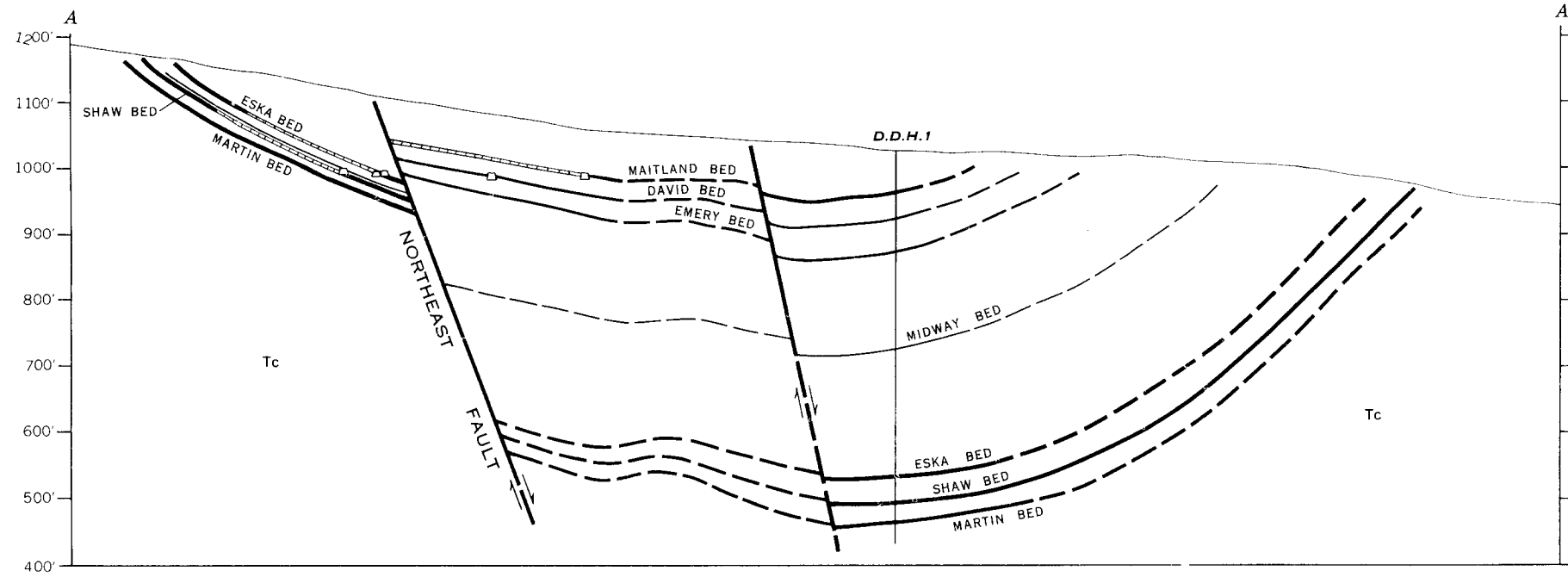
For location of section see plate 3
