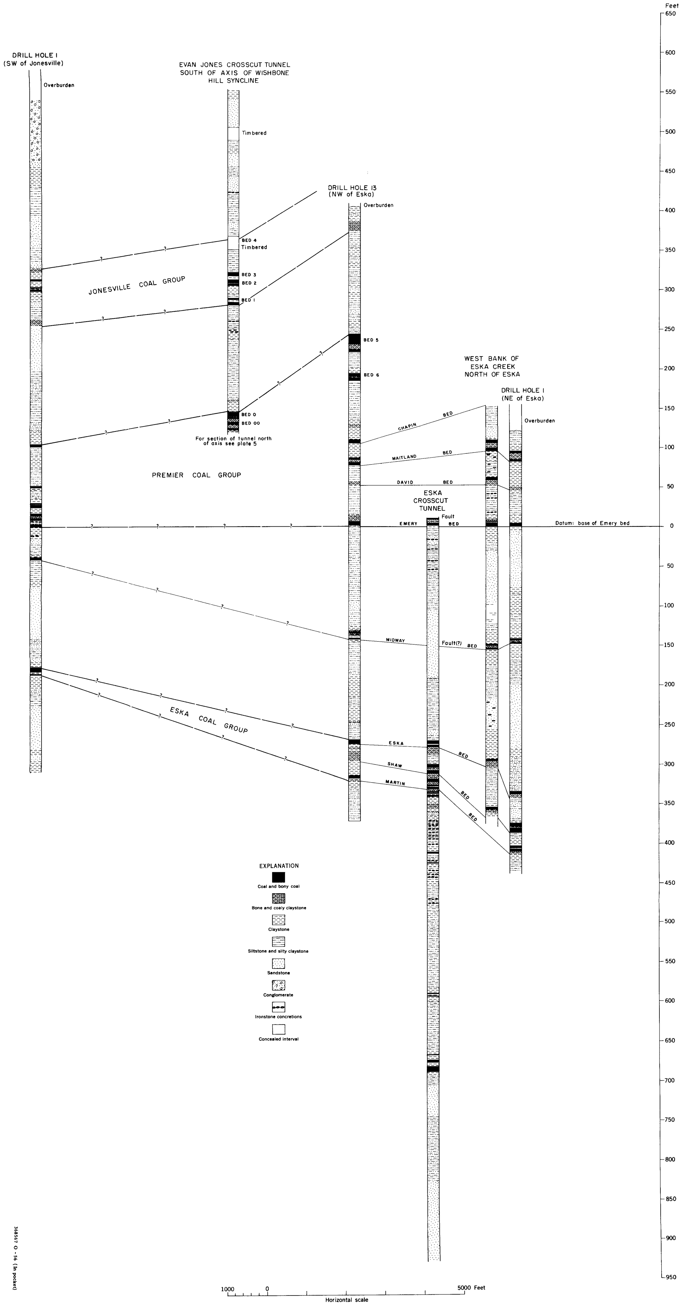
CORRELATED STRATIGRAPHIC SECTIONS IN THE ESKA-JONESVILLE AREA OF WISHBONE HILL DISTRICT, MATANUSKA COAL FIELD, ALASKA
