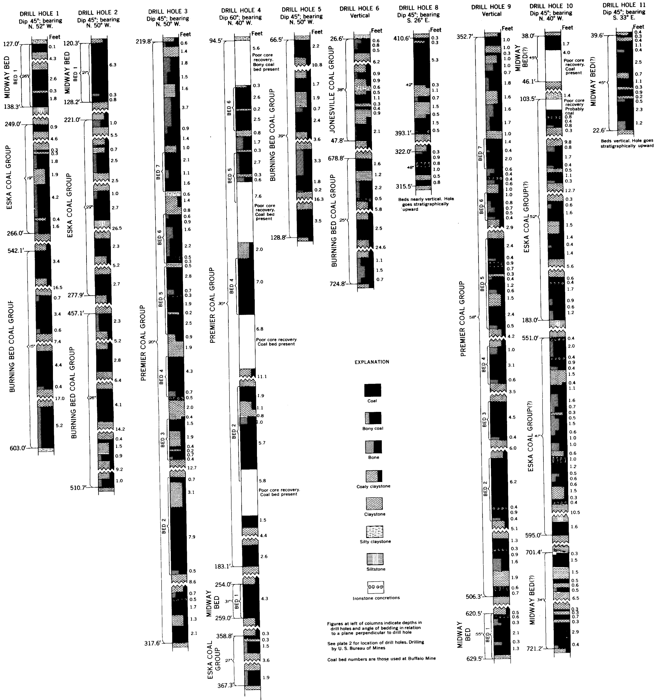
TRUE-THICKNESS LOGS OF COAL BEDS IN DIAMOND-DRILL HOLES ALONG MOOSE CREEK, WISHBONE HILL DISTRICT, MATANUSKA COAL FIELD, ALASKA
