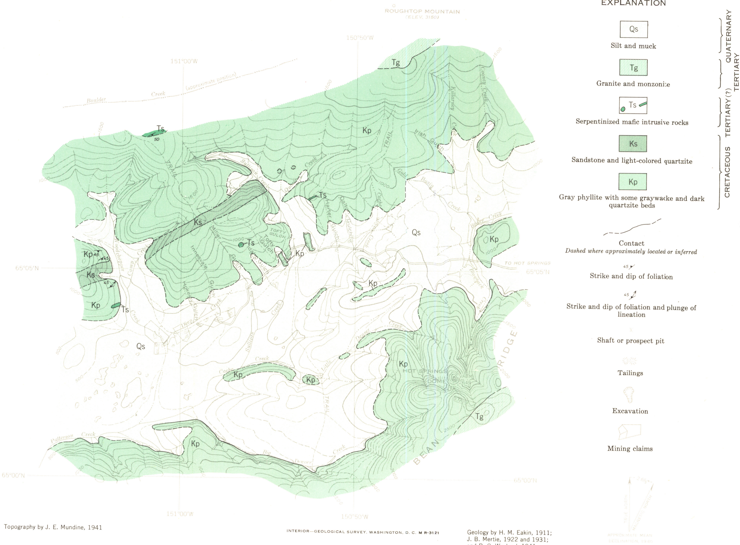
GEOLOGIC MAP OF THE TOFTY AREA, MANLEY HOT SPRINGS DISTRICT, ALASKA
