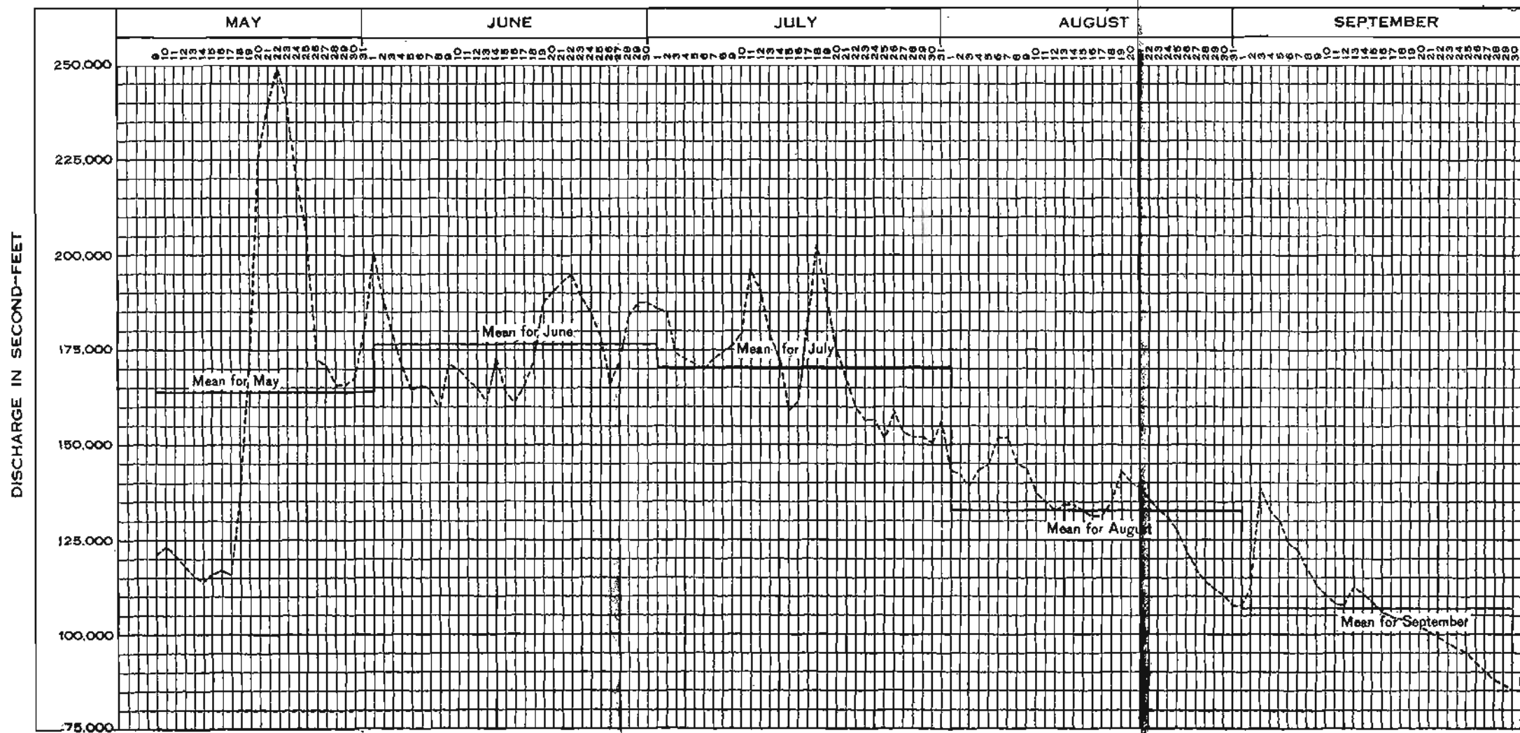
HYDROGRAPH SHOWING DAILY DISCHARGE OF YUKON RIVER AT EAGLE.
