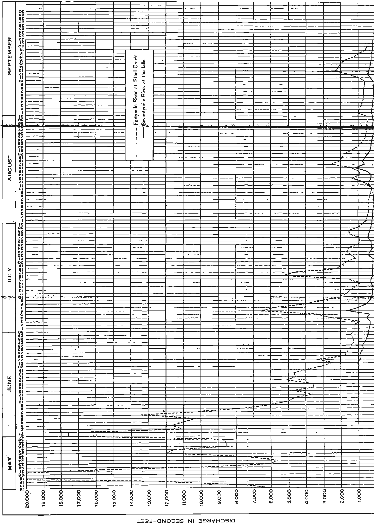
HYDROGRAPH SHOWING DAILY DISCHARGE OF FORTYMILE AND SEVENTYMILE RIVERS
