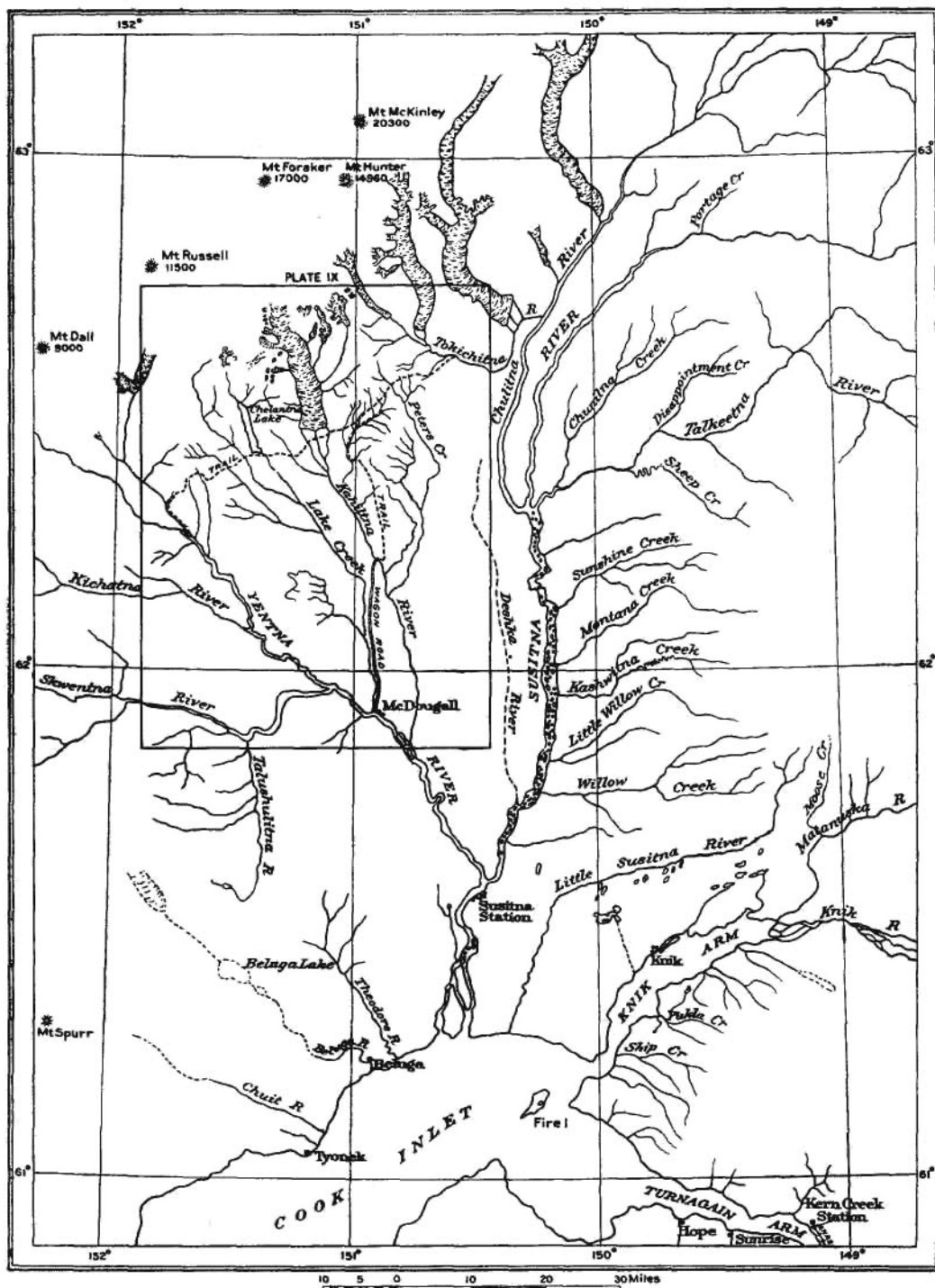
SKETCH MAP OF SUSITNA BASIN.
