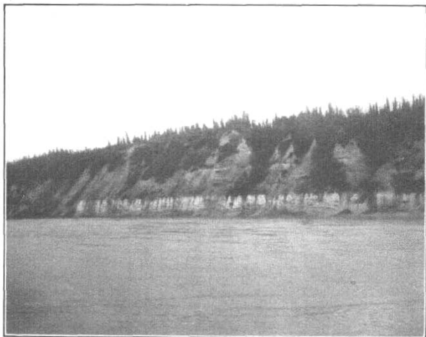
B. EOCENE BEDS OVERLAIN UNCONFORMABLY BY SILTS IN THE PALISADES OF THE YUKON.
