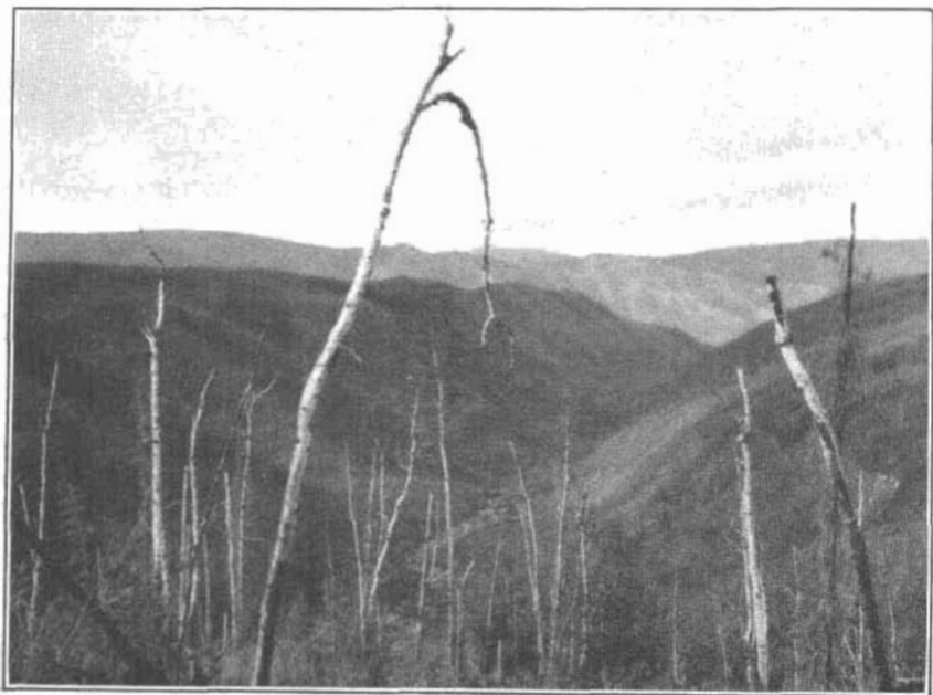
B. LITTLE MINOOK CREEK, SEEN FROM IDAHO BAR.
