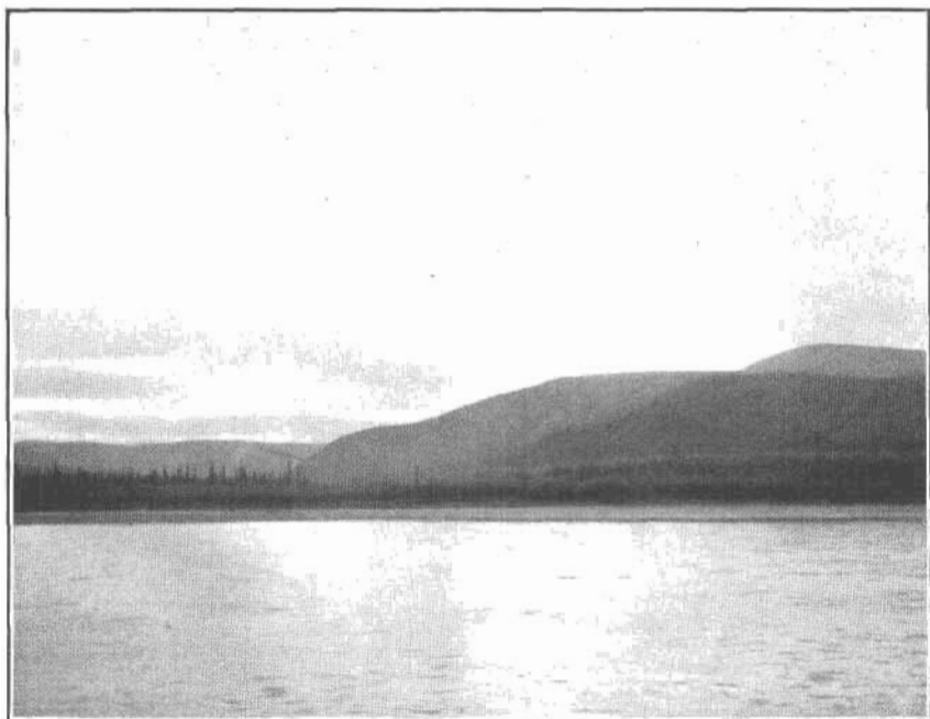
B. VIEW UP MINOOK VALLEY FROM THE YUKON.
