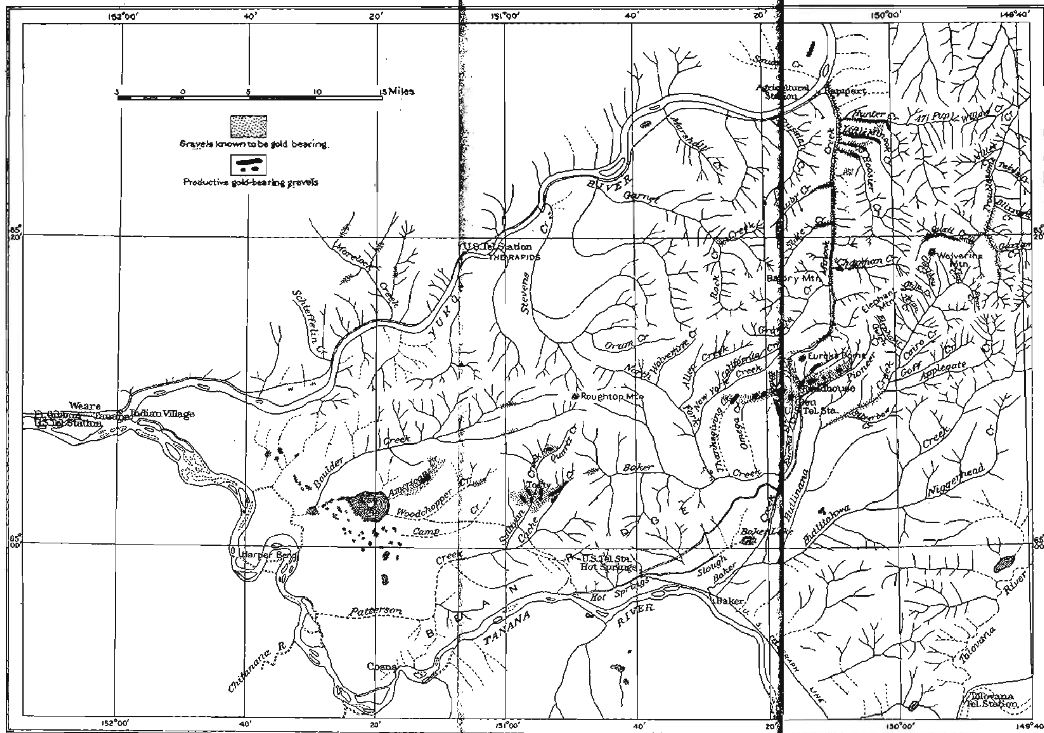
MAP OF RAMPART AND HOT SPRINGS DISTRICTS, ALASKA, SHOWING DISTRIBUTION OF PLACER GOLD.
