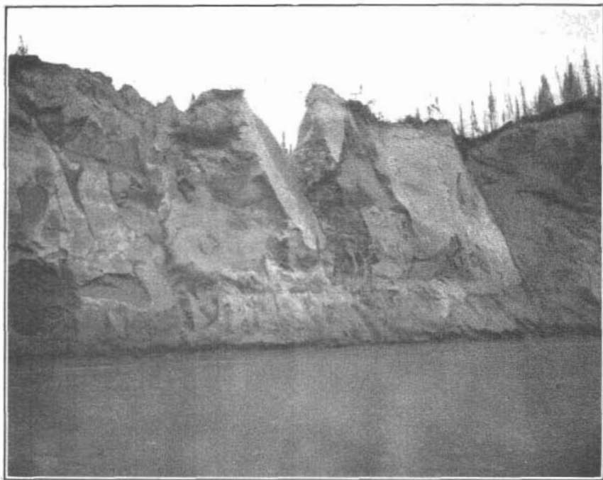
B. MASSIVE DEPOSIT OF SILT AT THE PALISADES OF THE YUKON, 25 MILES BELOW TANANA.
