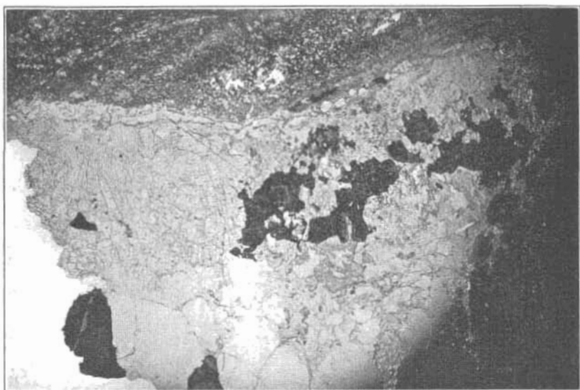
B. THIN SECTION OF CASSITERITE VEIN IN LIMESTONE NEAR CASSITERITE LODE.
