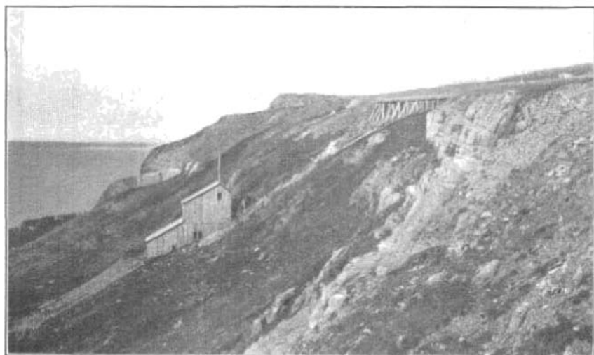
B. UPLAND SURFACE (1,000-FOOT TERRACE) AT CAPE MOUNTAIN. Empire Tin Mining Co.'s mill in the foreground; Bering Sea at the left.
