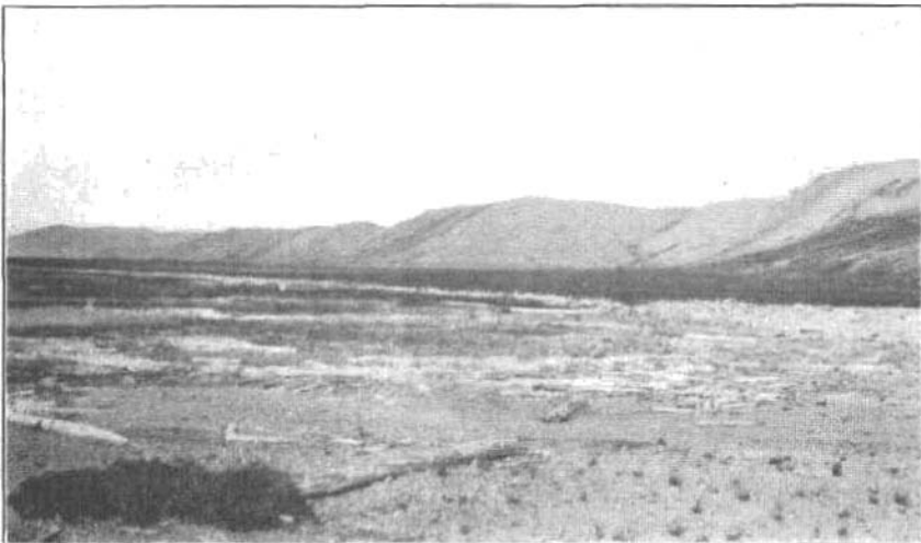
B. SEA CLIFFS AND TERRACE EAST OF LOST RIVER.
