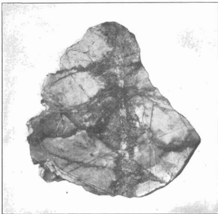
A. POLISHED SURFACE OF ALTERED LIMESTONE NEAR CASSITERITE LODE.
