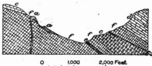
FIGURE 22.—Section near Willow Branch. a , Amygdaloid; b , porphyry dikes and quartz; c , metamorphosed limestone; d , Port Clarence limestone; e , gabbro and basalt; f , slate.
