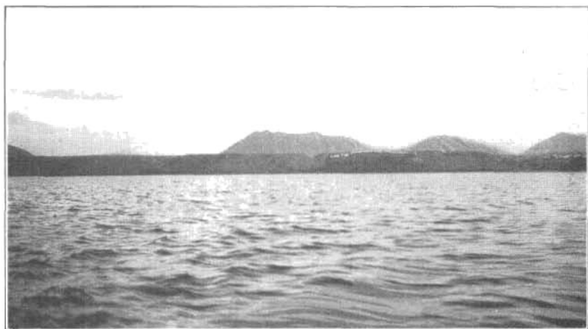
B. THE SEA TERRACE NEAR LOST RIVER.
