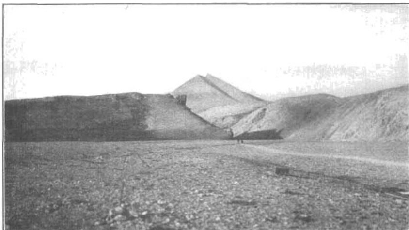
A. CANYON NEAR THE MOUTH OF LOST RIVER.
