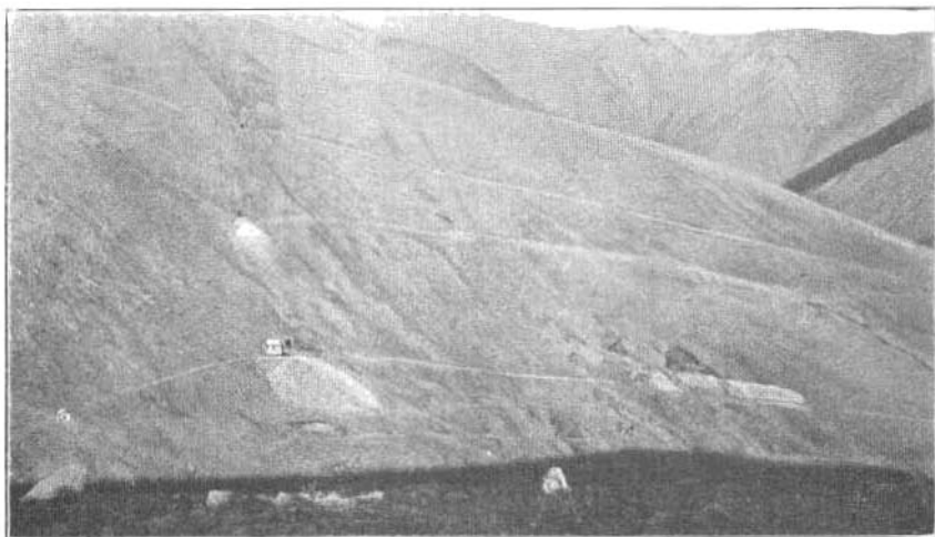
A. WORKINGS ON CASSITERITE DIKE ON EAST SIDE OF CASSITERITE CREEK (AT LEFT) AND ON THE GREENSTONE LODGE (AT RIGHT).
