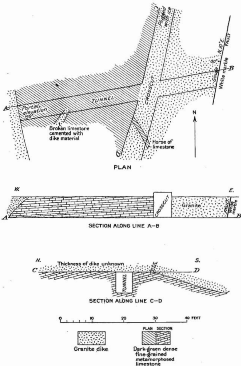
FIGURE 9.—Plan and sections of workings on Greenstone lode.
