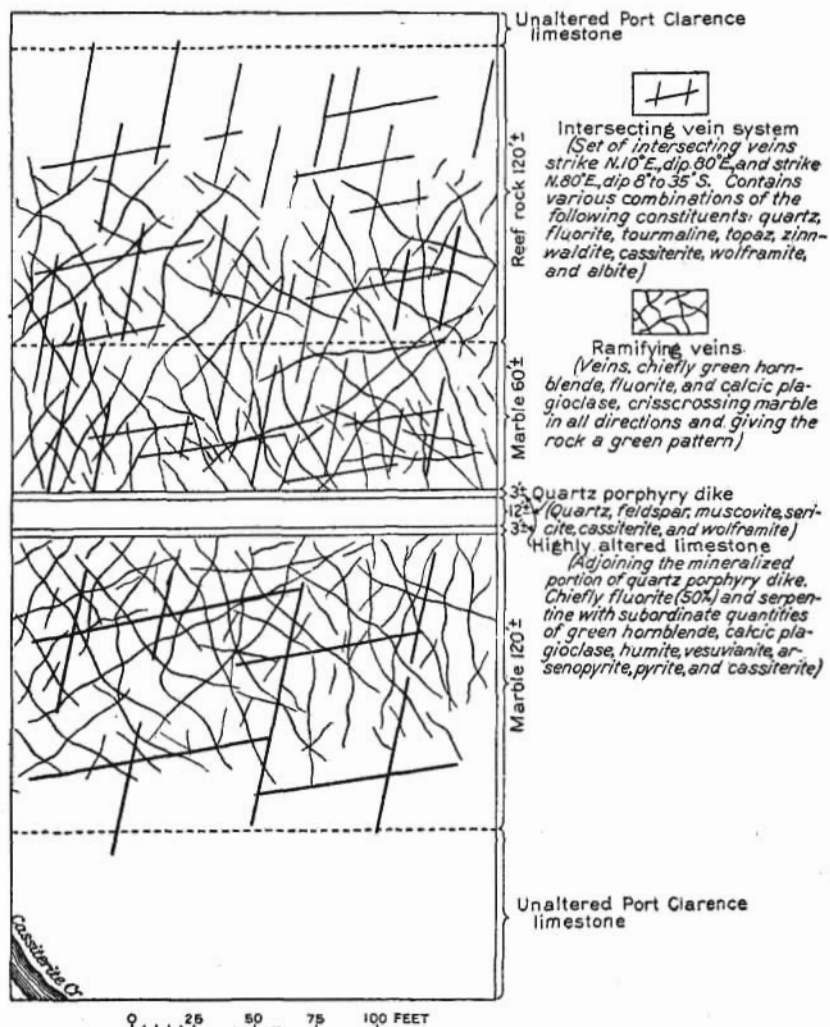
FIGURE 6.—Idealized sketch showing mineralization of limestone at Cassiterite Creek tin prospect.
