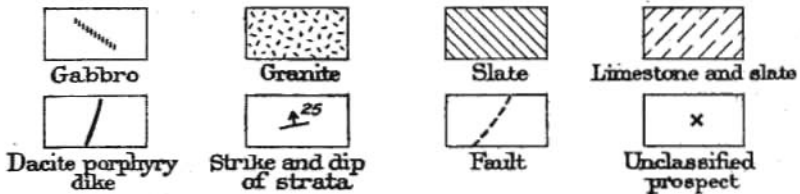
FIGURE 18.—Geologic sketch map of Ear Mountain. A-B, line of section, figure 19.
