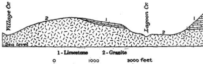
FIGURE 16.—Geologic section across Lagoon Creek, Cape Mountain.
