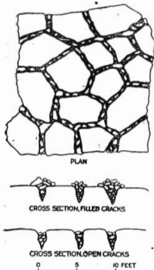
FIGURE 3.—Frost-crack pattern.
