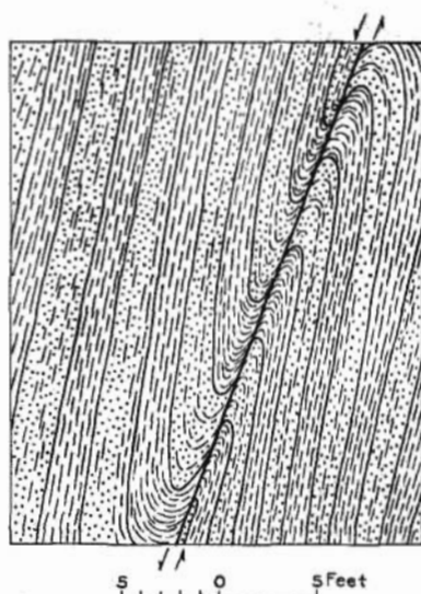
FIGURE 47.—Normal fault caused by compressive stresses.
