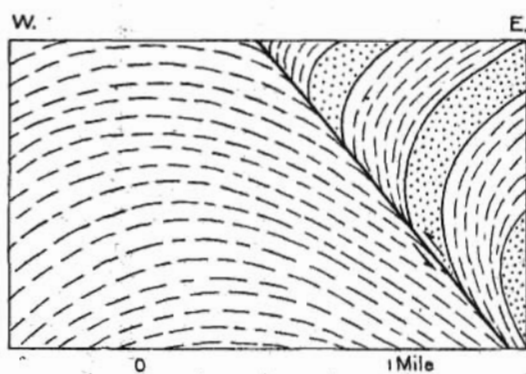
FIGURE 46.—Goat Mountain thrust fault.
