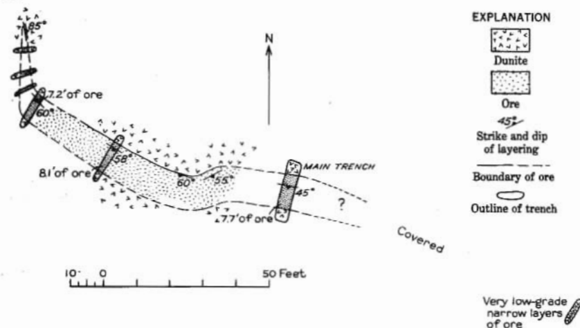
Figure 15.—Sketch map of Juneau No. 1 deposit, Red Mountain.
