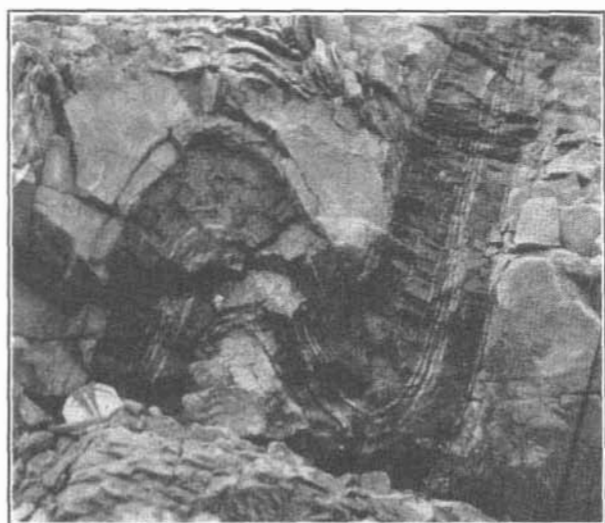
B. DRAG FOLD, DEPOSIT No. 13, RED MOUNTAIN.
