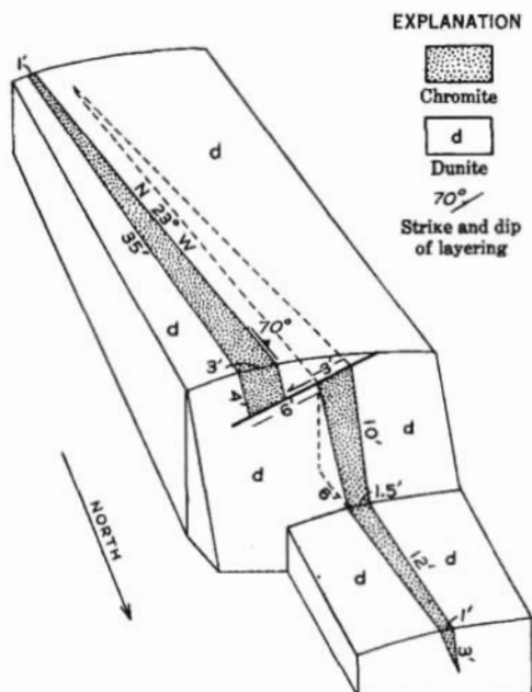
Figure 14.--Block diagram of deposit No. 5, Red Mountain.
