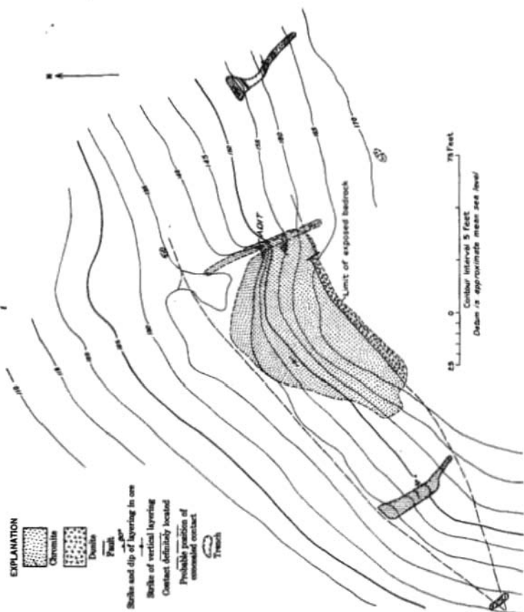
Figure 13.--Geologic map of the Bluff No. 1 deposit, Claim Point.
