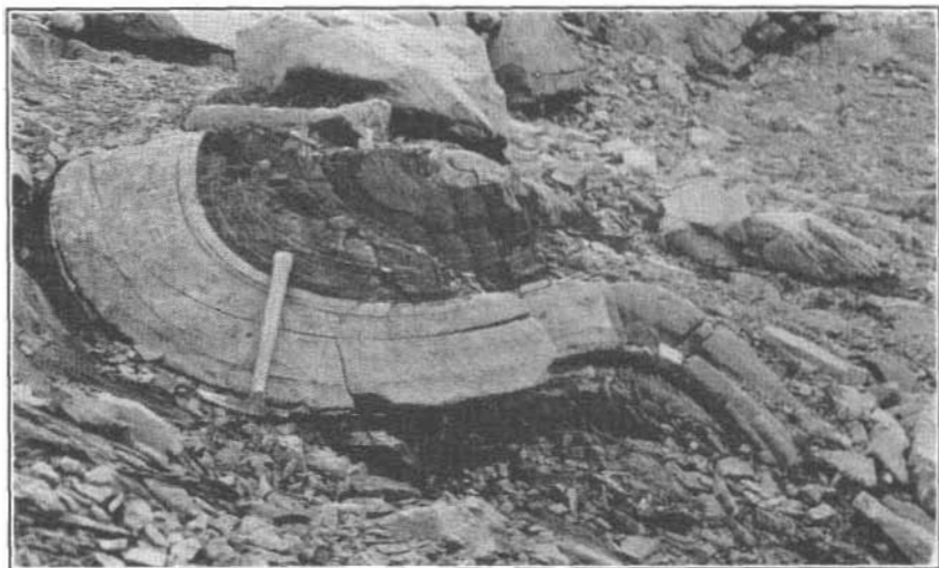
A. DRAG FOLD IN CHROMITE, DEPOSIT No. 24, RED MOUNTAIN.
