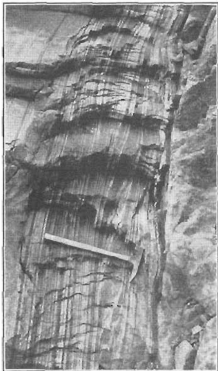
A. BANDED DISSEMINATED ORE. DEPOSIT No. 20, RED MOUNTAIN.
