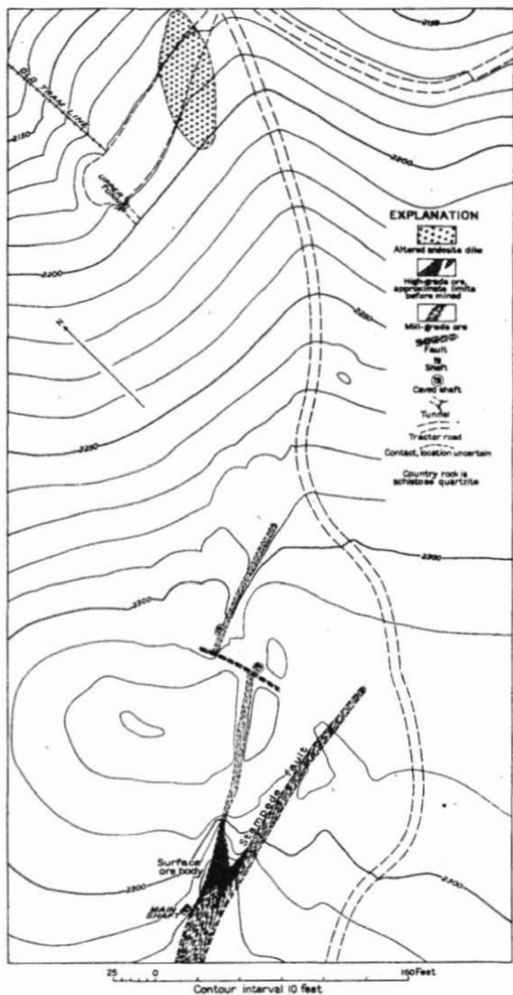
Figure 39.--Geologic map of the surface workings of the Stampede antimony mine.
