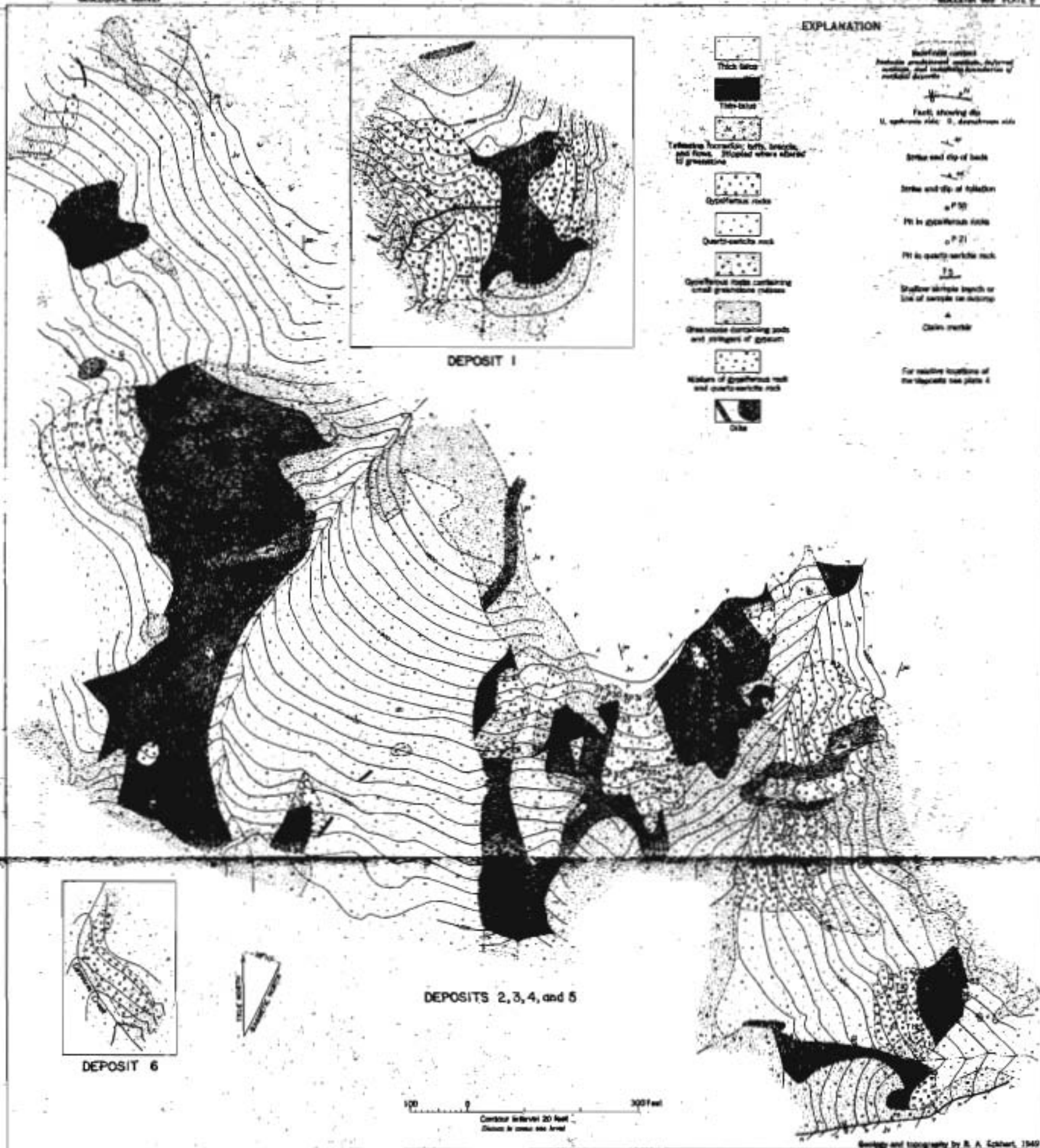
GEOLOGIC MAP OF GYPSIFEROUS DEPOSITS, SHEEP MOUNTAIN, ALASKA
