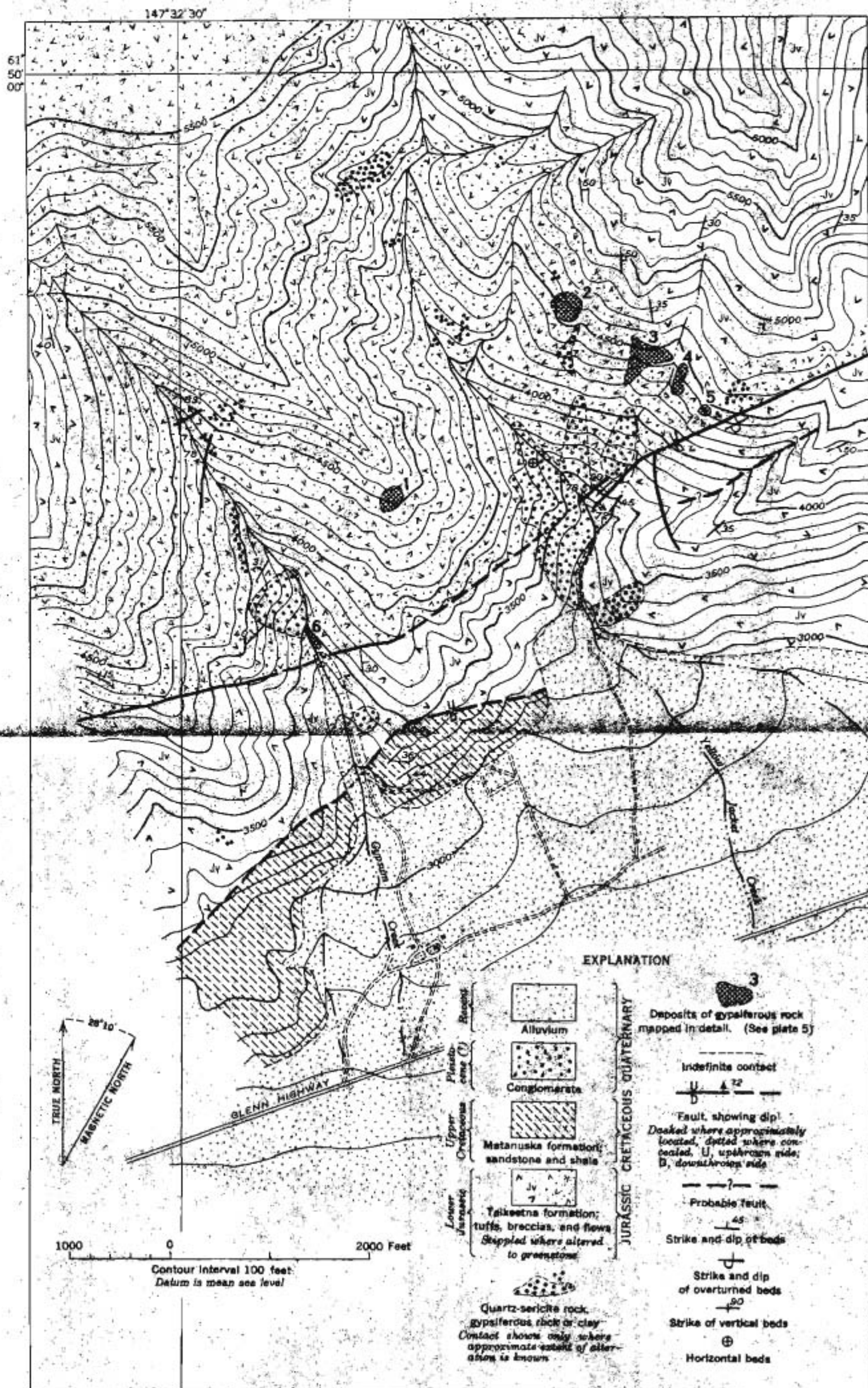
GEOLOGIC MAP OF AREA OF GYPSUM AND YELLOW JACKET CREEKS, SHEEP MOUNTAIN, ALASKA
