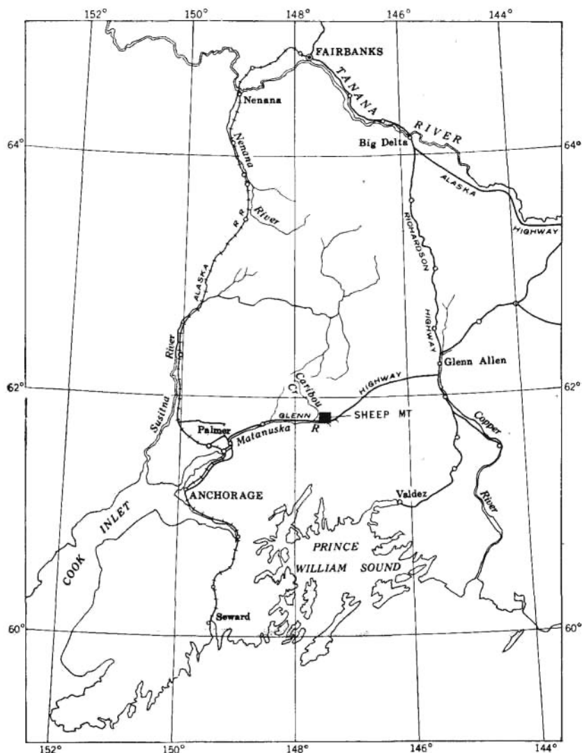
FIGURE 12.—Index map of south central Alaska showing location of Sheep Mountain.
