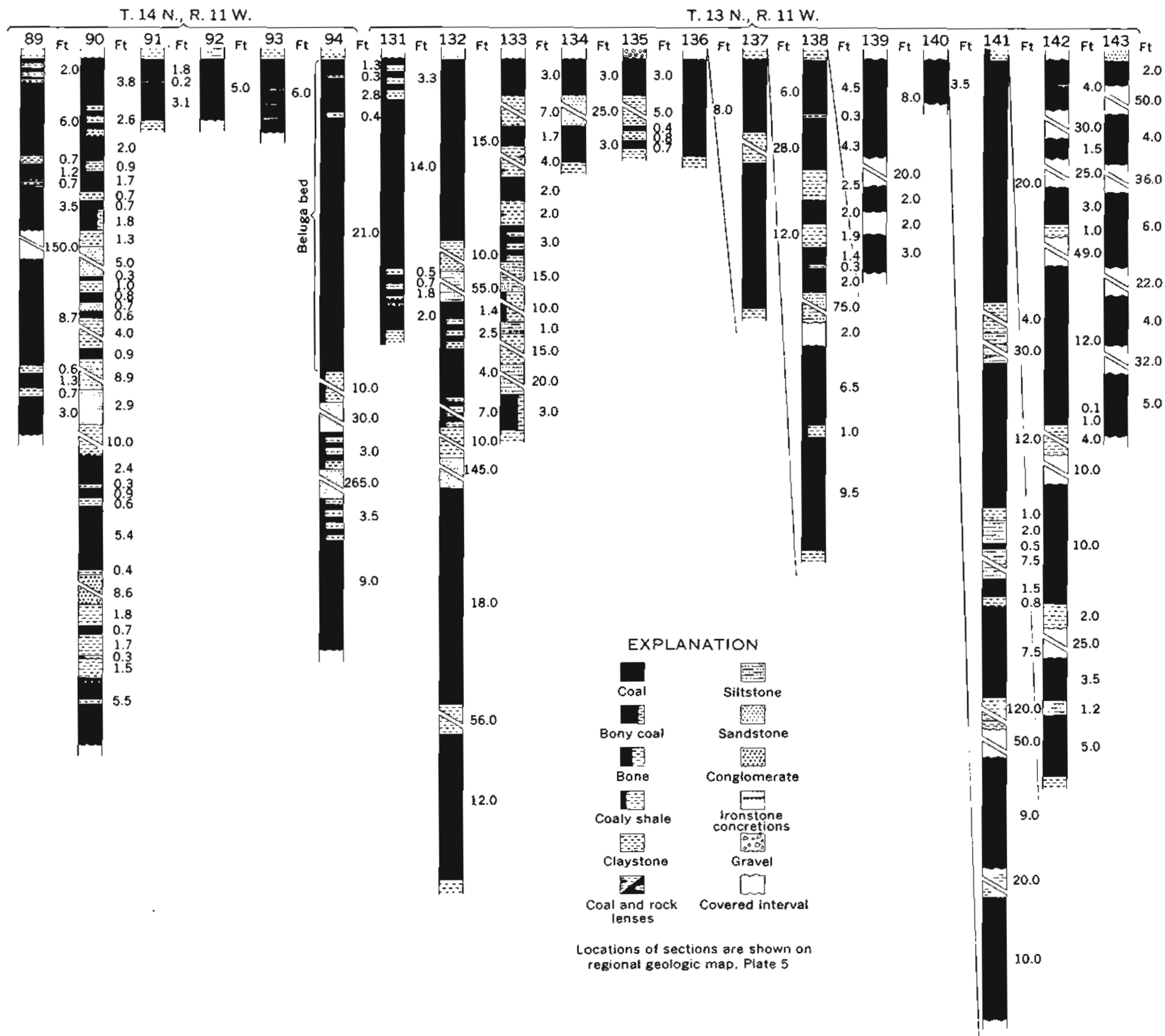
SECTIONS OF COAL BEDS IN BELUGA RIVER AREA, ALASKA
