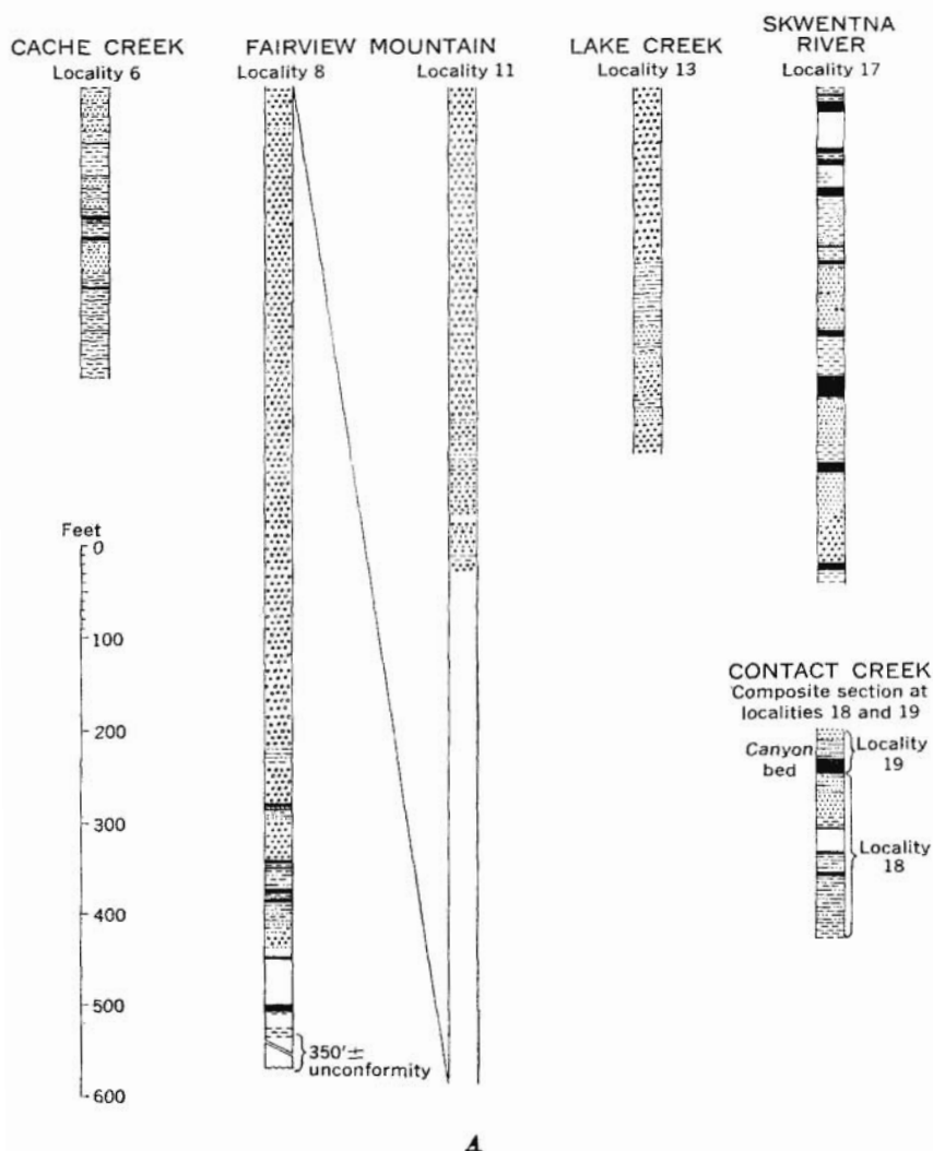
FIGURE 3.—Stratigraphic sections of the Kenai Formation. A , Yentna River basin. B , Beluga River area. Location of sections 6, 13, 17, 56 shown on plate 1; 8, 11 shown on plate 2, Fairview Mountain area; 18, 19 shown on
