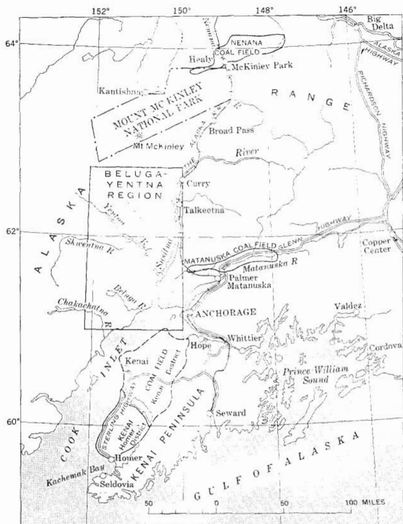
FIGURE 1.—Location of the Beluga-Yentna region and its relation to other coal fields in south-central Alaska.
