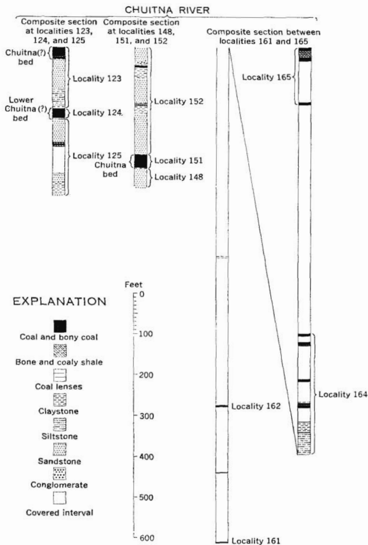
FIGURE 2.—Stratigraphic sections of the Kenai Formation in the Chuitna River and Capps Glacier areas and along the beach southwest of Tyonek. Location
