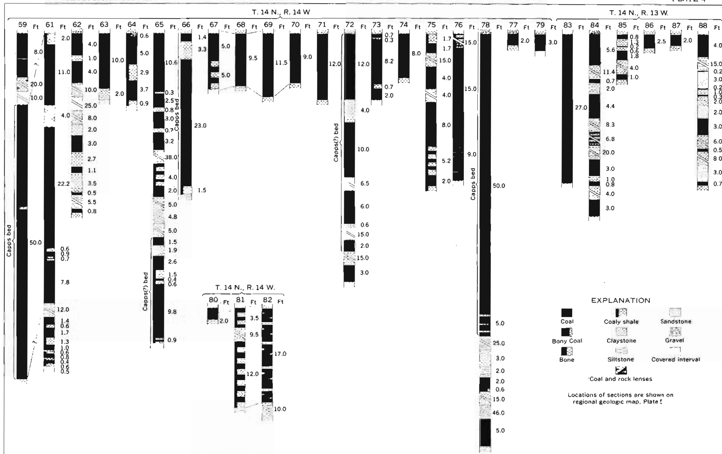
SECTIONS OF COAL BEDS IN CAPPS GLACIER AREA, ALASKA
