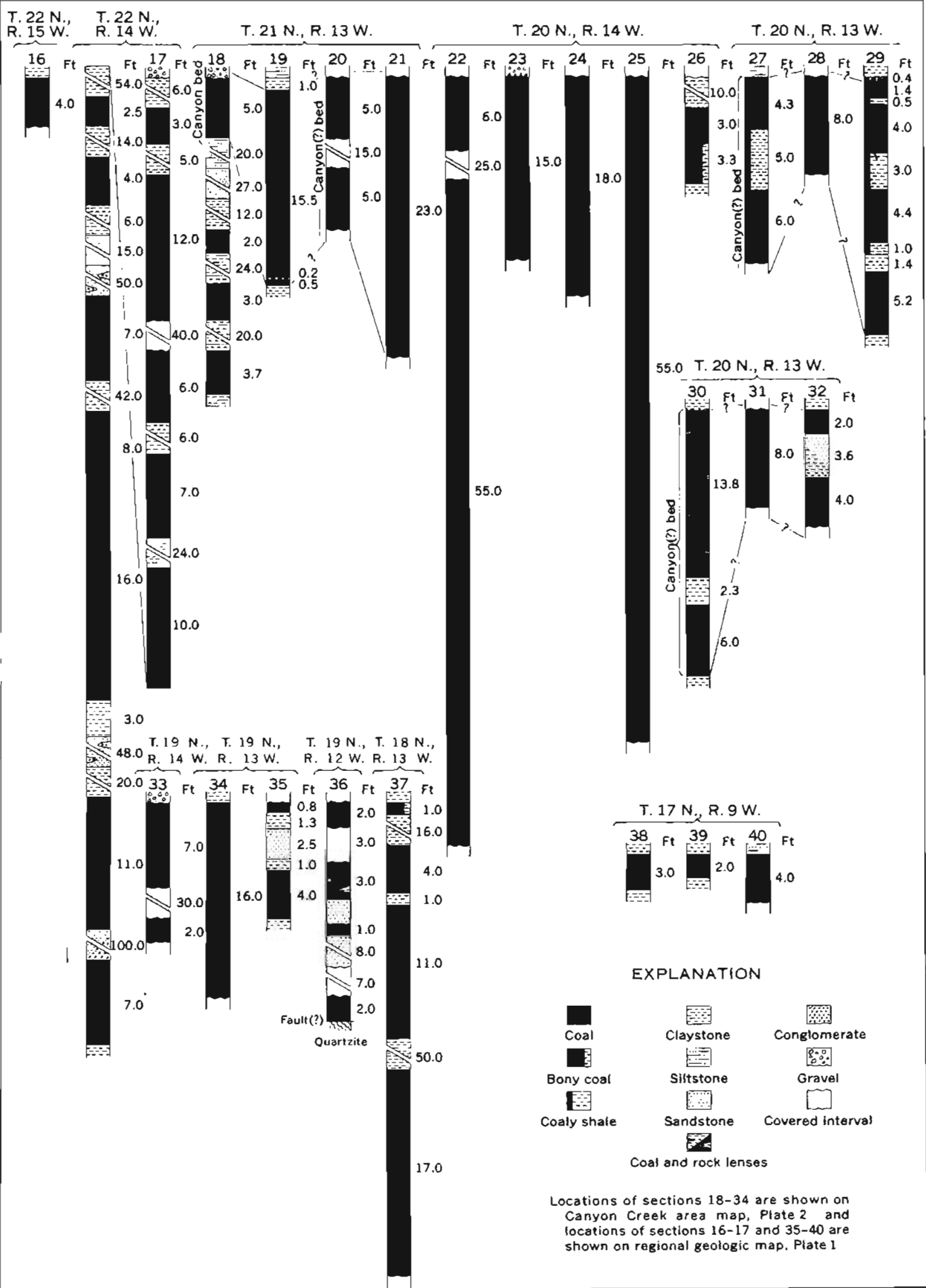
SECTIONS OF COAL BEDS IN CENTRAL PART OF BELUGA-YENTNA REGION, ALASKA
