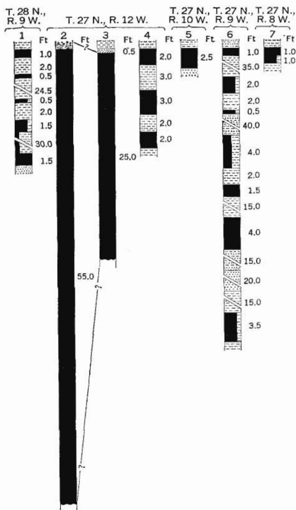
FIGURE 4.—Sections of coal beds in northern part of the Beluga-Yentna region. Locations of sections 1, 5-7, 12 are shown on plate 1; 2-4, 8-10 are on plate 2, Fairview Mountain area; 14-15 are on plate 2, Johnson Creek area.
