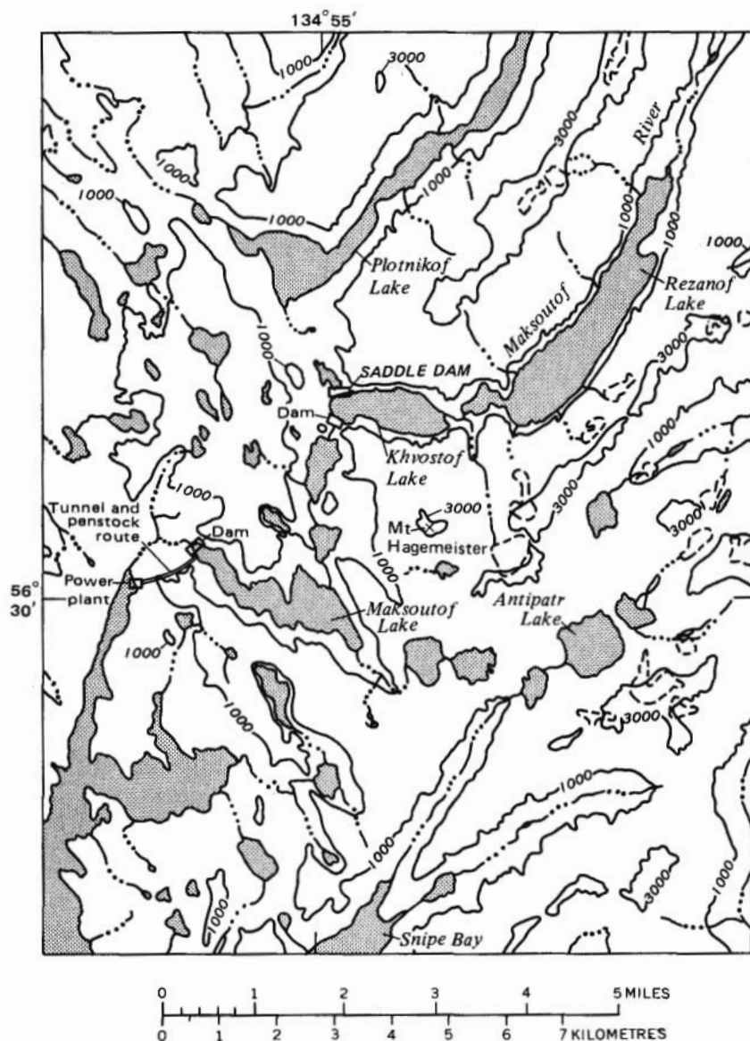
FIGURE 2.—Maksoutof River waterpower development plan.
