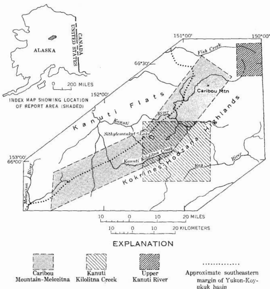
FIGURE 1.—Map of Kanuti River region showing location of areas described in text.
