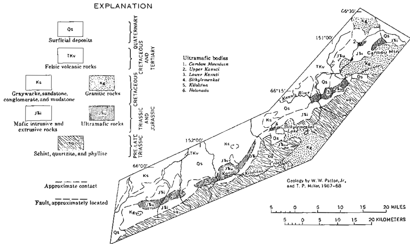
FIGURE 2.—Reconnaissance geologic map of Caribou Mountain-Melozitna ultramafic belt.
