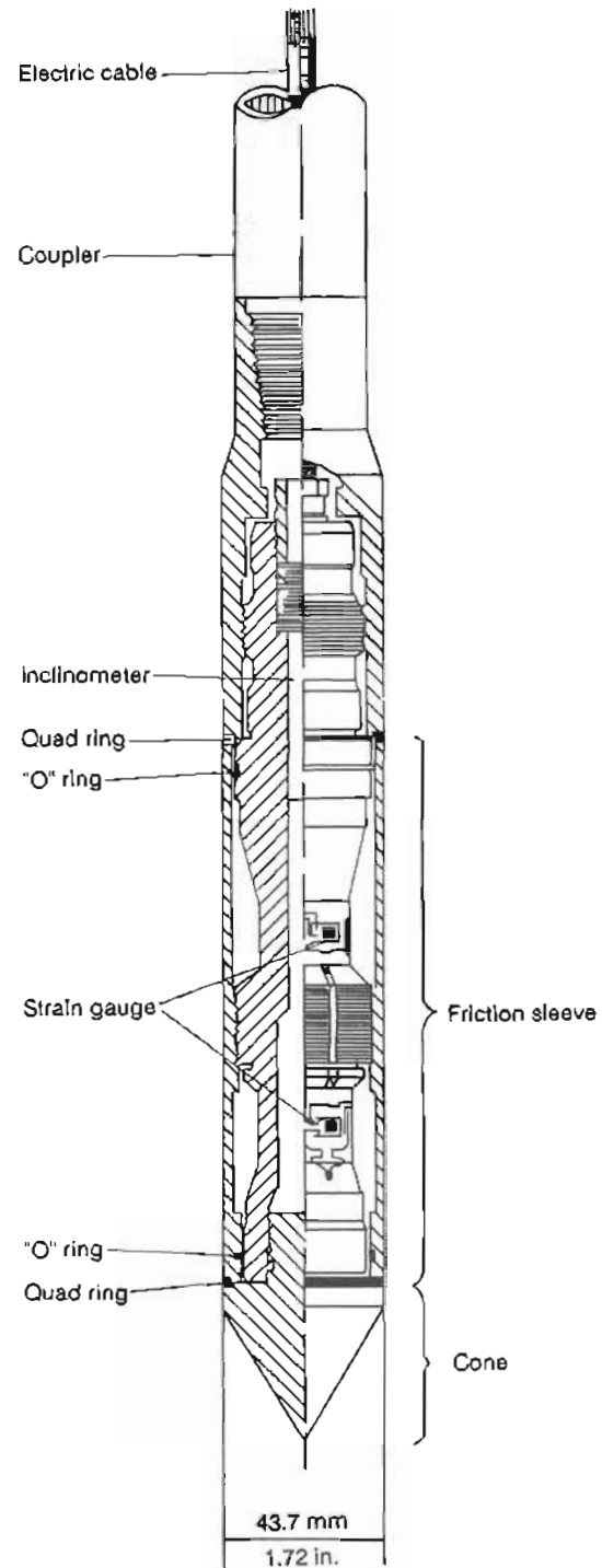
Figure 17. Longitudinal section of electric-cone assembly shown in figures 15 and 16.
