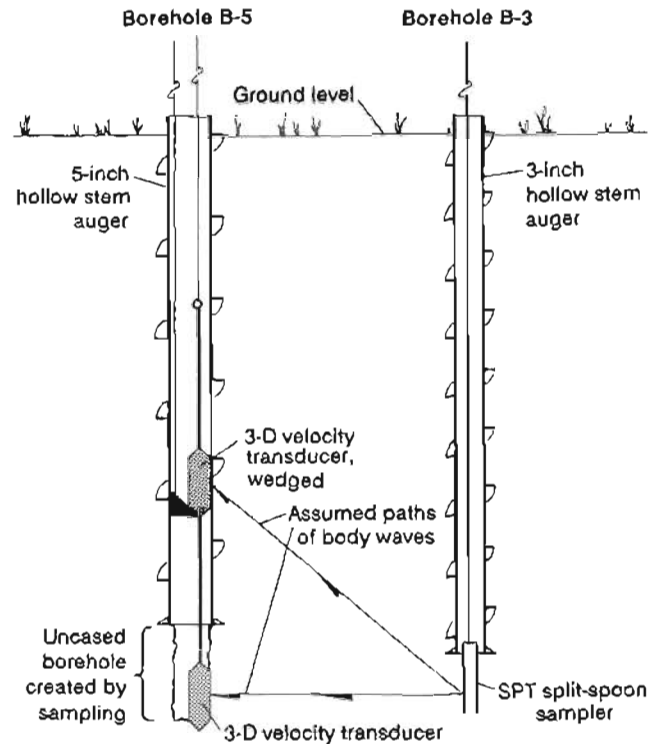
Figure 10. Crosshole configuration used to determine shear-wave velocities in figure 11 (from Hoar and Stokoe, 1980).
