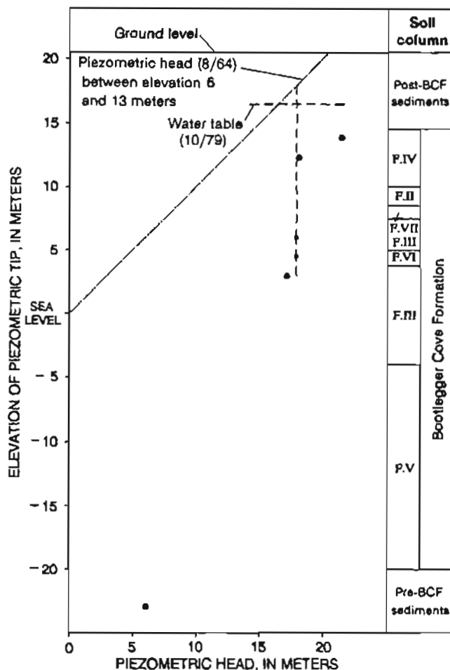
Figure 26. Piezometric head versus depth for piezometers installed in various boreholes behind scarp and in vicinity of Lynn Arty Park after the 1964 earthquake (Shannon and Wilson, 1964). Roman numerals indicate facies of the Bootlegger Cove Formation (BCF) for boreholes B-3 and B-5.
