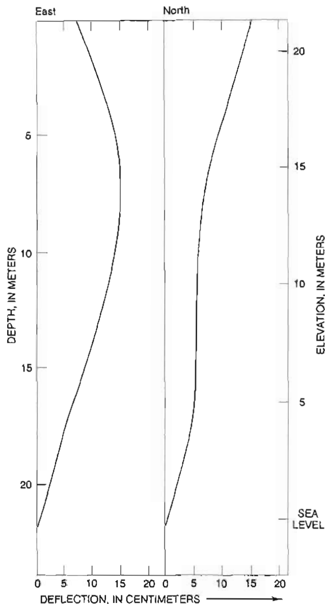
Figure 13. Incliner-casing profiles for borehole B-5 based on 1979 survey. Deflections of casing in east-west plane and north-south plane are shown. An additional survey of the casing in 1981 showed no change in profile.
