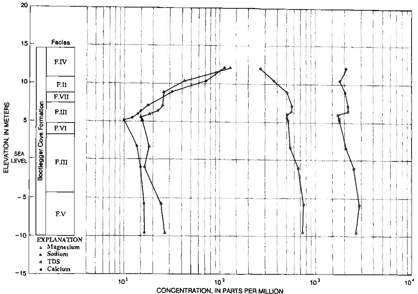
Figure 29. Profiles of pore-fluid cation and total dissolved solids (TDS) concentrations, in relation to the facies (Roman numerals) found in the B-3 and B-5 cores, Lynn Arty Park.
