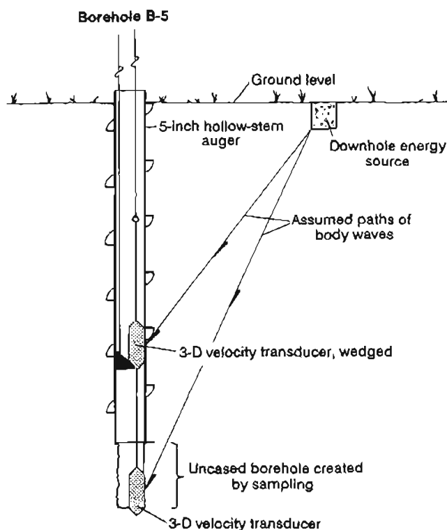
Figure 8. Downhole configuration used to determine shear-wave velocities shown in figure 11 (modified from Hoar and Stokoe, 1980).
