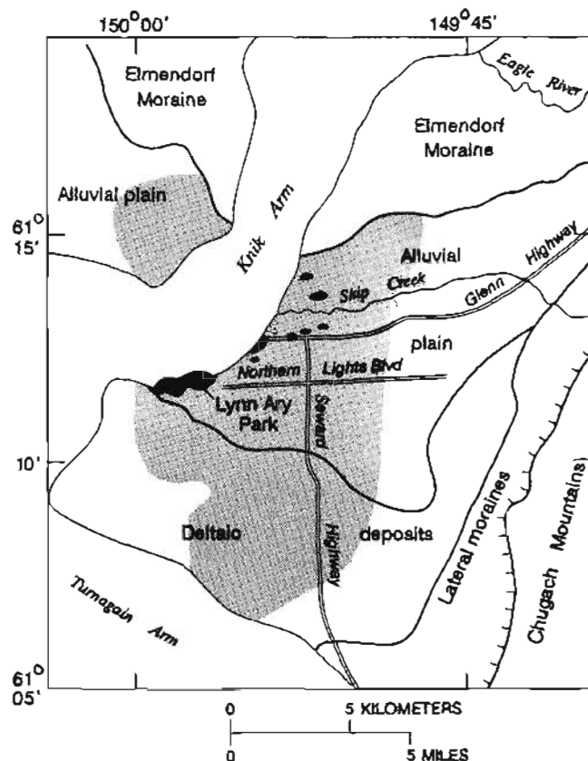
Figure 2. Geologic-physiographic units of the Anchorage lowland and adjacent areas. Bold hachured line indicates eastern boundary of Anchorage lowland; bold solid lines show approximate boundaries between units. Light-shaded area indicates cohesive facies of the Bootlegger Cove Formation, boundaries approximate except for northern extent, which is poorly known. Principal 1964 earthquake-induced landslides shown in dark shade. Map also shows location of Lynn Arty Park (approximately the area of fig. 3) and of other cultural features mentioned in text.
