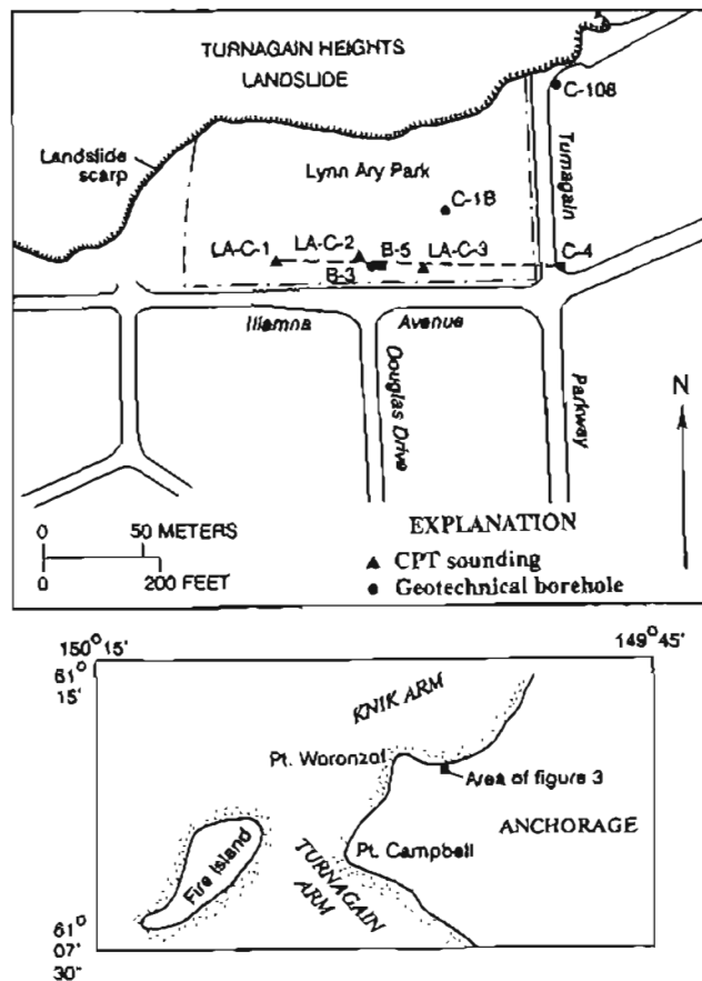
Figure 3. Location of geotechnical boreholes and cone-penetrometer test (CPT) soundings, vicinity of Lynn Arty Park. Boreholes B-3 and B-5 were made as part of this study; C-4, C-108, and C-1B were made shortly after the 1964 earthquake (Shannon and Wilson, 1964). Dashed line, position of cross section, plate 5. Landslide scarp (hachured line) is shown in approximately its original configuration.
