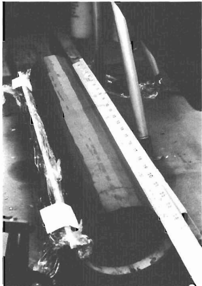
Figure 6. Photograph of 12.7-cm- (5-in.-) diameter core from the Bootlegger Cove Formation. Surface has been trimmed to reveal texture and structures.
