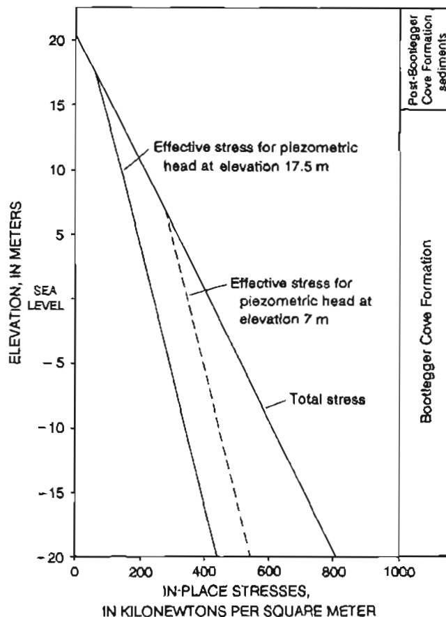
Figure 27. Total and effective-stress profiles at Lynn Arty Park, based on density data given on plates 1 and 2 and on pore-pressure data given in figure 26.
