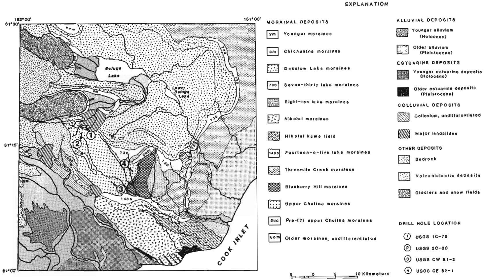
Figure 2. Generalized surficial geologic map of the Beluga plateau and vicinity, upper Cook Inlet region, Alaska.
