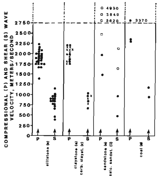
Figure 12. Distribution of ultrasonic compressional- and shear-wave velocity values for Chuitna coal field (USGS CW 81-2 and CE 82-1) core samples.
