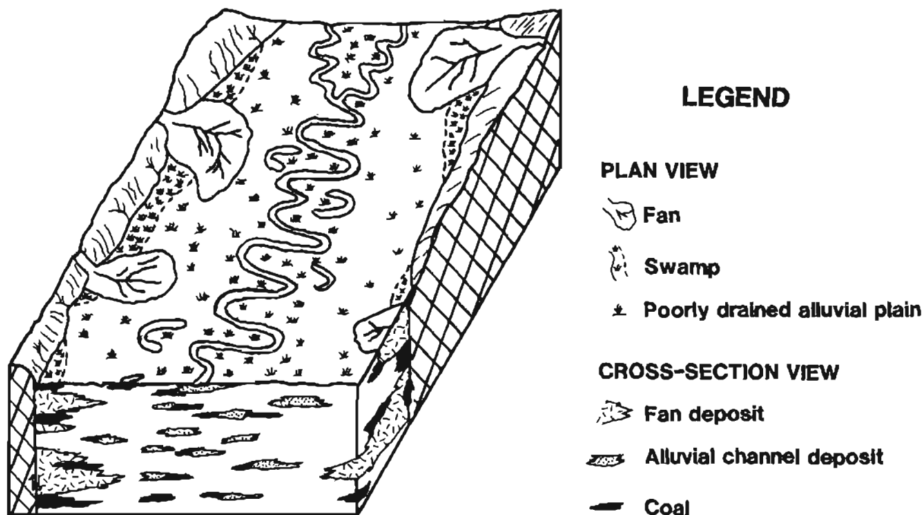
Figure 3. Depositional environment model of the Tyonek Formation showing a poorly drained alluvial basin (Hite, 1976).
