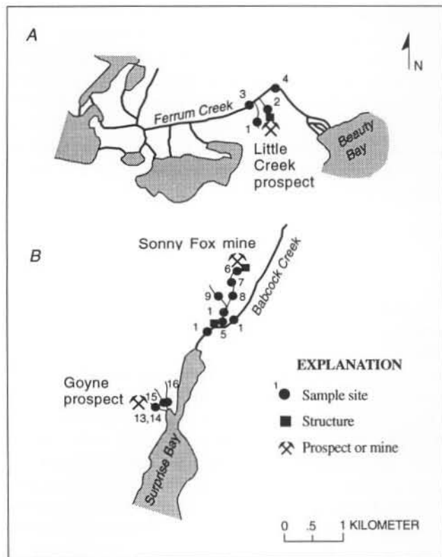
Figure 2. Location of stream-water sample sites near (A) Little Creek prospect and (B) Sonny Fox mine and Goyne prospect.
