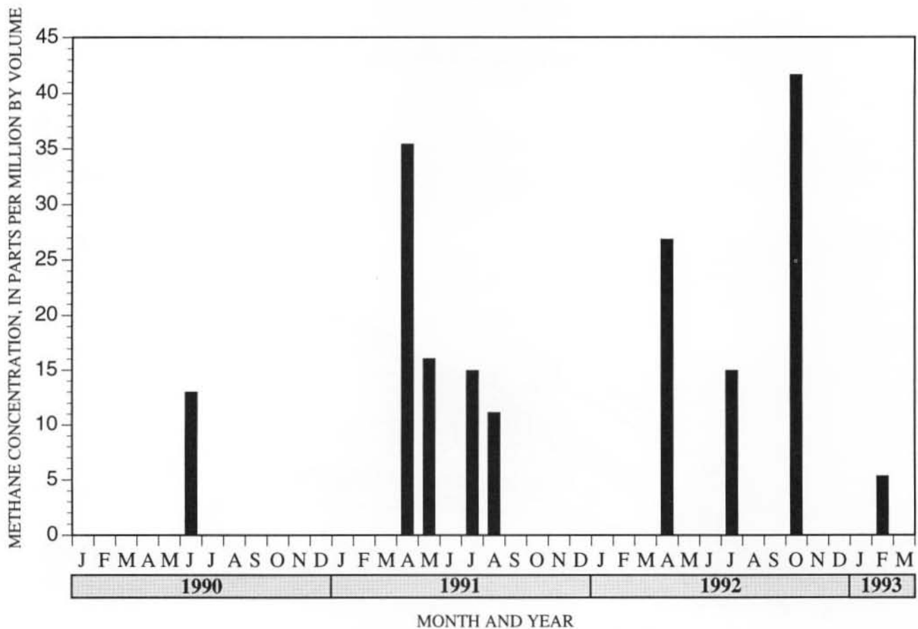
Figure 3. Average methane concentrations (ppmv) measured 9 times at 5 to 10 stations during 1990–1993 in the air of the Fox permafrost tunnel.
