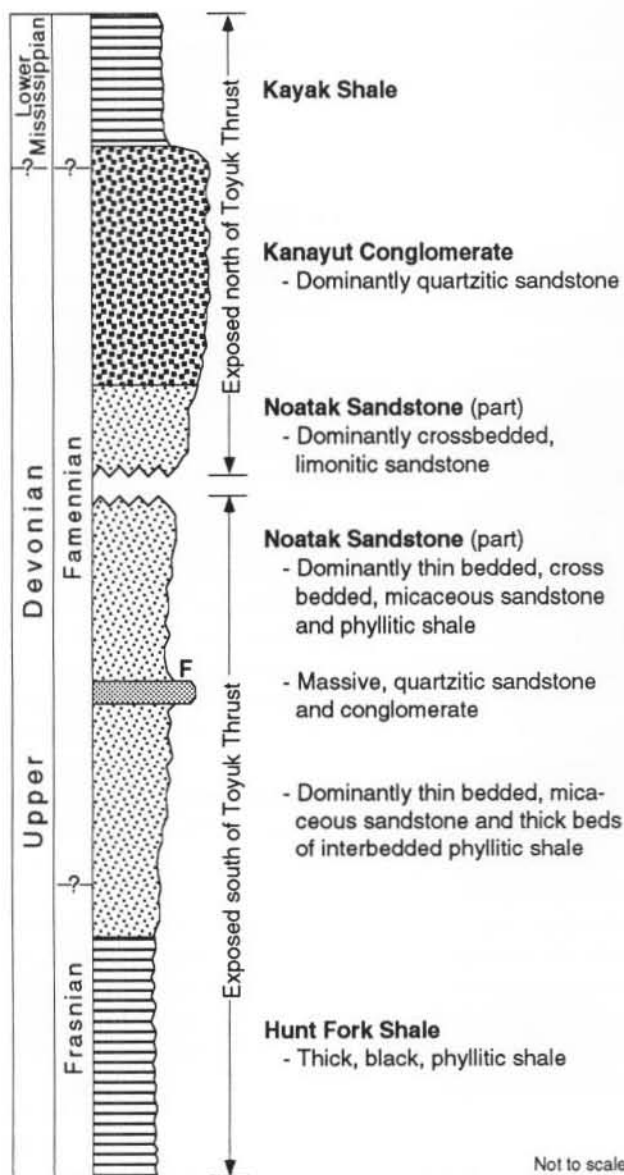
Figure 2. Generalized stratigraphic column of the Endicott Group in Ivotuk Creek area. F, approximate level of fossil collections.
