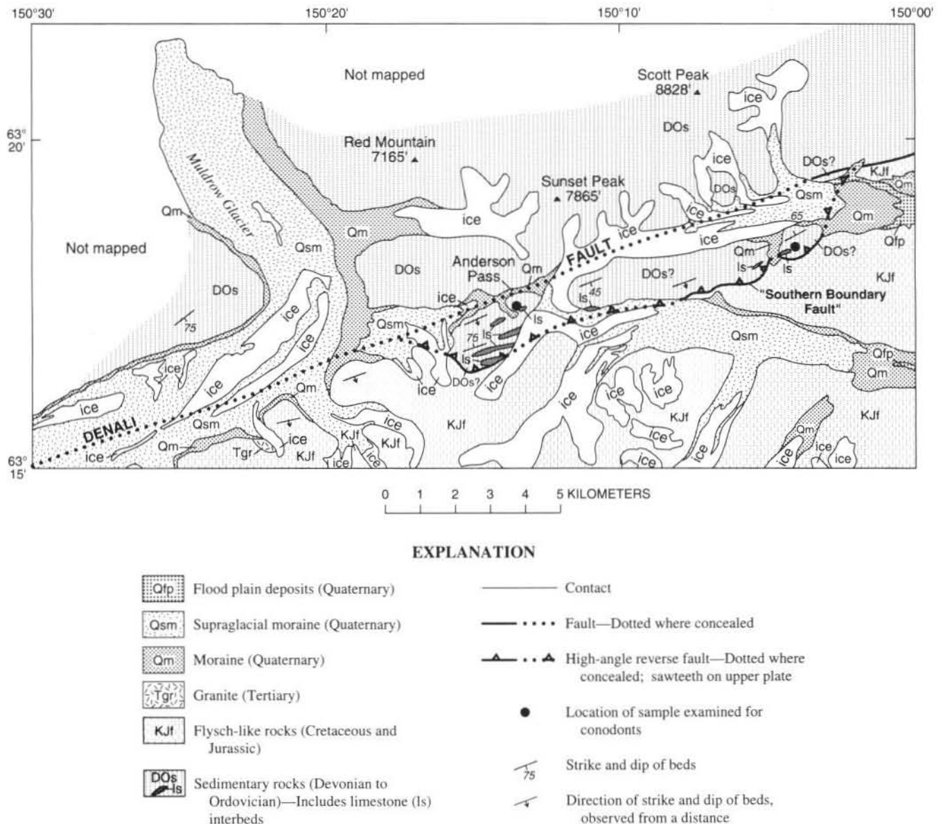
Figure 1. Generalized geologic map of Anderson Pass area of central Alaska Range, Denali National Park, Alaska.
