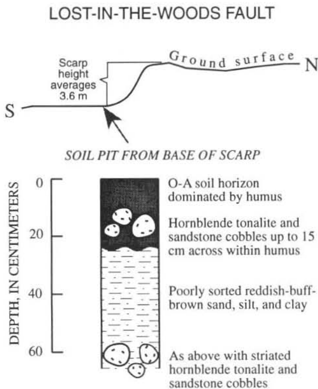
Figure 6. Profile of scarp and soil pit stratigraphy at Lost-in-the-woods fault.
