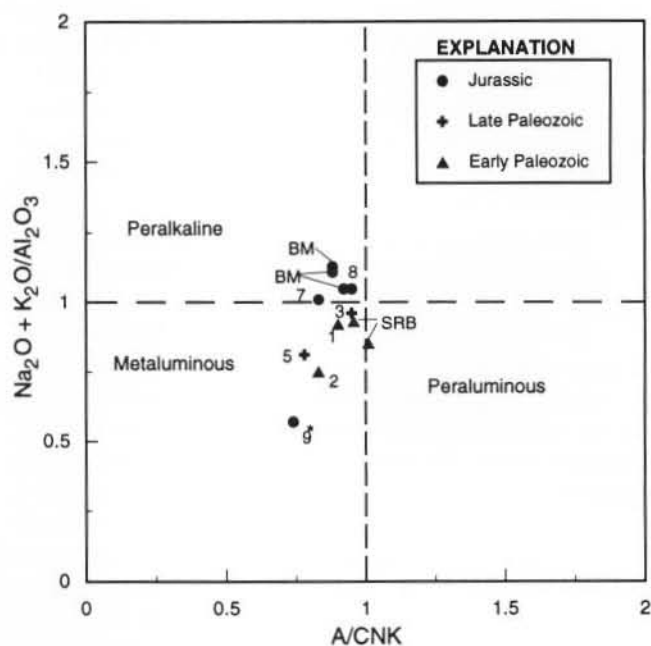
Figure 3. Plot of (Na 2 O+K 2 O)/Al 2 O 3 vs. A/CNK (molecular ratio of Al 2 O 3 /[CaO+Na 2 O+K 2 O]) for alkalic rocks from Prince of Wales Island; field boundary from Shand (1951). See figure 1 for location of sample numbers. Data for Bokan Mountain Granite (BM) and Stone Rock Bay pluton (SRB) from MacKevett (1963).
