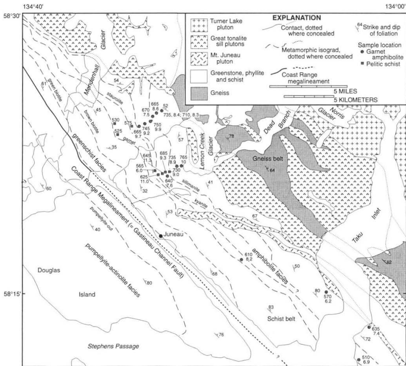
Figure 3. Geologic map of Juneau area, southeastern Alaska (parts of A1, A2, B1, and B2 quadrangles), showing distribution of metamorphic facies, metamorphic isograds, and calculated temperatures ( ^{\circ}\text{C} ) and pressures (kbar). Schist belt unpatterned for
