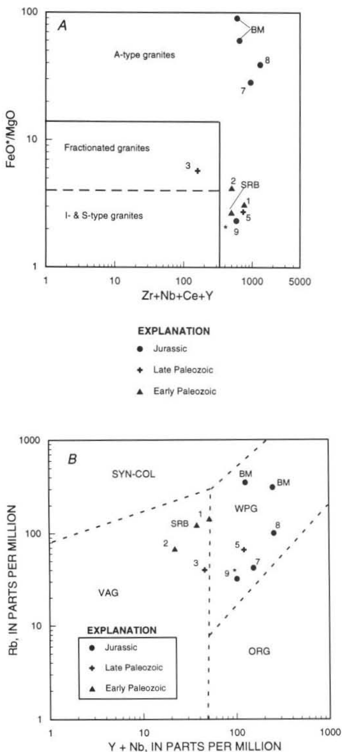
Figure 7. Trace element classification diagrams of alkalic plutons on Prince of Wales Island. A , Petrologic affinity classification. B , Tectonic classification: VAG, volcanic-arc granitoids; ORG, oceanic-ridge granitoids; WPG, within-plate granitoids; SRB, Stone Rock Bay pluton. SYN-COL, syn-collision or late tectonic granitoids. Field boundaries for A and B from Whalen and others (1987) and Pearce and others (1984), respectively. Bokan Mountain Granite (BM) data from Thompson and others (1982).
