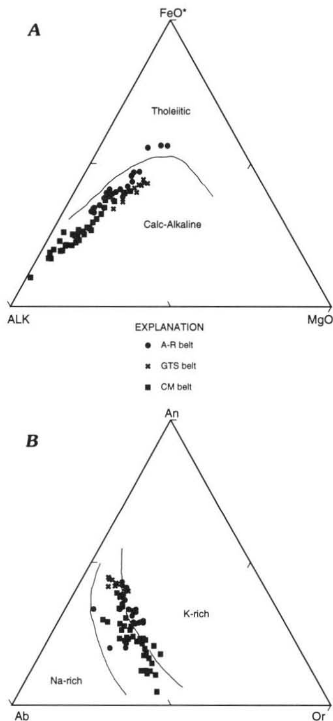
Figure 7. Ternary diagrams for plutonic rocks from three major plutonic belts of the Taku Inlet transect. A-R, Admiralty-Revillagigedo belt; GTS, Great tonalite sill belt; CM, Coast Mountains belt. A, AFM diagram with boundary line from Irvine and Baragar (1971). \text{FeO}^* , \text{FeO} + (.8998 \times \text{Fe}_2\text{O}_3) ; Alk, \text{Na}_2\text{O} + \text{K}_2\text{O} . B, Normative feldspar composition diagram with boundary lines from Irvine and Baragar (1971). An, anorthite percent; Ab, albite percent; Or, orthoclase percent.
