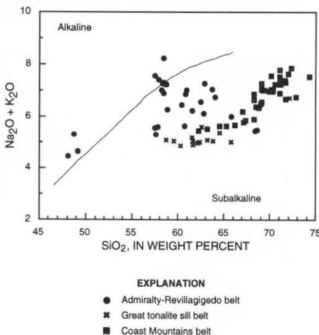
Figure 5. Variation diagram of SiO 2 versus total alkalis (Na 2 O+K 2 O) for plutonic rocks from three major plutonic belts of the Taku Inlet transect. Field boundary from Irvine and Baragar (1971).
