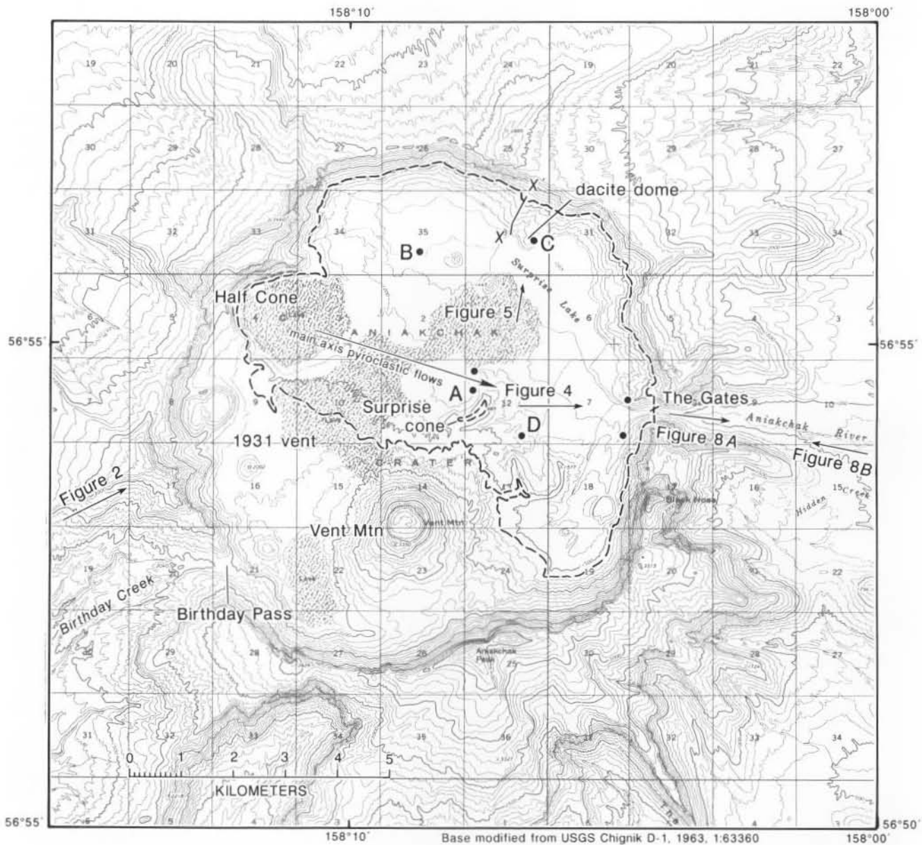
Figure 3. Topographic map of Aniakchak Crater. Large arrow shows main emplacement direction of pyroclastic-flow deposits produced during explosive destruction of Half Cone. Line X-X' marks location of traverse across wave-cut terraces on north caldera wall. Small arrows show direction of view in other figures. Solid circles are locations of lake sediments discussed in text, and points A-C mark specific outcrops referred to in text. Point D is location for
