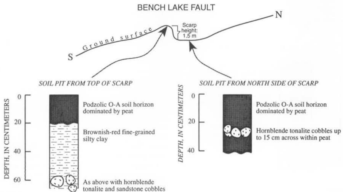
Figure 5. Profile of scarp and soil pit stratigraphy at Bench Lake fault.
