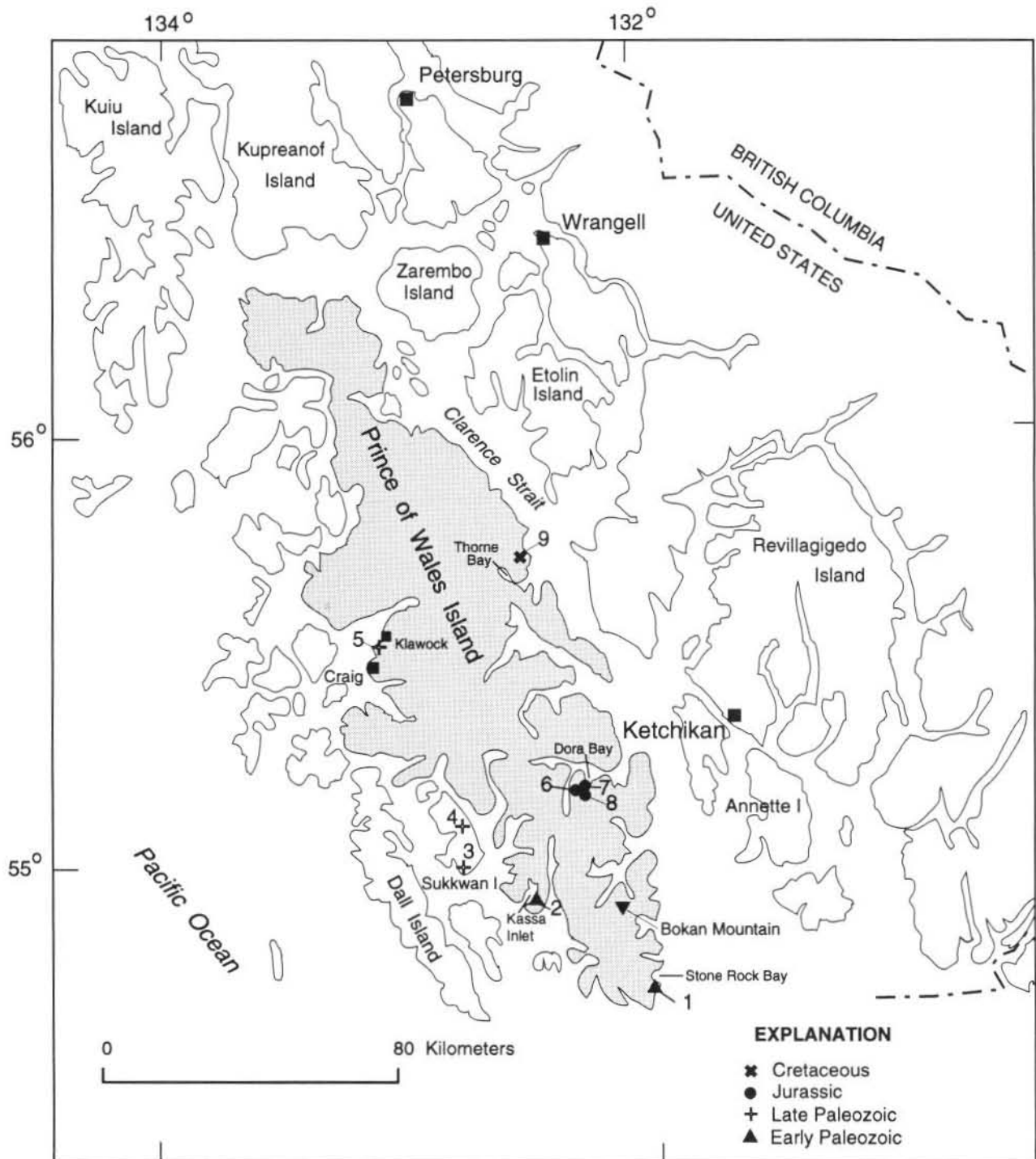
Figure 1. Index map of Prince of Wales Island showing sample locations from alkalic plutons described in this report. Numbers correspond to samples listed in tables 1 and 2.
