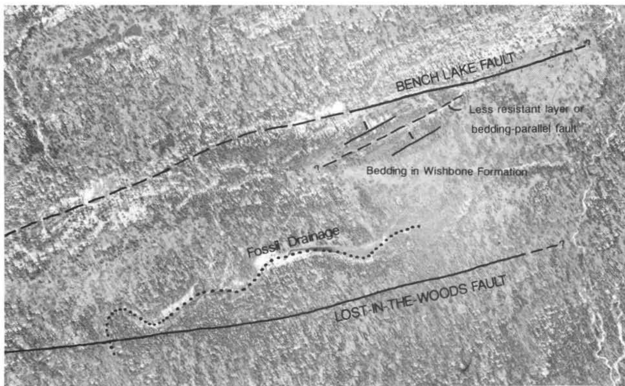
Figure 3. A , Uninterpreted vertical aerial photograph in the vicinity of Bench Lake and Lost-in-the-woods faults. B , Same aerial photograph showing interpreted locations of Bench Lake and Lost-in-the-woods faults, and bedding orientation in conglomerate of the Wishbone Formation.
