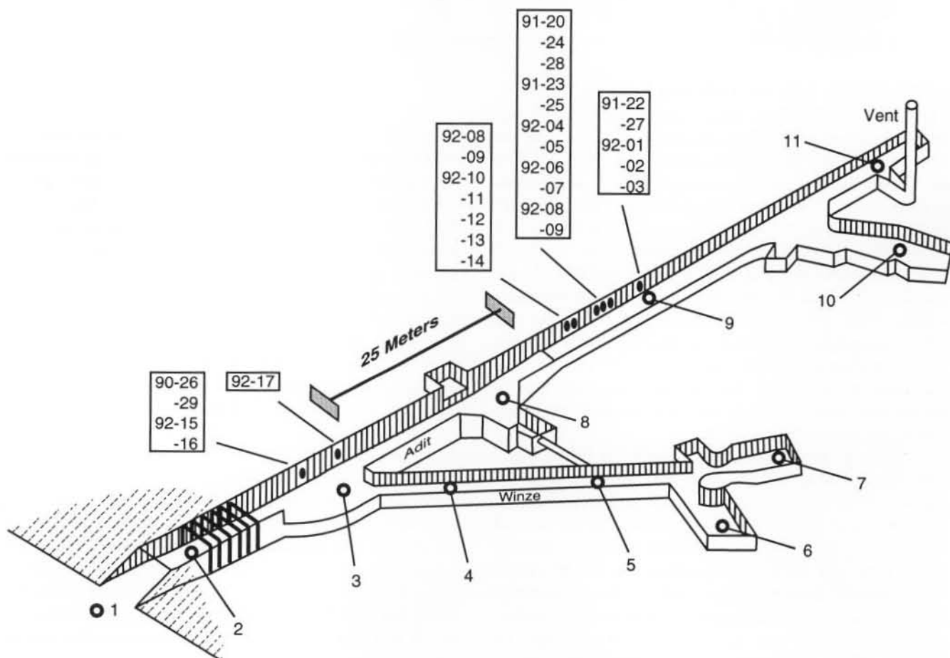
Figure 2. Isometric view of the Fox permafrost tunnel showing sites where air samples (open circles) and permafrost cores (solid circles) were collected for methane analysis. Adit and winze are 110-m and 61-m long, respectively. Numbers in boxes refer to
