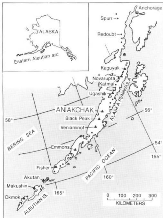
Figure 1. Location of Aniakchak caldera and other major Holocene volcanoes of the eastern Aleutian arc. Triangles denote calderas and circles denote stratovolcanoes. From Miller and Smith, 1987.
