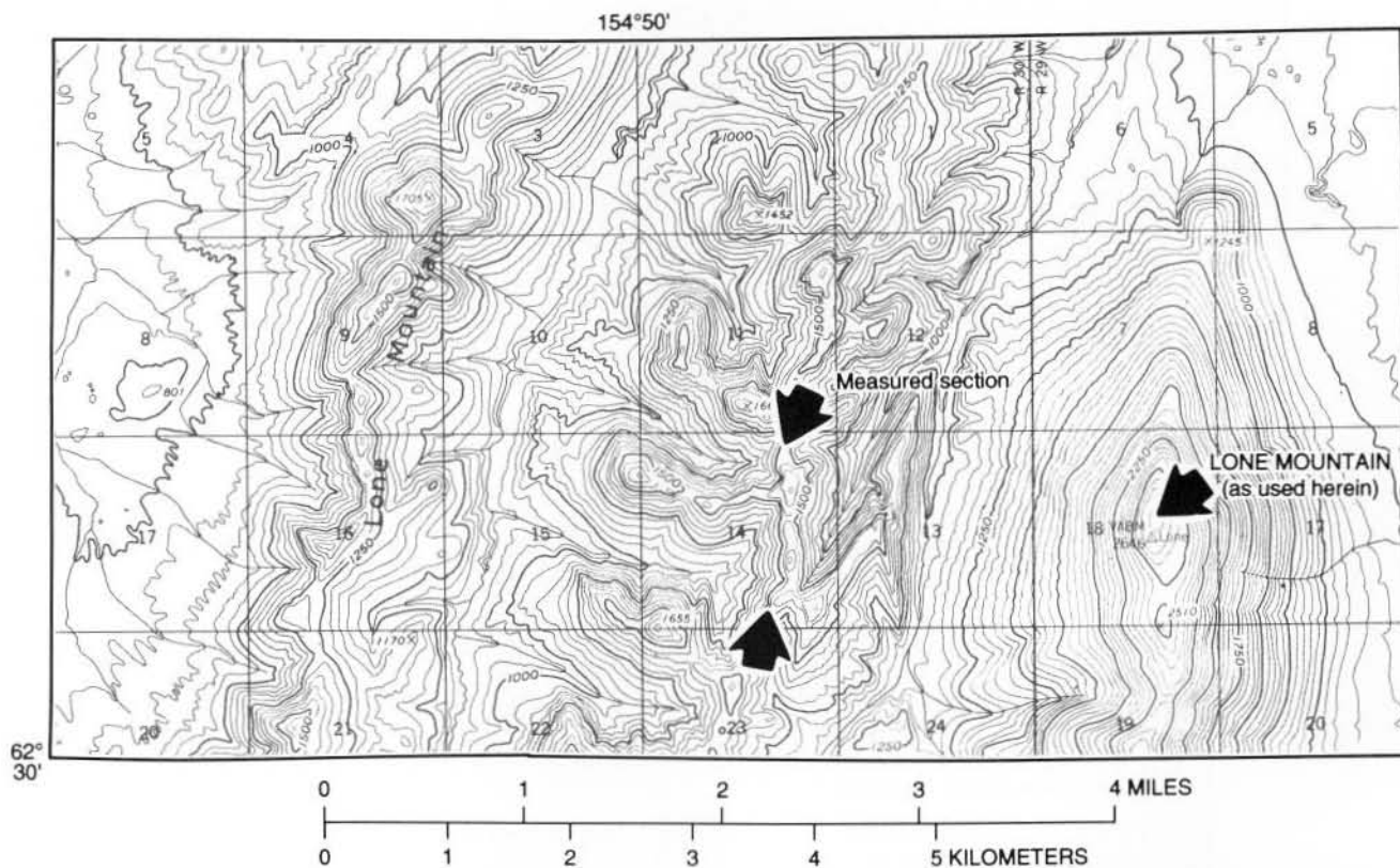
Figure 2. Topographic map showing current and corrected usage of Lone Mountain, as well as location of measured section discussed in text. Map includes part of T. 28 N. from the McGrath C-4 1:63:360 topographic quadrangle (U.S. Geological Survey, 1953). On the map, Lone Mountain is identified by uppercase and lowercase lettering as a low ridge principally through sec-
