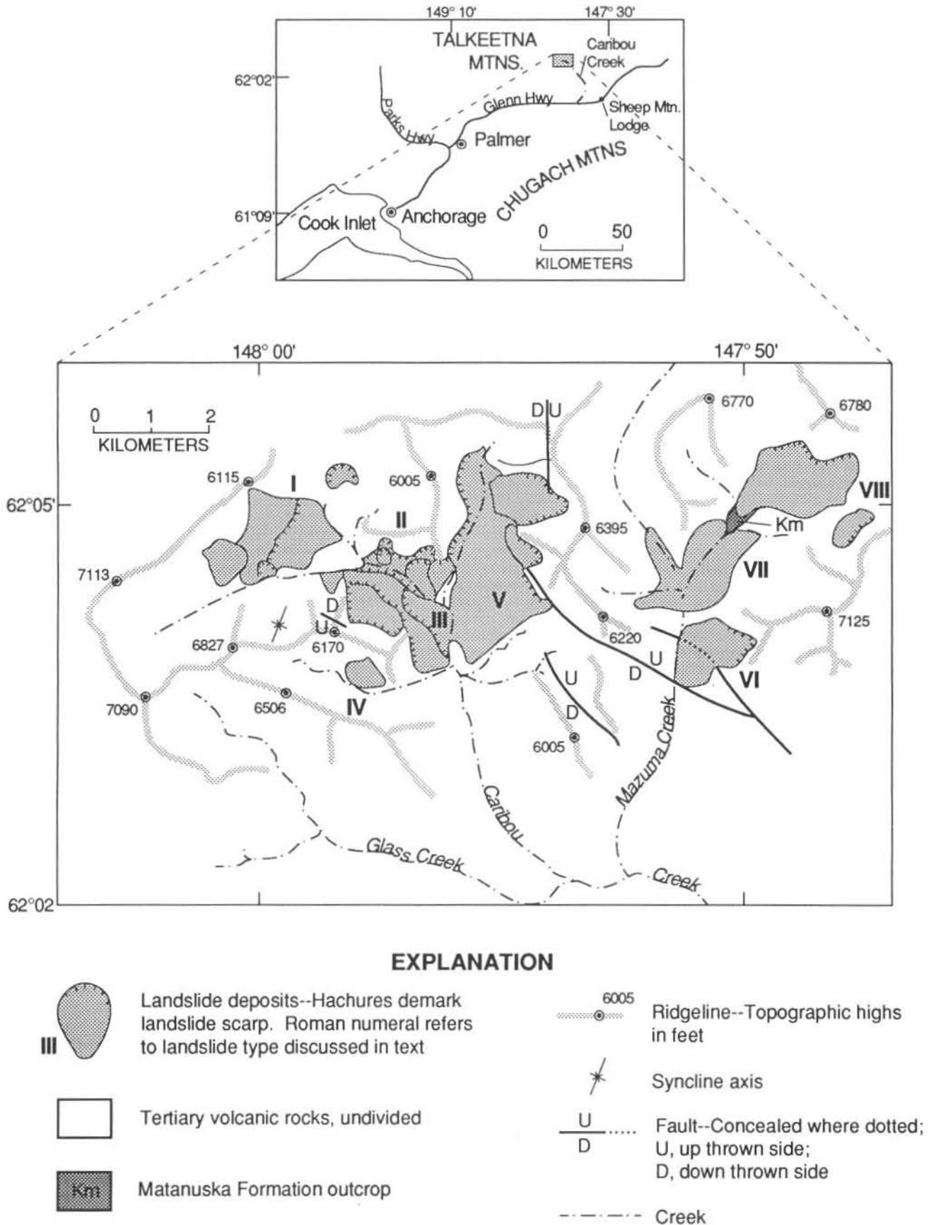
Figure 1. Caribou Creek area, landslides, and other geologic features.
