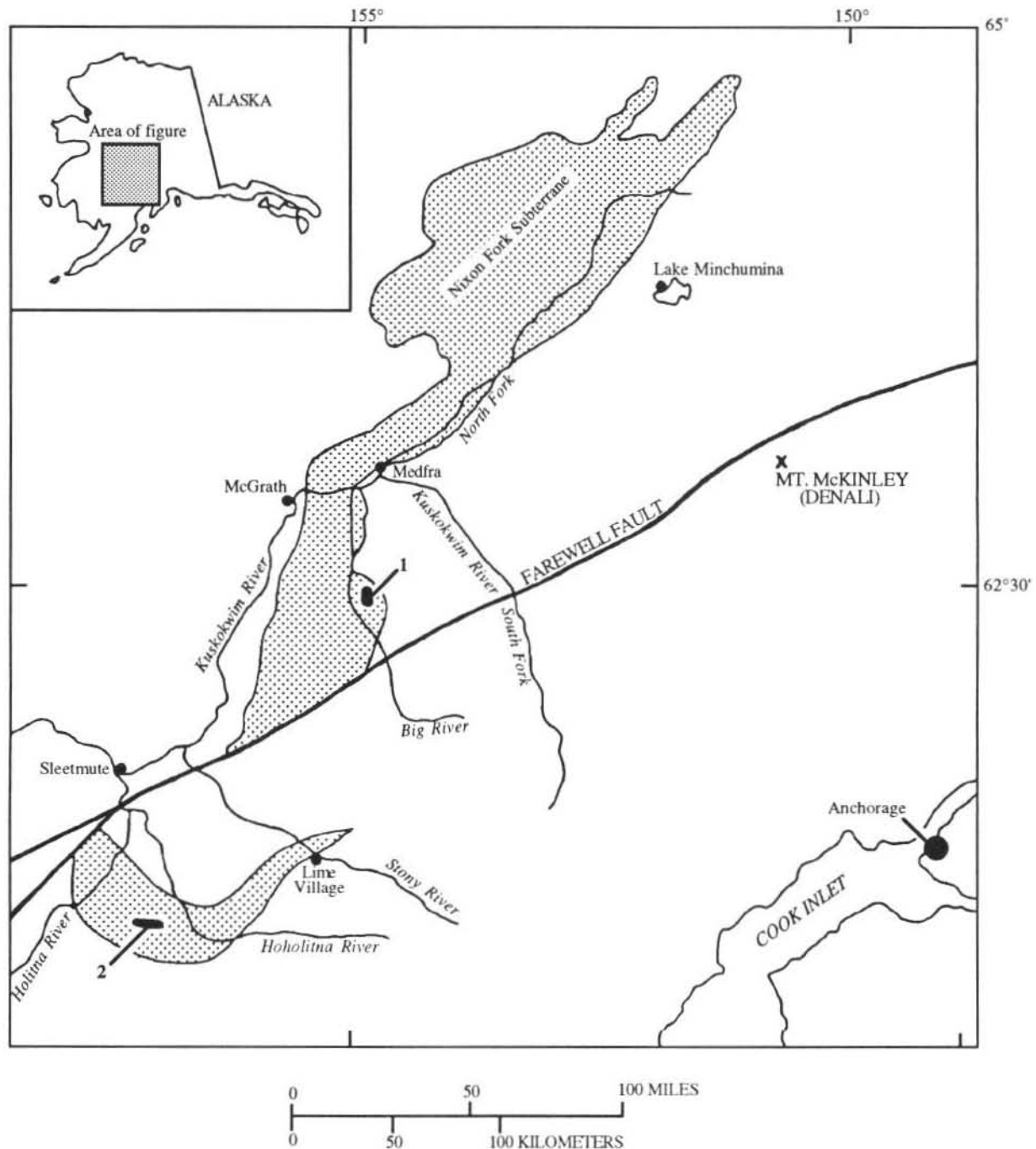
Figure 1. Index map of part of west-central and southwestern Alaska showing location of Nixon Fork subterrane of the Farewell terrane (stippled areas); modified from Blodgett and Gilbert (1992a). Map symbols: 1, area of Pro-
