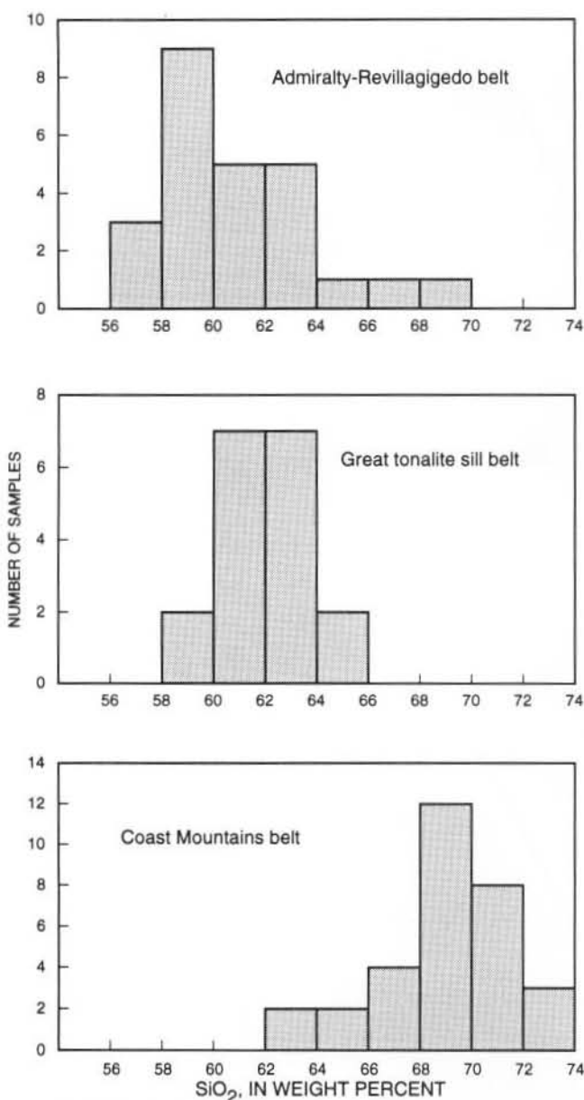
Figure 3. Distribution of SiO 2 content in plutonic rocks from three major plutonic belts of the Taku Inlet transect.
