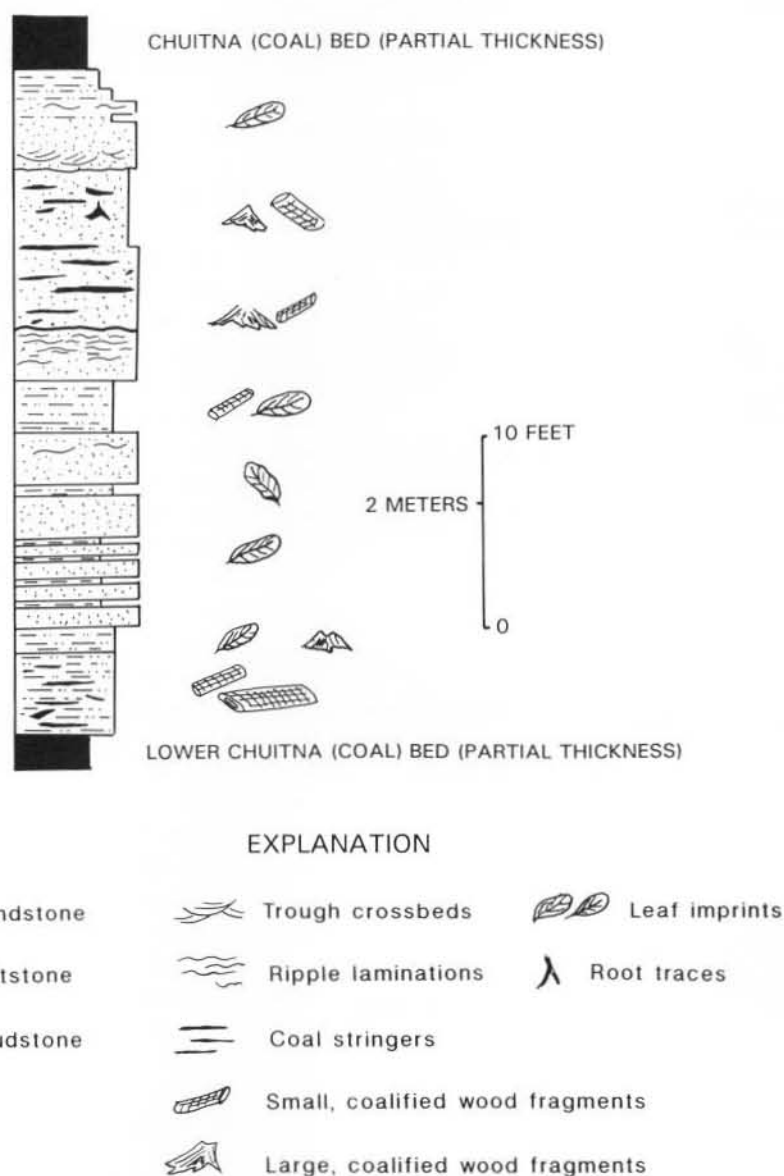
Figure 14. Facies profile proximal to informally named Lower Chuitna conglomeratic sandstone bed and adopted from measured section 16 (see fig. 2 for location) of Adkison and others (1975).
