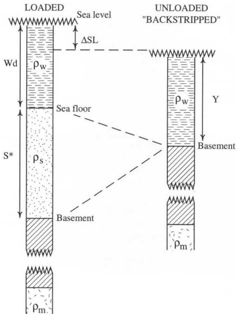
Figure 4. Schematic diagram of a reconstructed (loaded) sedimentary column and a backstripped (unloaded) column. S^* , delithified sedimentary thickness; Wd , water depth; \Delta SL , change in sea level; Y , depth to basement in the absence of sedimentary load; \rho_w , density of water; \rho_s , density of sediment; \rho_m , density of mantle. From Steckler and Watts (1978).
