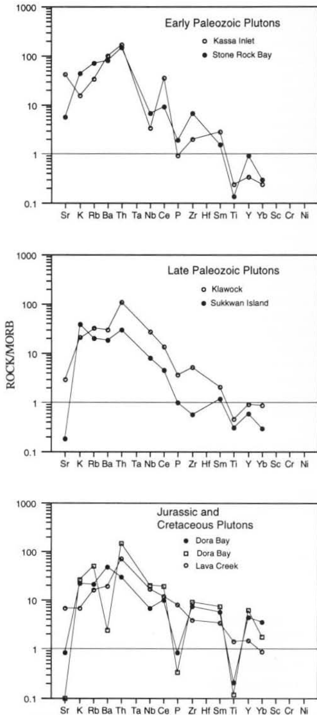
Figure 5. Mid-ocean ridge basalt (MORB) normalized multi-element diagrams (spidergrams) for alkalic plutons on Prince of Wales Island; MORB values from Pearce (1983).
