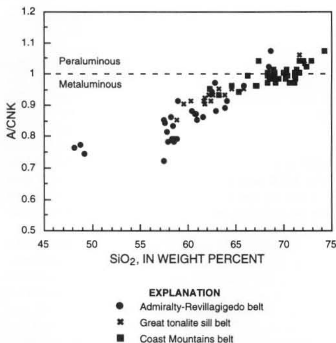
Figure 4. Variation diagram of SiO 2 versus A/CNK (molecular proportions Al 2 O 3 /CaO+Na 2 O+K 2 O) for granitoids from three major plutonic belts of the Taku Inlet transect.
