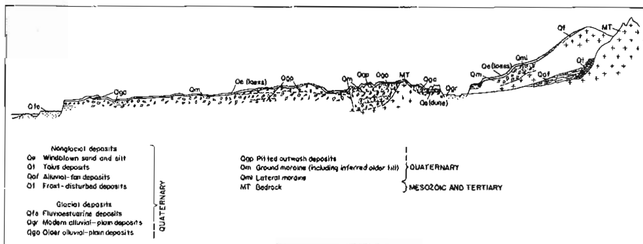
Figure 3. Generalized section of the Matanuska Valley agricultural area showing stratigraphic units.
