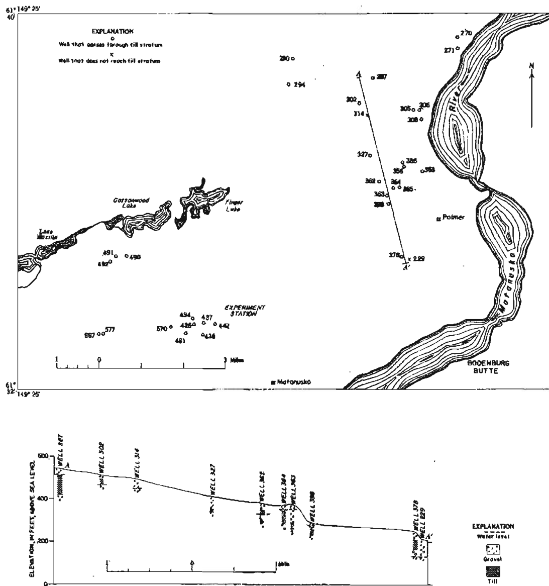
Figure 5. Map and section showing distribution of older glacial deposits known from well logs.
