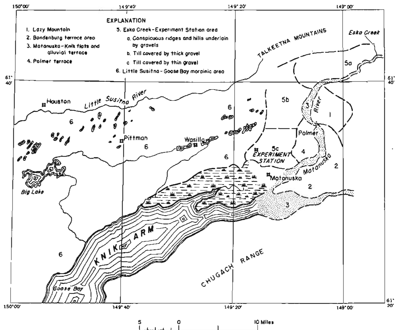
Figure 2. Physiographic units in the Matanuska Valley agricultural area.
