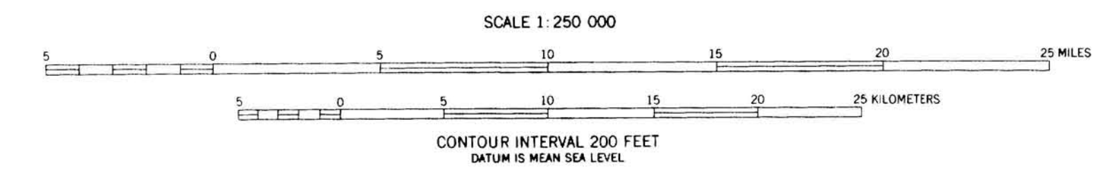
METALLIC MINERAL RESOURCES MAP OF THE CHANDALAR QUADRANGLE, ALASKA Compiled by Edward H. Cobb, 1972
