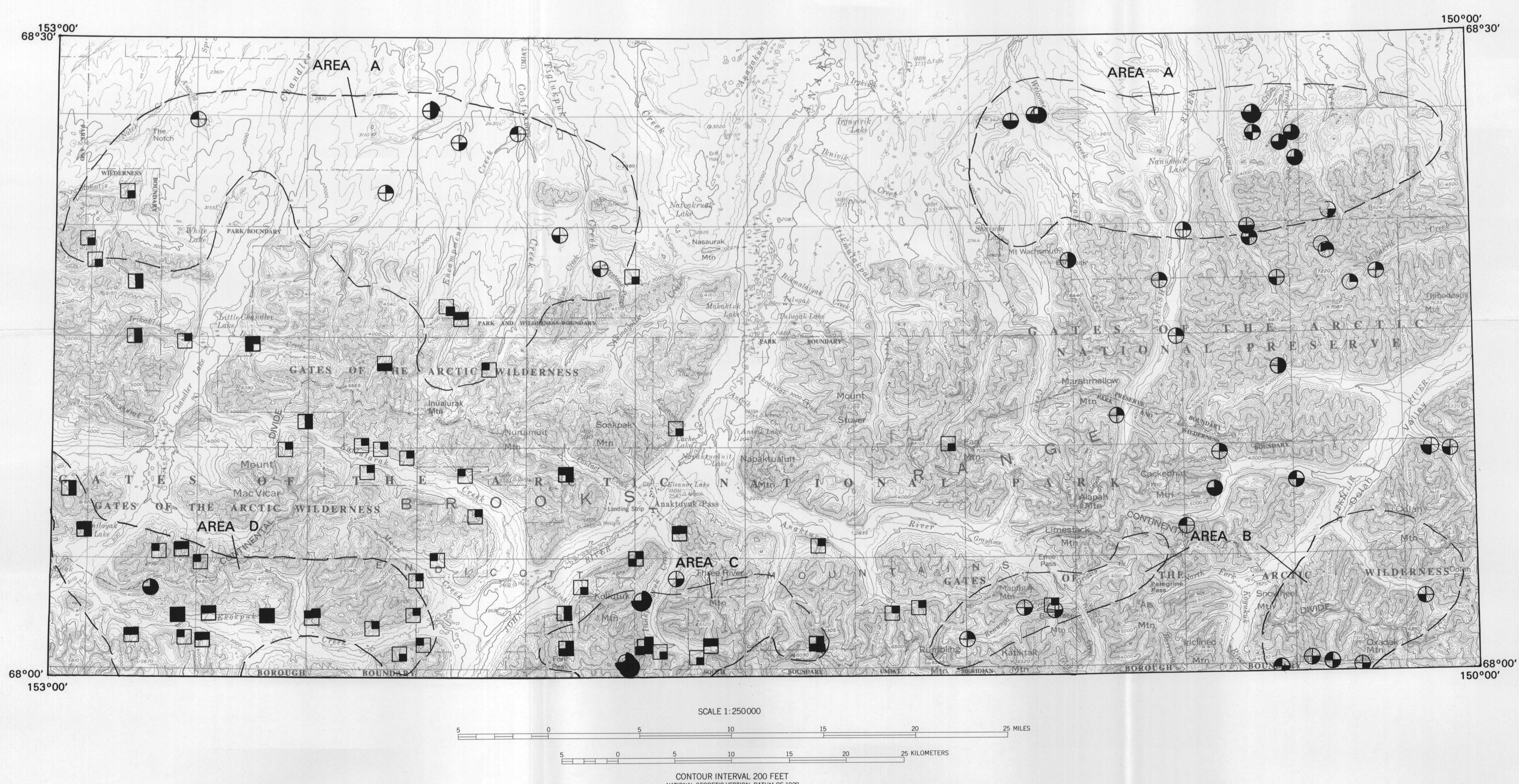
MAP D. DISTRIBUTION OF ARSENIC, COBALT, CHROMIUM, AND NICKEL IN MINUS-30- AND MINUS-80-MESH STREAM-SEDIMENT SAMPLES
