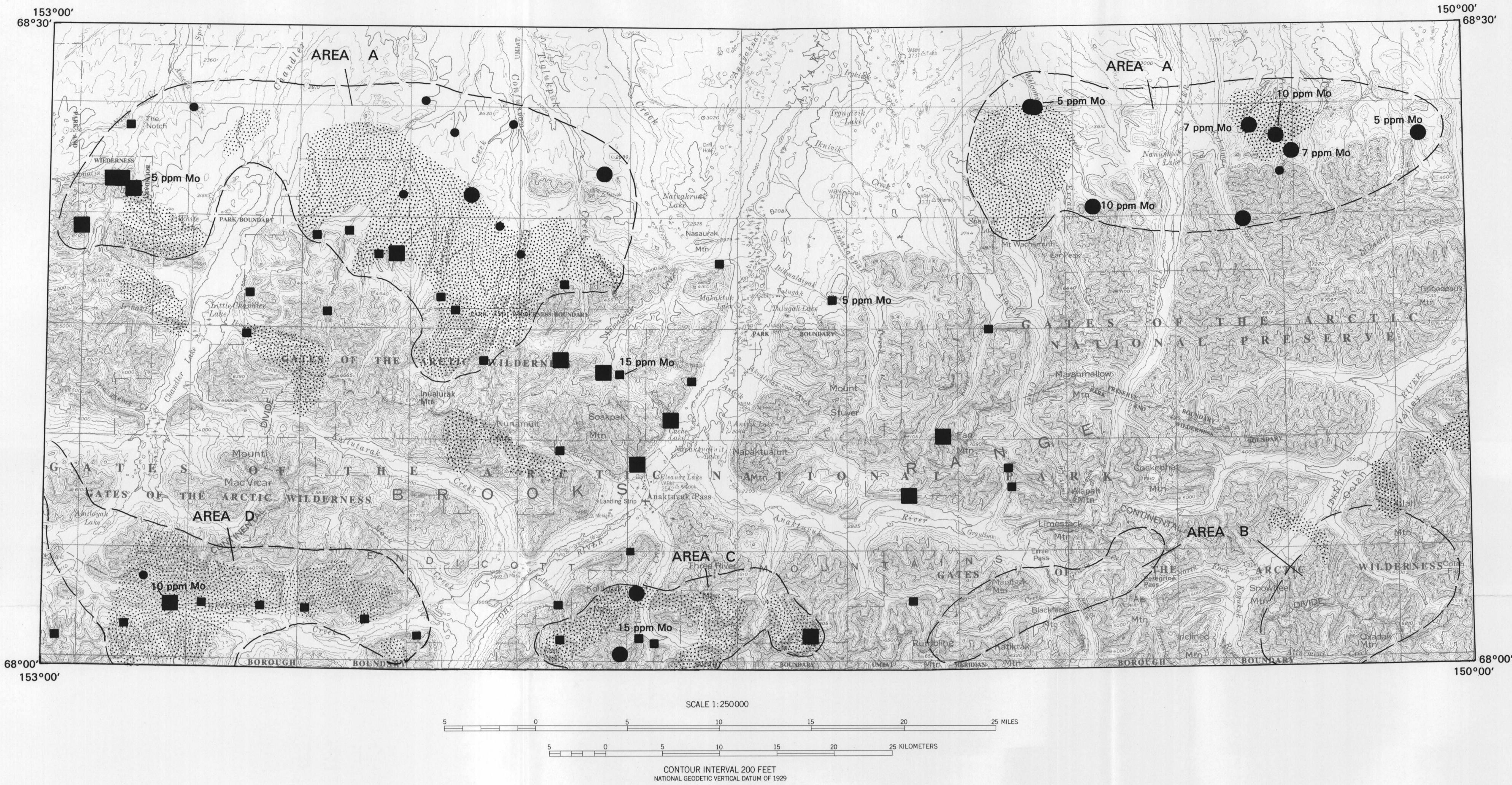
MAP B. DISTRIBUTION OF BARIUM, MANGANESE, AND MOLYBDENUM IN MINUS-30- AND MINUS-80-MESH STREAM-SEDIMENT SAMPLES
