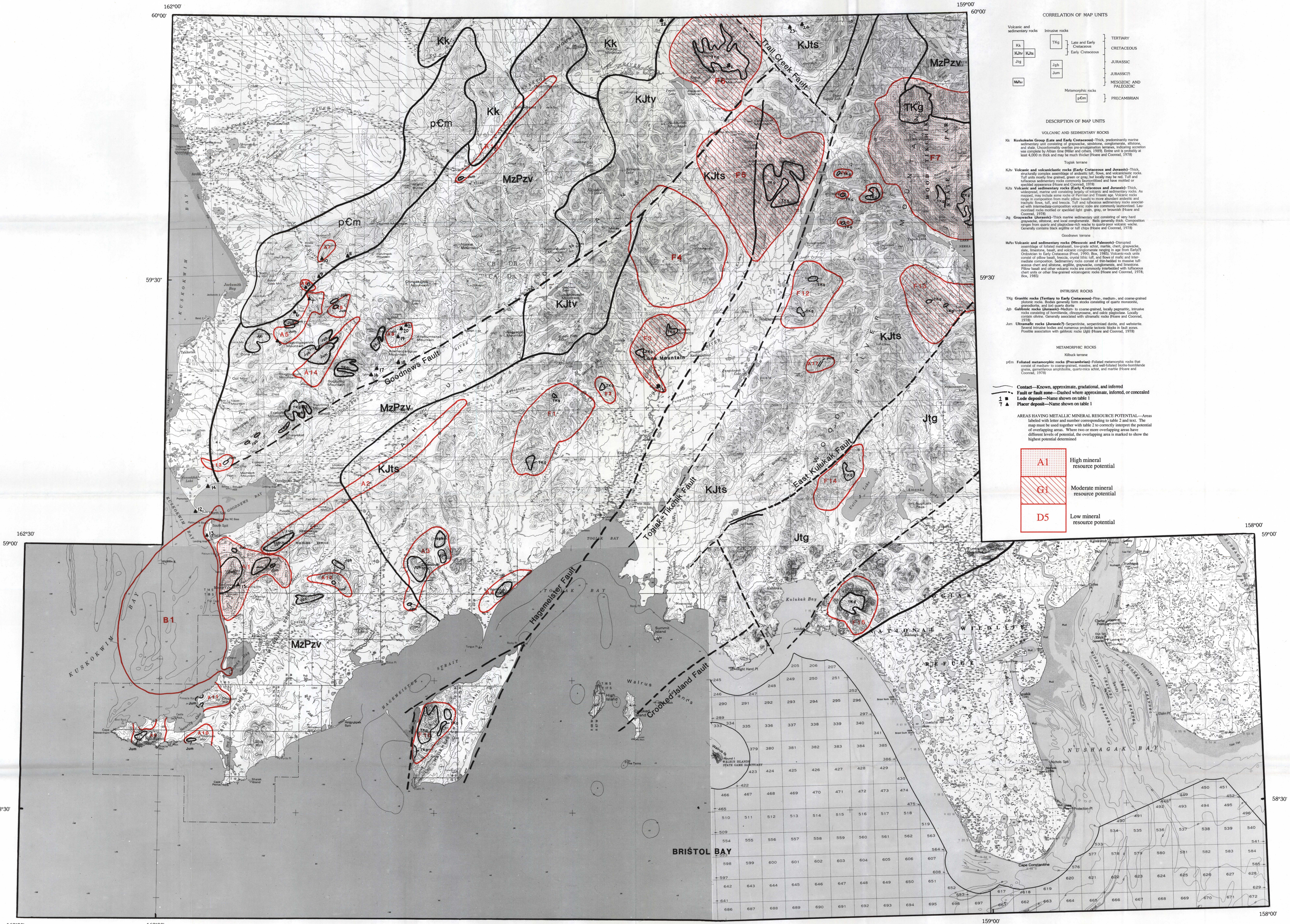
MAP A. Showing areas A1-A17, B1, and F1-F16 of metallic mineral resource potential
